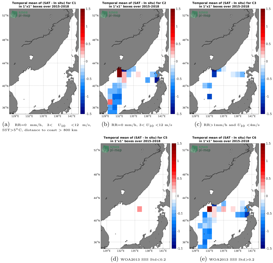
Figure 12: Temporal mean gridded over spatial boxes of size 1^\circ \times 1^\circ of \Delta\text{SSS} (SMAP-L3-JPL-V4.3-8DAY-RUNNING-60KM - TSG-LEGOS-DM) for 5 different subdatasets corresponding to: RR=0 mm/h, 3 < U_{10} < 12 m/s, SST > 5^\circ\text{C} , distance to coast > 800 km (a), RR=0 mm/h, 3 < U_{10} < 12 m/s (b), RR > 1\text{mm/h} and U_{10} < 4\text{m/s} (c), WOA2013 SSS Std < 0.2 (d), WOA2013 SSS Std > 0.2 (e).
