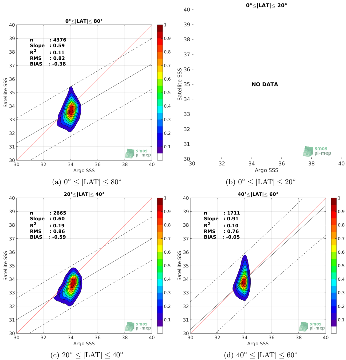
Figure 9: Contour maps of the concentration of SMAP-L3-JPL-V4.3-8DAY-RUNNING-60KM SSS (y-axis) versus Argo SSS (x-axis) at match-up pairs for different latitudinal bands. For each plot, the red line shows x=y . The black thin and dashed lines indicate a linear fit through the data cloud and the \pm 95\% confidence levels, respectively. The number match-up pairs n , the slope and R^2 coefficient of the linear fit, the root mean square (RMS) and the mean bias between satellite and in situ data are indicated for each latitude band in each plot.
