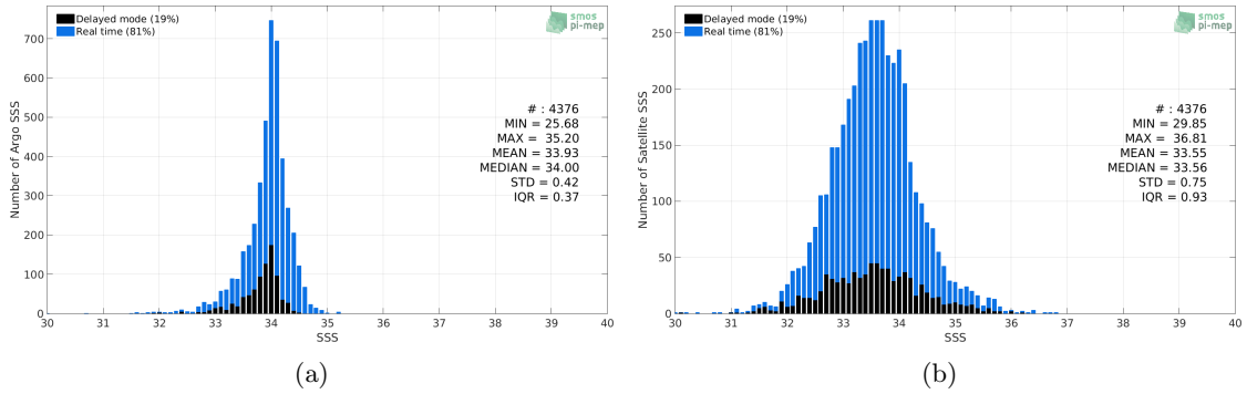
Figure 2: Histograms of SSS from Argo (a) and SMAP-L3-JPL-V4.3-8DAY-RUNNING-60KM (b) considering all match-up pairs per bins of 0.1 over the Sea of Japan Pi-MEP region and for the full satellite product period.
