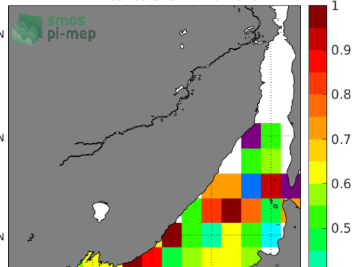
Temporal STD of (Sat - Argo) in 1°x1° boxes over 2015-2019
