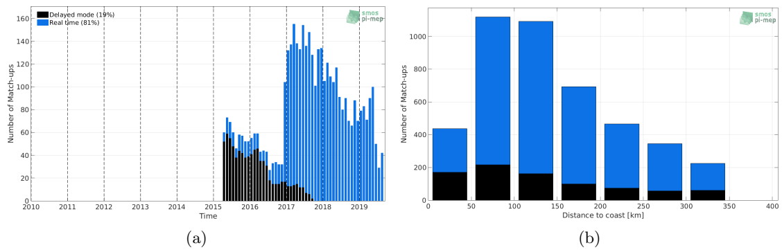
Figure 1: Number of match-ups between Argo and SMAP-L3-JPL-V4.3-8DAY-RUNNING-60KM SSS as a function of time (a) and as function of the distance to coast (b) over the Sea of Japan Pi-MEP region and for the full satellite product period.
