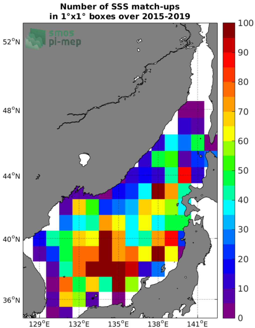
Figure 4: Number of SSS match-ups between Argo SSS and the SMAP-L3-JPL-V4.3-8DAY-RUNNING-60KM SSS product for the Sea of Japan Pi-MEP region over 1°x1° boxes and for the full satellite product period.
