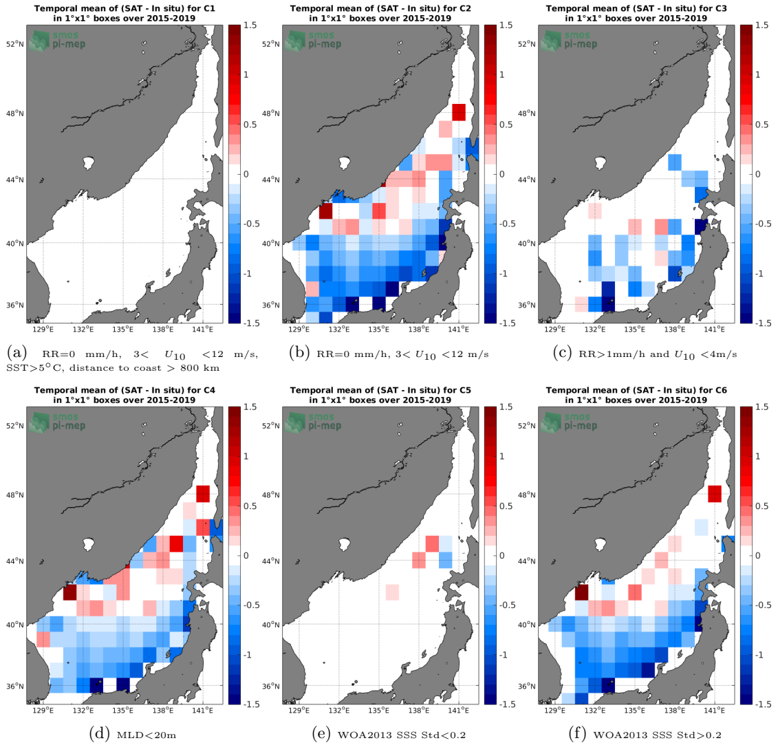
Figure 12: Temporal mean gridded over spatial boxes of size 1°x1° of \Delta\text{SSS} (SMAP-L3-JPL-V4.3-8DAY-RUNNING-60KM - Argo) for 6 different subdatasets corresponding to:RR=0 mm/h, 3 < U_{10} < 12 m/s, SST > 5^\circ\text{C} , distance to coast > 800 km (a), RR=0 mm/h, 3 < U_{10} < 12 m/s (b), RR > 1 mm/h and U_{10} < 4 m/s (c),MLD < 20 m (d),WOA2013 SSS Std < 0.2 (e),WOA2013 SSS Std > 0.2 (f).
