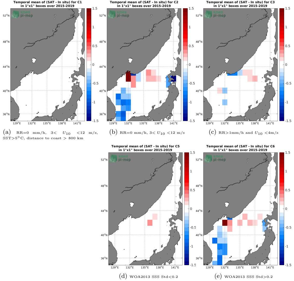
Figure 12: Temporal mean gridded over spatial boxes of size 1°x1° of \Delta\text{SSS} (SMAP-L3-JPL-V4.3-MONTHLY-60KM - TSG-LEGOS-DM) for 5 different subdatasets corresponding to: RR=0 mm/h, 3 < U_{10} < 12 m/s, SST > 5^\circ\text{C} , distance to coast > 800 km (a), RR=0 mm/h, 3 < U_{10} < 12 m/s (b), RR > 1 mm/h and U_{10} < 4 m/s (c), WOA2013 SSS Std < 0.2 (d), WOA2013 SSS Std > 0.2 (e).
