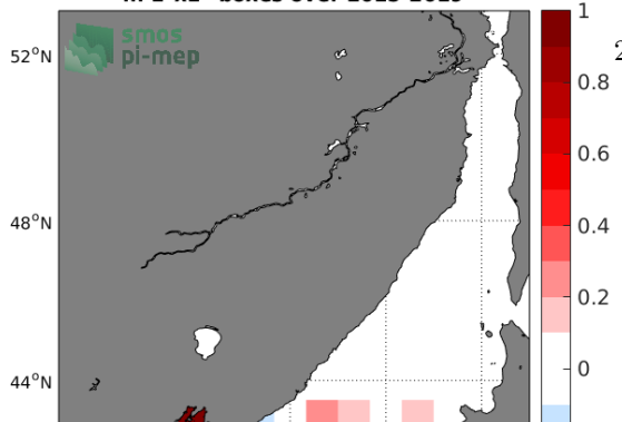
Temporal mean of (Sat - TSG-LEGOS-DM) in 1°x1° boxes over 2015-2019
