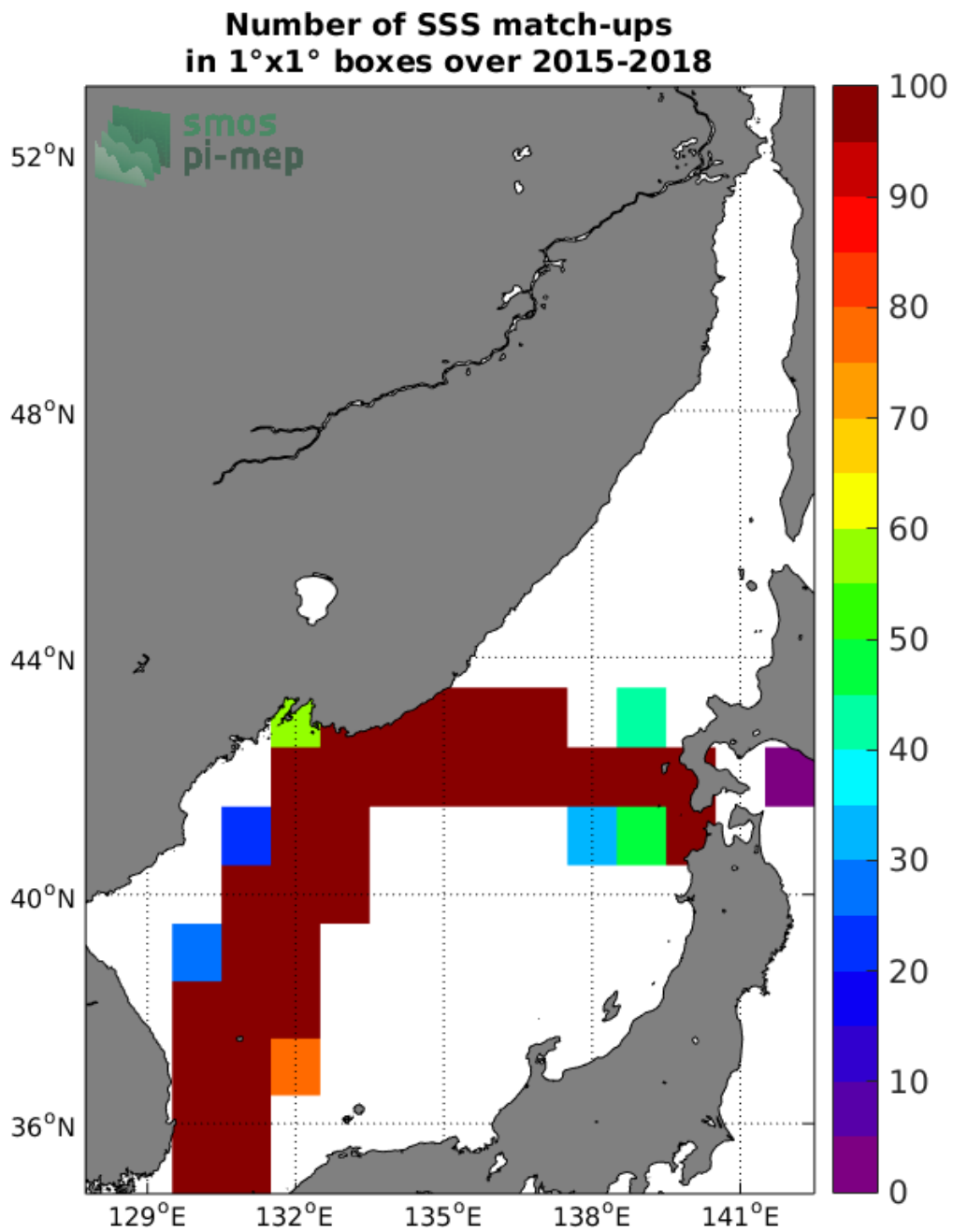
Figure 4: Number of SSS match-ups between TSG-LEGOS-DM SSS and the SMAP-L3-JPL-V4.3-MONTHLY-60KM SSS product for the Sea of Japan Pi-MEP region over 1°x1° boxes and for the full satellite product period.
