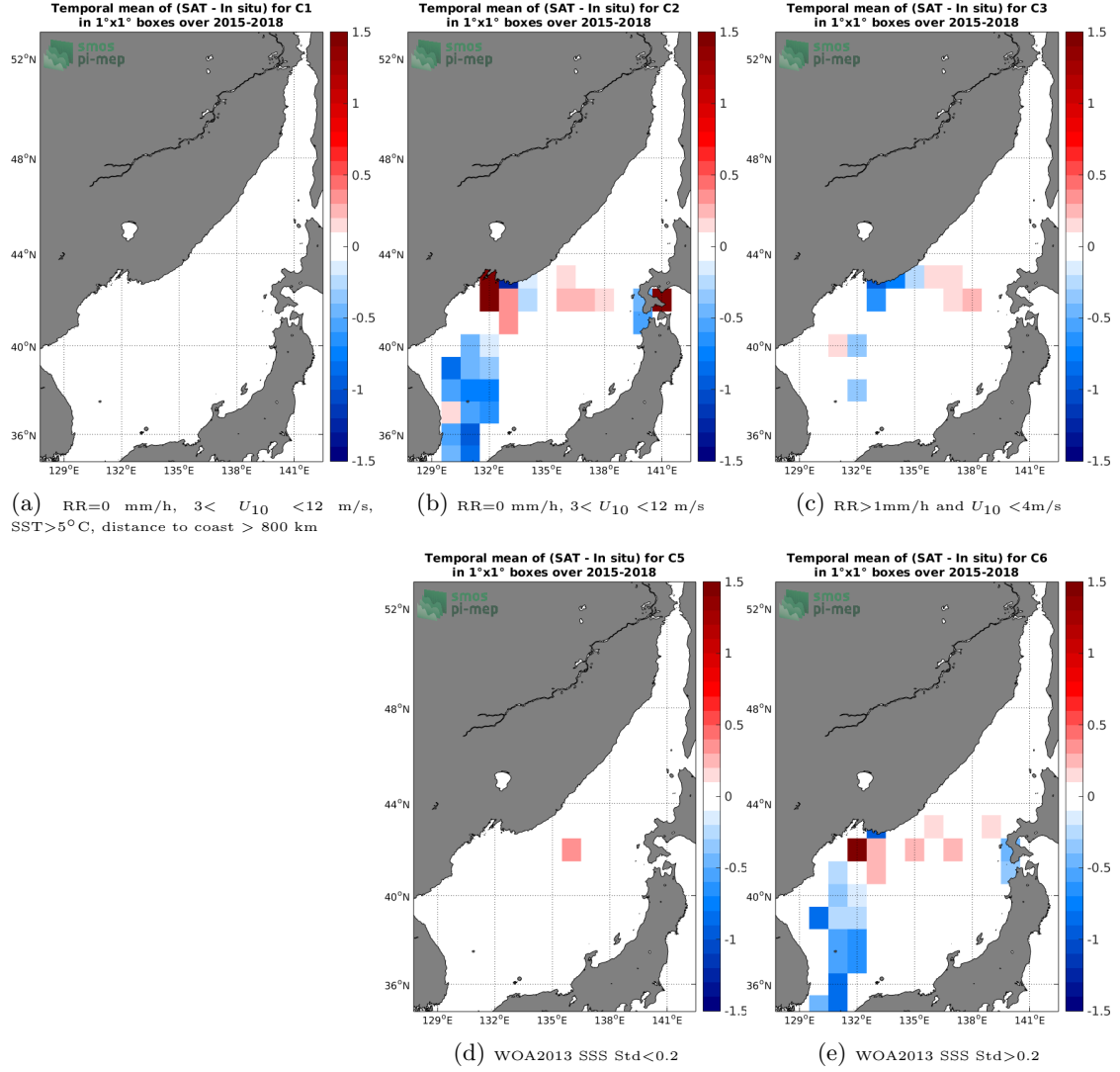
Figure 12: Temporal mean gridded over spatial boxes of size 1^\circ \times 1^\circ of \Delta SSS (SMAP-L3-JPL-V4.3-MONTHLY-60KM - TSG-LEGOS-DM) for 5 different subdatasets corresponding to:RR=0 mm/h, 3 < U_{10} < 12 m/s, SST>5°C, distance to coast > 800 km (a), RR=0 mm/h, 3 < U_{10} < 12 m/s (b), RR>1mm/h and U_{10} < 4 m/s (c), WOA2013 SSS Std<0.2 (d), WOA2013 SSS Std>0.2 (e).
