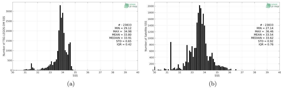
Figure 2: Histograms of SSS from TSG-LEGOS-DM (a) and SMAP-L3-JPL-V4.3-MONTHLY-60KM (b) considering all match-up pairs per bins of 0.1 over the Sea of Japan Pi-MEP region and for the full satellite product period.
