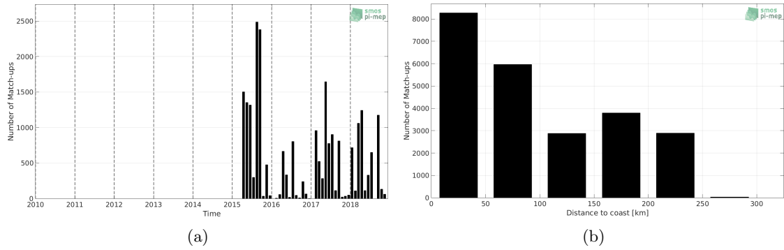
Figure 1: Number of match-ups between TSG-LEGOS-DM and SMAP-L3-JPL-V4.3-MONTHLY-60KM SSS as a function of time (a) and as function of the distance to coast (b) over the Sea of Japan Pi-MEP region and for the full satellite product period.
