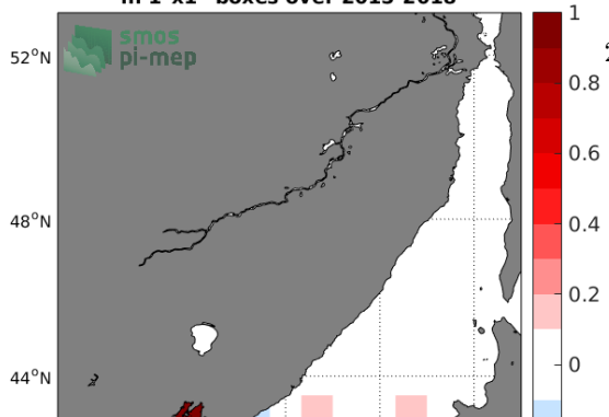
Temporal mean of (Sat - TSG-LEGOS-DM) in 1°x1° boxes over 2015-2018
