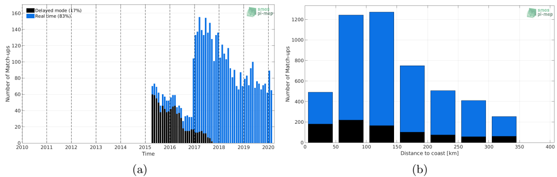
Figure 1: Number of match-ups between Argo and SMAP-L3-JPL-V4.3-MONTHLY-60KM SSS as a function of time (a) and as function of the distance to coast (b) over the Sea of Japan Pi-MEP region and for the full satellite product period.
