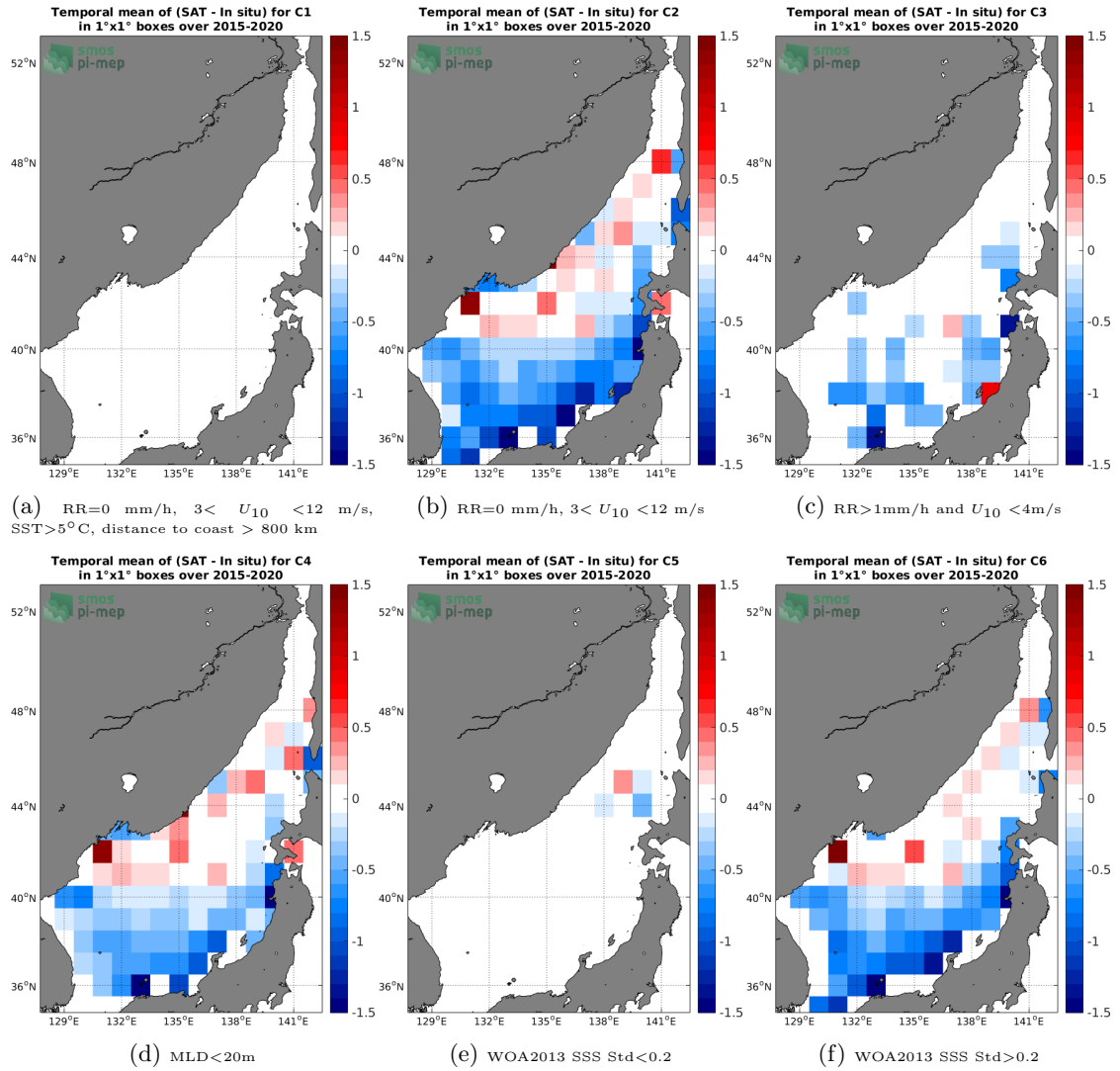
Figure 12: Temporal mean gridded over spatial boxes of size 1°x1° of \Delta\text{SSS} (SMAP-L3-JPL-V4.3-MONTHLY-60KM - Argo) for 6 different subdatasets corresponding to: RR=0 mm/h, 3 < U_{10} < 12 m/s, SST > 5^\circ\text{C} , distance to coast > 800 km (a), RR=0 mm/h, 3 < U_{10} < 12 m/s (b), RR > 1 mm/h and U_{10} < 4 m/s (c), MLD < 20 m (d), WOA2013 SSS Std < 0.2 (e), WOA2013 SSS Std > 0.2 (f).
