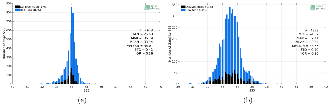
Figure 2: Histograms of SSS from Argo (a) and SMAP-L3-JPL-V4.3-MONTHLY-60KM (b) considering all match-up pairs per bins of 0.1 over the Sea of Japan Pi-MEP region and for the full satellite product period.
