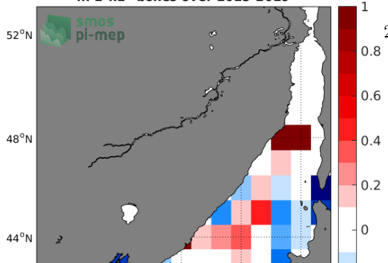
Temporal mean of (Sat - Argo) in 1°x1° boxes over 2015-2019
