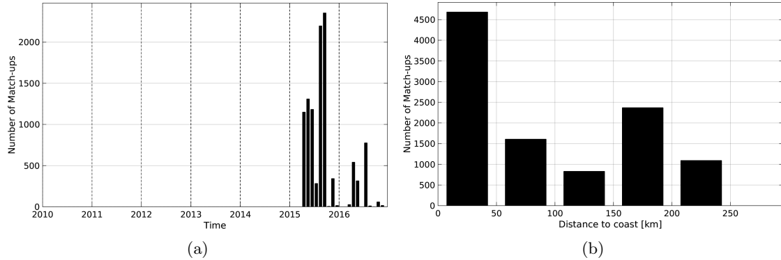
Figure 1: Number of match-ups between TSG-LEGOS-DM and SMAP-L3-JPL-V4-8DAY-RUNNING-60KM SSS as a function of time (a) and as function of the distance to coast (b) over the Sea of Japan Pi-MEP region and for the full satellite product period.
