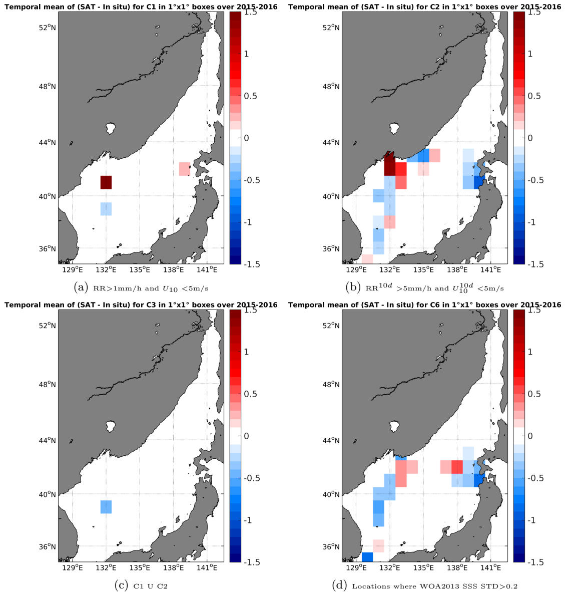
Figure 12: Temporal mean gridded over spatial boxes of size 1°x1° of \Delta SSS (SMAP-L3-JPL-V4-8DAY-RUNNING-60KM - TSG-LEGOS-DM) for 4 different subdatasets corresponding to: RR > 1\text{mm/h} and U_{10} < 5\text{m/s} (a), RR^{10d} > 5\text{mm/h} and U_{10}^{10d} < 5\text{m/s} (b), C1 U C2 (c), Locations where WOA2013 SSS STD > 0.2 (d).
