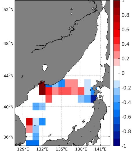
(e) MEAN( \Delta SSS) (Satellite - TSG-LEGOS-DM)
