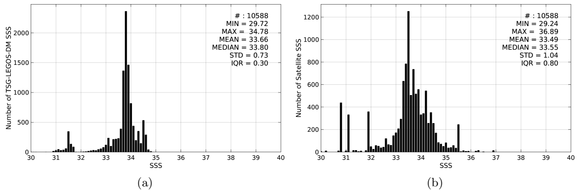
Figure 2: Histograms of SSS from TSG-LEGOS-DM (a) and SMAP-L3-JPL-V4-8DAY-RUNNING-60KM (b) considering all match-up pairs per bins of 0.1 over the Sea of Japan Pi-MEP region and for the full satellite product period.
