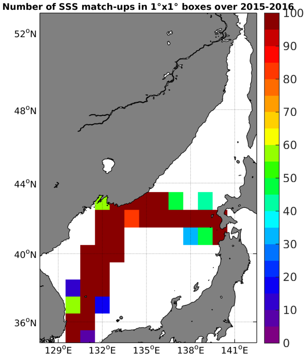
Figure 4: Number of SSS match-ups between TSG-LEGOS-DM SSS and the SMAP-L3-JPL-V4-8DAY-RUNNING-60KM SSS product for the Sea of Japan Pi-MEP region over 1°x1° boxes and for the full satellite product period.
