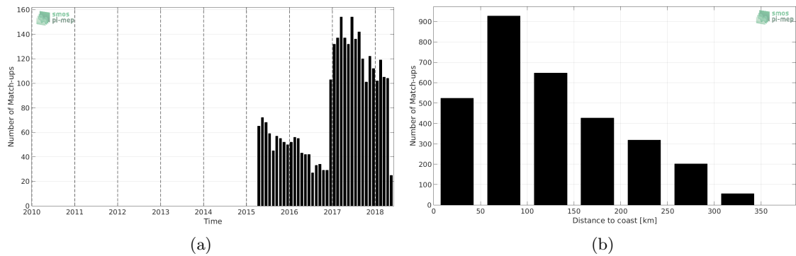
Figure 1: Number of match-ups between Argo and SMAP-L3-JPL-V4-8DAY-RUNNING-60KM SSS as a function of time (a) and as function of the distance to coast (b) over the Sea of Japan Pi-MEP region and for the full satellite product period.
