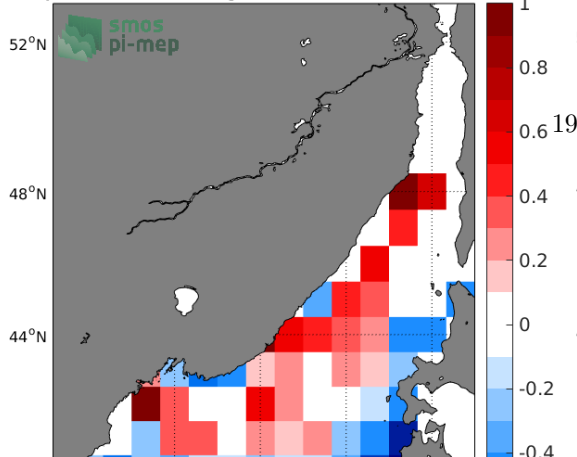
Temporal mean of (Sat-Argo) in 1°x1° boxes over 2015-2018
