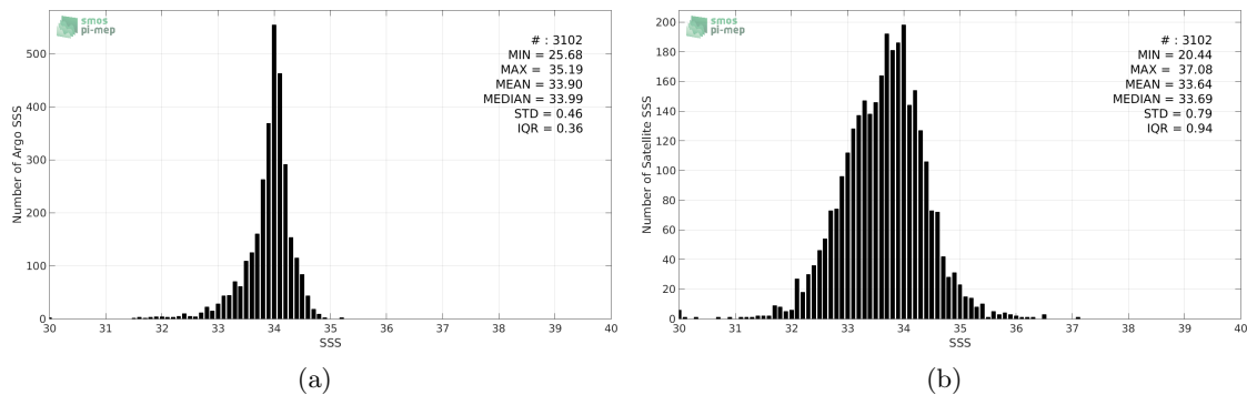
Figure 2: Histograms of SSS from Argo (a) and SMAP-L3-JPL-V4-8DAY-RUNNING-60KM (b) considering all match-up pairs per bins of 0.1 over the Sea of Japan Pi-MEP region and for the full satellite product period.
