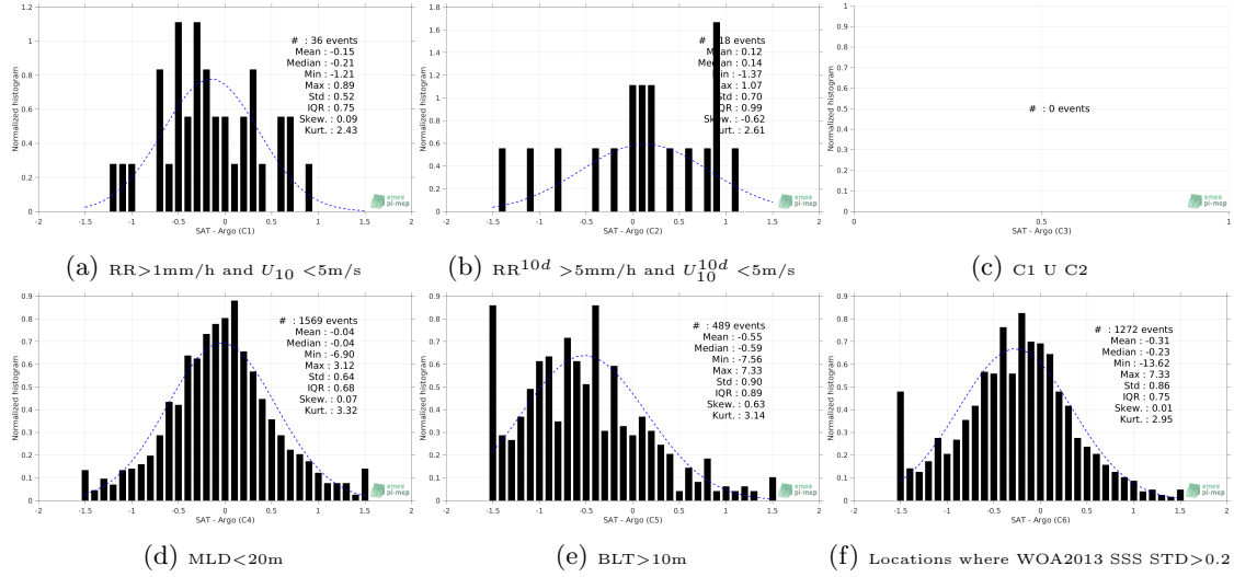
Figure 13: Normalized histogram of \Delta SSS (SMAP-L3-JPL-V4-8DAY-RUNNING-60KM - Argo) for 6 different subdatasets corresponding to: RR > 1\text{mm/h} and U_{10} < 5\text{m/s} (a), RR^{10d} > 5\text{mm/h} and U_{10}^{10d} < 5\text{m/s} (b), C1 U C2 (c), MLD < 20\text{m} (d), BLT > 10\text{m} (e), Locations where WOA2013 SSS STD > 0.2 (f).
