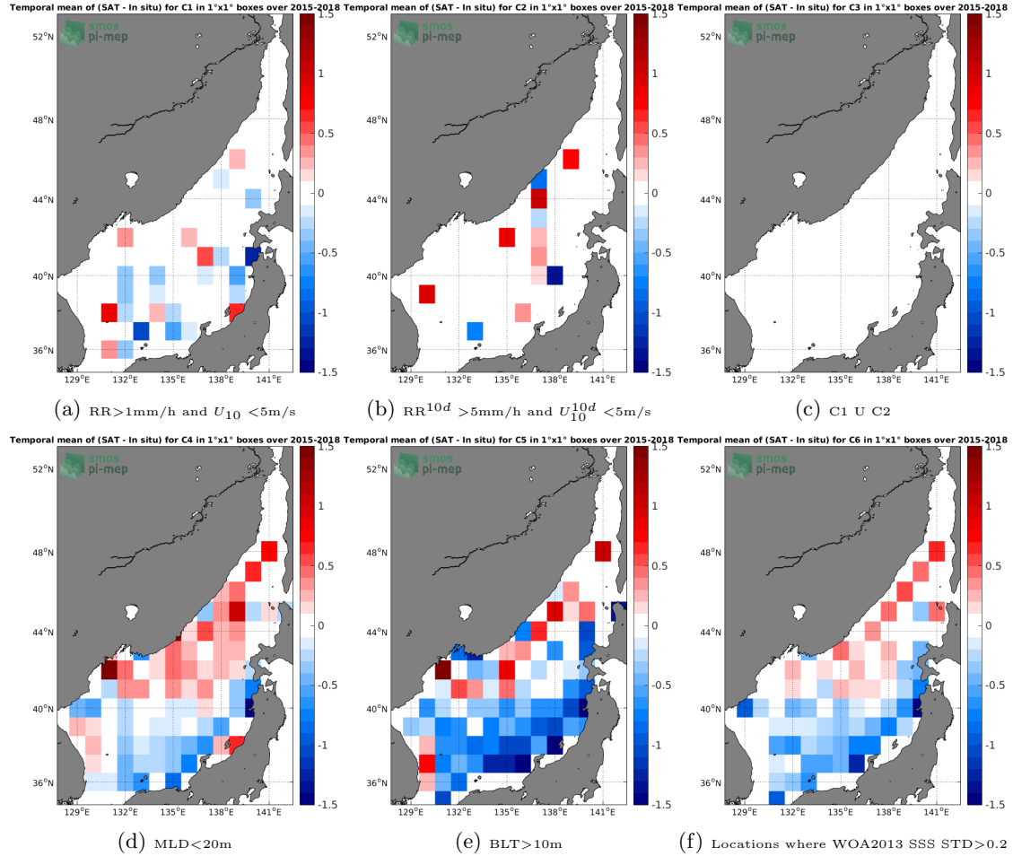
Figure 12: Temporal mean gridded over spatial boxes of size 1^\circ \times 1^\circ of \Delta SSS (SMAP-L3-JPL-V4-8DAY-RUNNING-60KM - Argo) for 6 different subdatasets corresponding to: RR > 1mm/h and U_{10} < 5\text{m/s} (a), RR^{10d} > 5\text{mm/h} and U_{10}^{10d} < 5\text{m/s} (b), C1 U C2 (c), MLD < 20m (d), BLT > 10m (e), Locations where WOA2013 SSS STD > 0.2 (f).
