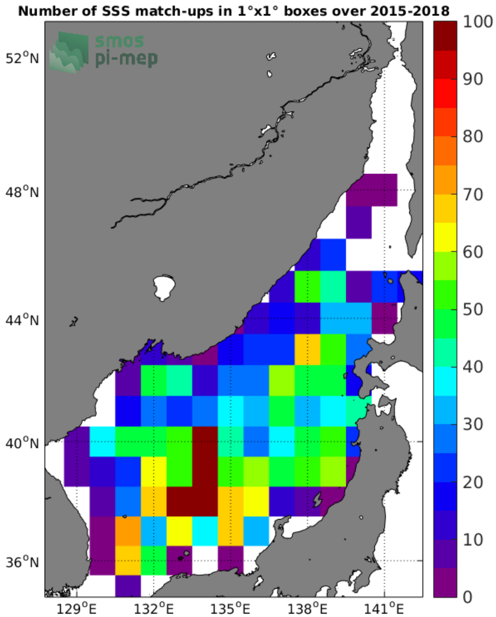
Figure 4: Number of SSS match-ups between Argo SSS and the SMAP-L3-JPL-V4-8DAY-RUNNING-60KM SSS product for the Sea of Japan Pi-MEP region over 1°x1° boxes and for the full satellite product period.
