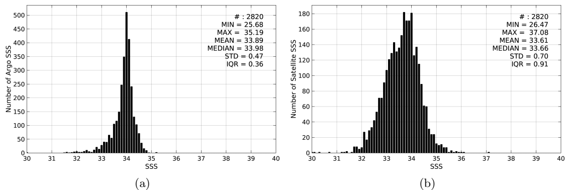
Figure 2: Histograms of SSS from Argo (a) and SMAP-L3-JPL-V4-8DAY-RUNNING-60KM (b) considering all match-up pairs per bins of 0.1 over the Sea of Japan Pi-MEP region and for the full satellite product period.
