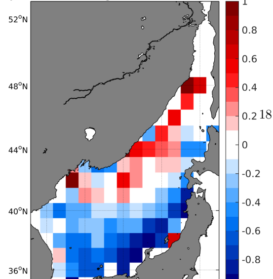
Temporal mean of (Sat-Argo) in 1°x1° boxes over 2015-2018
