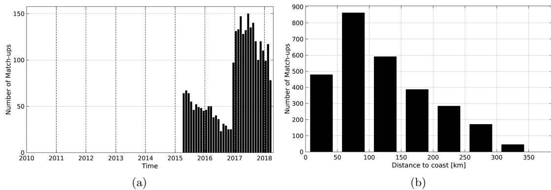
Figure 1: Number of match-ups between Argo and SMAP-L3-JPL-V4-8DAY-RUNNING-60KM SSS as a function of time (a) and as function of the distance to coast (b) over the Sea of Japan Pi-MEP region and for the full satellite product period.
