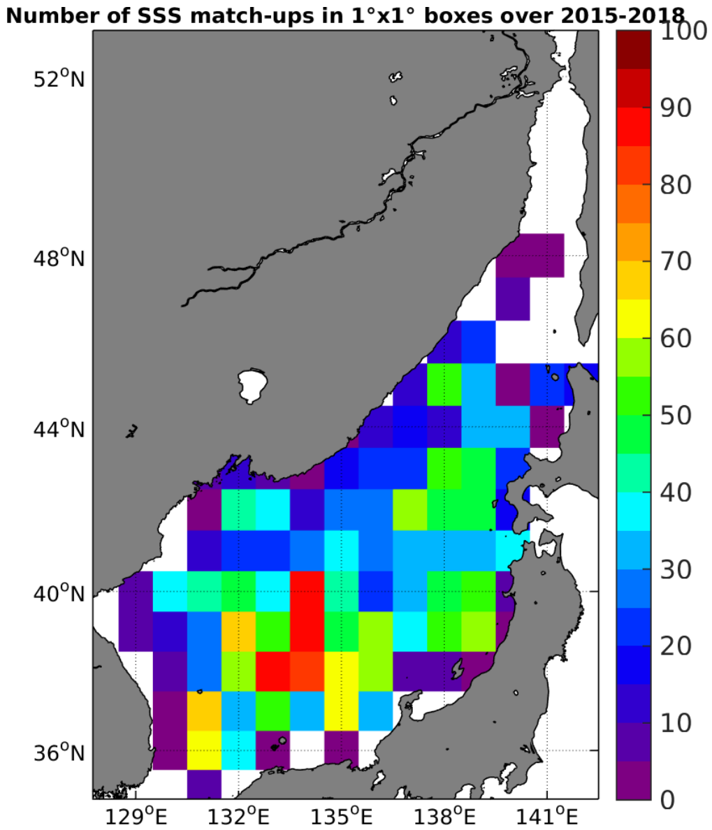
Figure 4: Number of SSS match-ups between Argo SSS and the SMAP-L3-JPL-V4-8DAY-RUNNING-60KM SSS product for the Sea of Japan Pi-MEP region over 1°x1° boxes and for the full satellite product period.
