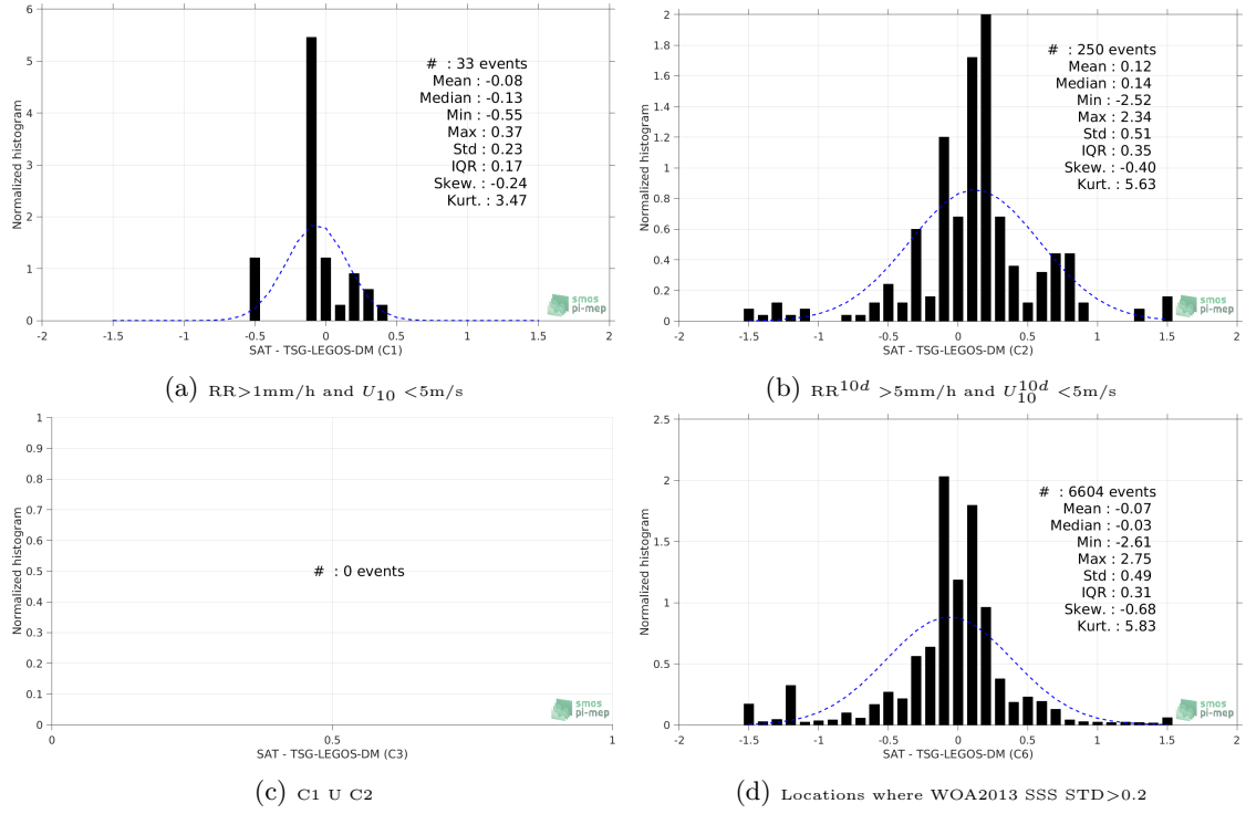
Figure 13: Normalized histogram of \Delta\text{SSS} (SMAP-L3-JPL-V4-MONTHLY-60KM - TSG-LEGOS-DM) for 6 different subdatasets corresponding to: RR > 1mm/h and U_{10} < 5\text{m/s} (a), RR^{10d} > 5\text{mm/h} and U_{10}^{10d} < 5\text{m/s} (b), C1 U C2 (c), Locations where WOA2013 SSS STD > 0.2 (d).
