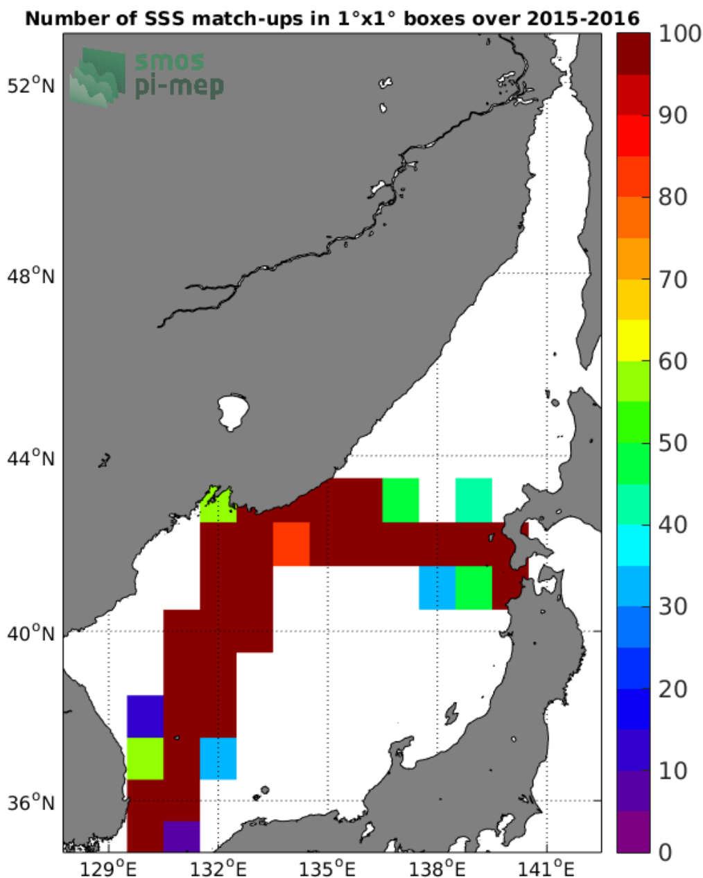
Figure 4: Number of SSS match-ups between TSG-LEGOS-DM SSS and the SMAP-L3-JPL-V4-MONTHLY-60KM SSS product for the Sea of Japan Pi-MEP region over 1°x1° boxes and for the full satellite product period.
