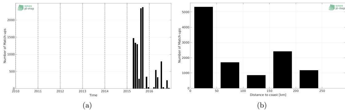
Figure 1: Number of match-ups between TSG-LEGOS-DM and SMAP-L3-JPL-V4-MONTHLY-60KM SSS as a function of time (a) and as function of the distance to coast (b) over the Sea of Japan Pi-MEP region and for the full satellite product period.
