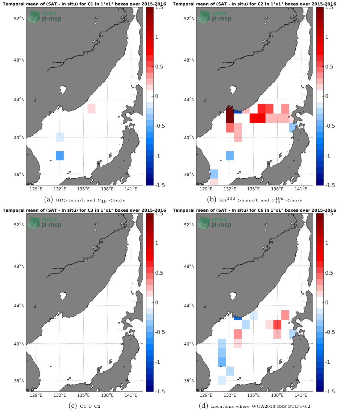
Figure 12: Temporal mean gridded over spatial boxes of size 1°x1° of \Delta\text{SSS} (SMAP-L3-JPL-V4-MONTHLY-60KM - TSG-LEGOS-DM) for 4 different subdatasets corresponding to: RR > 1\text{mm/h} and U_{10} < 5\text{m/s} (a), RR^{10d} > 5\text{mm/h} and U_{10}^{10d} < 5\text{m/s} (b), C1 U C2 (c), Locations where WOA2013 SSS STD > 0.2 (d).
