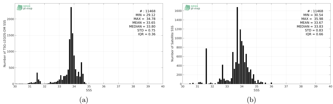
Figure 2: Histograms of SSS from TSG-LEGOS-DM (a) and SMAP-L3-JPL-V4-MONTHLY-60KM (b) considering all match-up pairs per bins of 0.1 over the Sea of Japan Pi-MEP region and for the full satellite product period.
