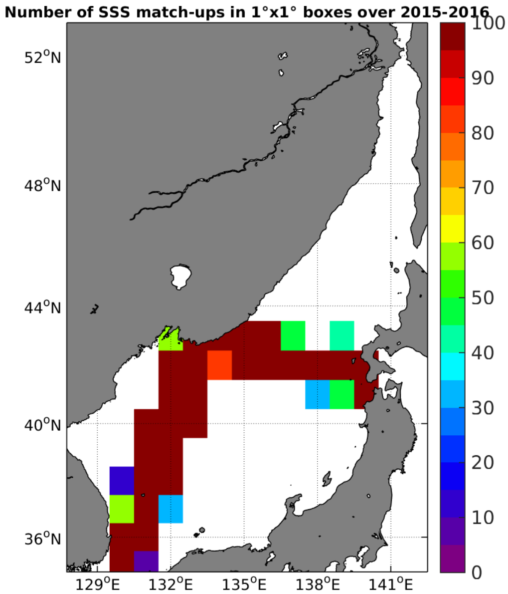
Figure 4: Number of SSS match-ups between TSG-LEGOS-DM SSS and the SMAP-L3-JPL-V4-MONTHLY-60KM SSS product for the Sea of Japan Pi-MEP region over 1°x1° boxes and for the full satellite product period.
