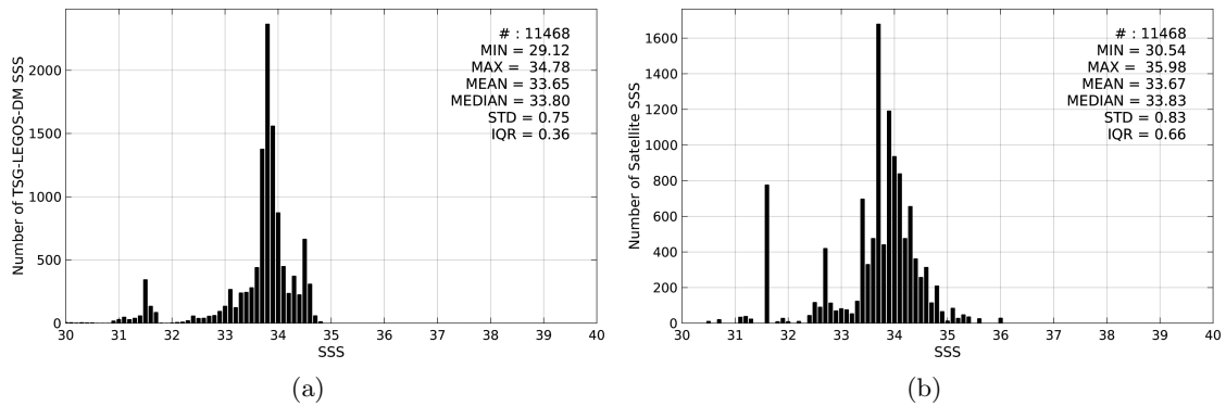
Figure 2: Histograms of SSS from TSG-LEGOS-DM (a) and SMAP-L3-JPL-V4-MONTHLY-60KM (b) considering all match-up pairs per bins of 0.1 over the Sea of Japan Pi-MEP region and for the full satellite product period.
