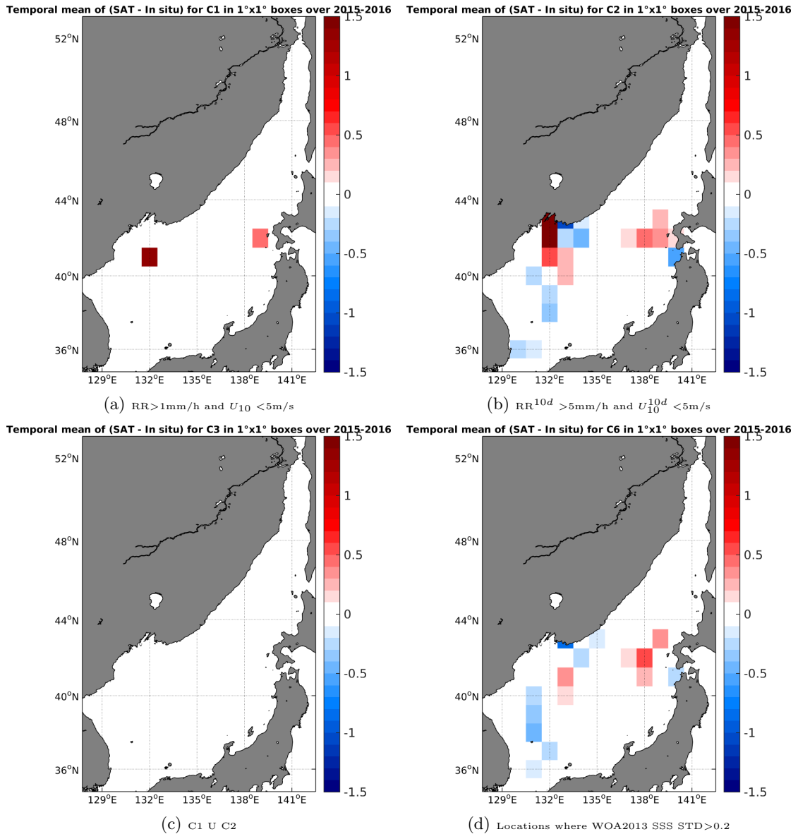
Figure 12: Temporal mean gridded over spatial boxes of size 1°x1° of \Delta SSS (SMAP-L3-JPL-V4-MONTHLY-60KM - TSG-LEGOS-DM) for 4 different subdatasets corresponding to: RR > 1\text{mm/h} and U_{10} < 5\text{m/s} (a), RR^{10d} > 5\text{mm/h} and U_{10}^{10d} < 5\text{m/s} (b), C1 U C2 (c), Locations where WOA2013 SSS STD > 0.2 (d).
