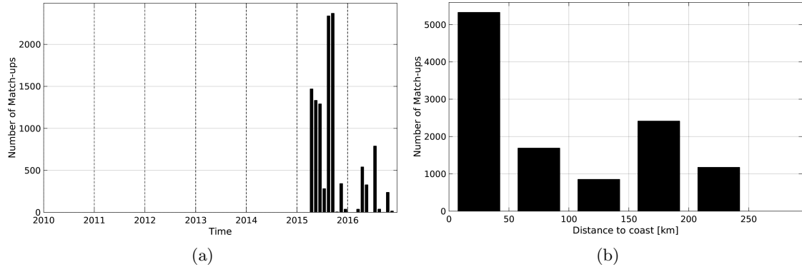
Figure 1: Number of match-ups between TSG-LEGOS-DM and SMAP-L3-JPL-V4-MONTHLY-60KM SSS as a function of time (a) and as function of the distance to coast (b) over the Sea of Japan Pi-MEP region and for the full satellite product period.
