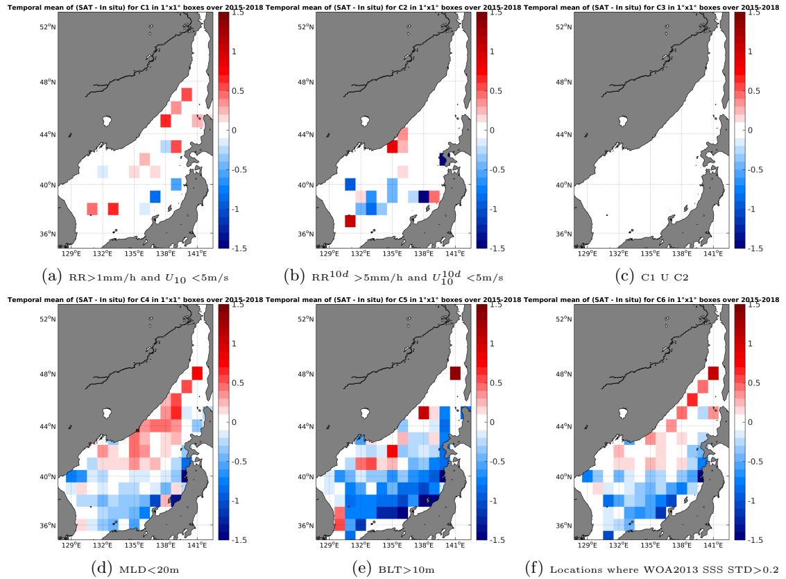
Figure 12: Temporal mean gridded over spatial boxes of size 1°x1° of \Delta SSS (SMAP-L3-JPL-V4-MONTHLY-60KM - Argo) for 6 different subdatasets corresponding to: RR > 1\text{mm/h} and U_{10} < 5\text{m/s} (a), RR^{10d} > 5\text{mm/h} and U_{10}^{10d} < 5\text{m/s} (b), C1 U C2 (c), MLD < 20\text{m} (d), BLT > 10\text{m} (e), Locations where WOA2013 SSS STD > 0.2 (f).
