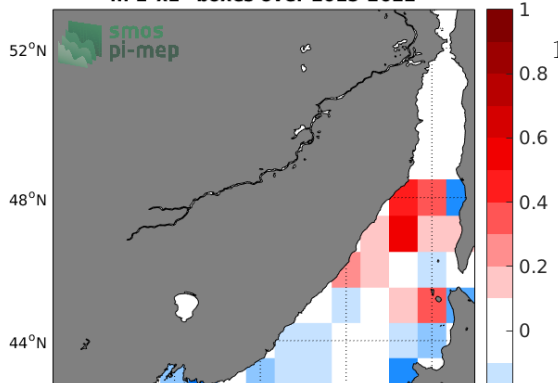
Temporal mean of (Sat - Argo) in 1°x1° boxes over 2015-2022
