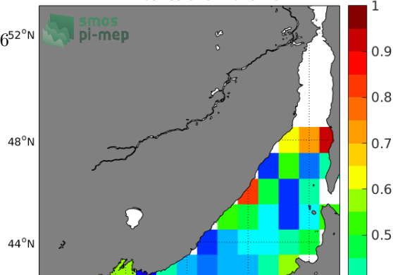
Temporal STD of (Sat - Argo) in 1°x1° boxes over 2015-2022
