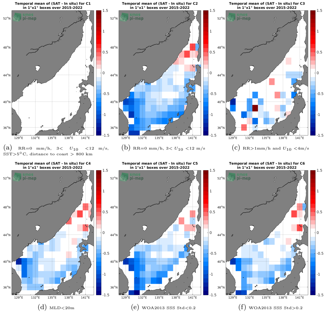
Figure 12: Temporal mean gridded over spatial boxes of size 1^\circ \times 1^\circ of \Delta SSS (SMAP SSS L2-AVERAGED v5 (RSS) - Argo) for 6 different subdatasets corresponding to: RR=0 mm/h, 3 < U_{10} < 12 m/s, SST > 5°C, distance to coast > 800 km (a), RR=0 mm/h, 3 < U_{10} < 12 m/s (b), RR > 1mm/h and U_{10} < 4 m/s (c), MLD < 20m (d), WOA2013 SSS Std < 0.2 (e), WOA2013 SSS Std > 0.2 (f).
