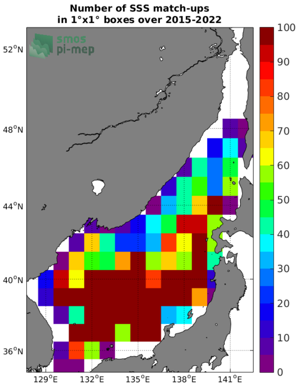
Figure 4: Number of SSS match-ups between Argo SSS and the SMAP SSS L2-AVERAGED v5 (RSS) SSS product for the Sea of Japan Pi-MEP region over 1°×1° boxes and for the full satellite product period.
