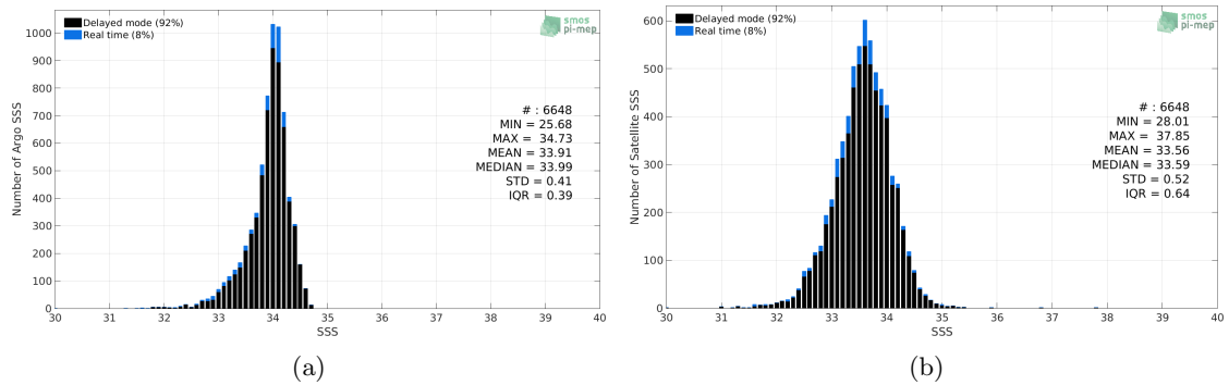
Figure 2: Histograms of SSS from Argo (a) and SMAP SSS L2-AVERAGED v5 (RSS) (b) considering all match-up pairs per bins of 0.1 over the Sea of Japan Pi-MEP region and for the full satellite product period.
