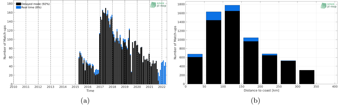
Figure 1: Number of match-ups between Argo and SMAP SSS L2-AVERAGED v5 (RSS) SSS as a function of time (a) and as function of the distance to coast (b) over the Sea of Japan Pi-MEP region and for the full satellite product period.
