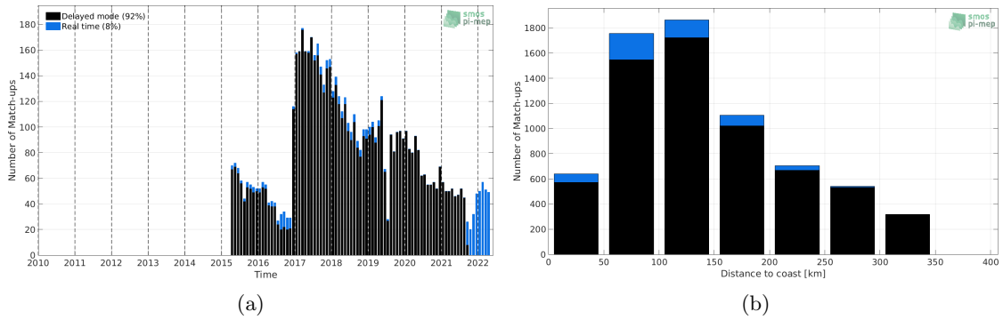
Figure 1: Number of match-ups between Argo and SMAP SSS L2-AVERAGED v5.0 (JPL) SSS as a function of time (a) and as function of the distance to coast (b) over the Sea of Japan Pi-MEP region and for the full satellite product period.
