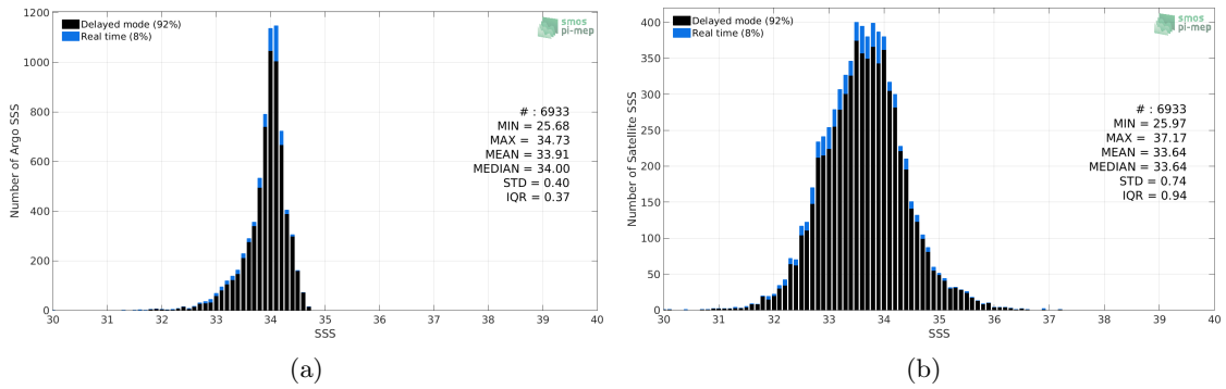
Figure 2: Histograms of SSS from Argo (a) and SMAP SSS L2-AVERAGED v5.0 (JPL) (b) considering all match-up pairs per bins of 0.1 over the Sea of Japan Pi-MEP region and for the full satellite product period.
