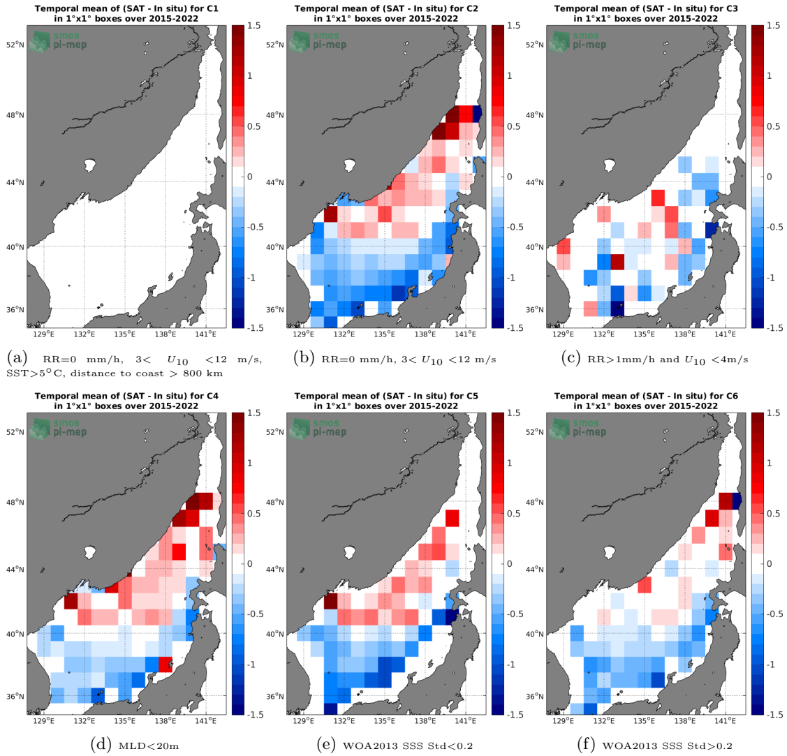
Figure 12: Temporal mean gridded over spatial boxes of size 1^\circ \times 1^\circ of \Delta SSS (SMAP SSS L2-AVERAGED v5.0 (JPL) - Argo) for 6 different subdatasets corresponding to: RR=0 mm/h, 3 < U_{10} < 12 m/s, SST > 5^\circ\text{C} , distance to coast > 800 km (a), RR=0 mm/h, 3 < U_{10} < 12 m/s (b), RR > 1 mm/h and U_{10} < 4 m/s (c), MLD < 20 m (d), WOA2013 SSS Std < 0.2 (e), WOA2013 SSS Std > 0.2 (f).
