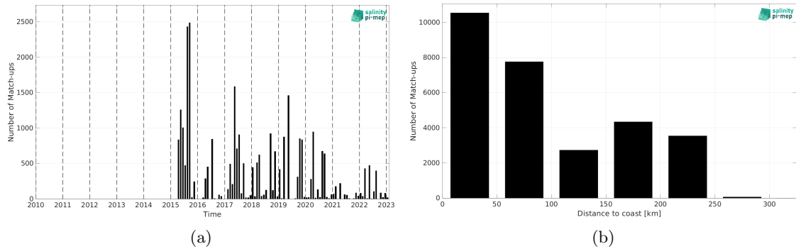
Figure 2: Number of match-ups between TSG (LEGOS-DM) and SMAP SSS L2 v6 (RSS) SSS as a function of time (a) and as function of the distance to coast (b) over the Sea of Japan Pi-MEP region and for the full satellite product period.
