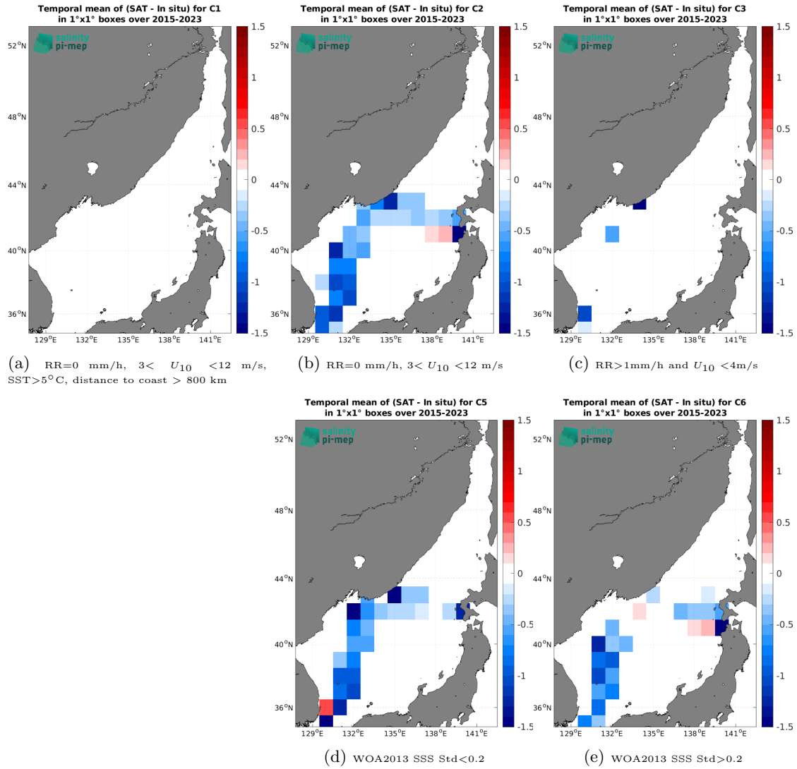
Figure 14: Temporal mean gridded over spatial boxes of size 1^\circ \times 1^\circ of \Delta\text{SSS} (SMAP SSS L2 v6 (RSS) - TSG (LEGOS-DM)) for 5 different subdatasets corresponding to: RR=0 mm/h, 3 < U_{10} < 12 m/s, SST > 5^\circ\text{C} , distance to coast > 800 km (a), RR=0 mm/h, 3 < U_{10} < 12 m/s (b), RR > 1 mm/h and U_{10} < 4 m/s (c), WOA2013 SSS Std < 0.2 (d), WOA2013 SSS Std > 0.2 (e).
