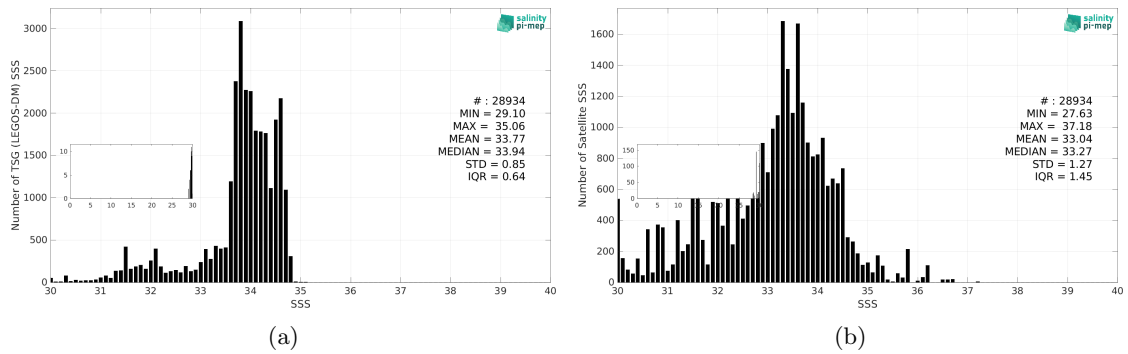
Figure 3: Histograms of SSS from TSG (LEGOS-DM) (a) and SMAP SSS L2 v6 (RSS) (b) considering all match-up pairs per bins of 0.1 over the Sea of Japan Pi-MEP region and for the full satellite product period.
