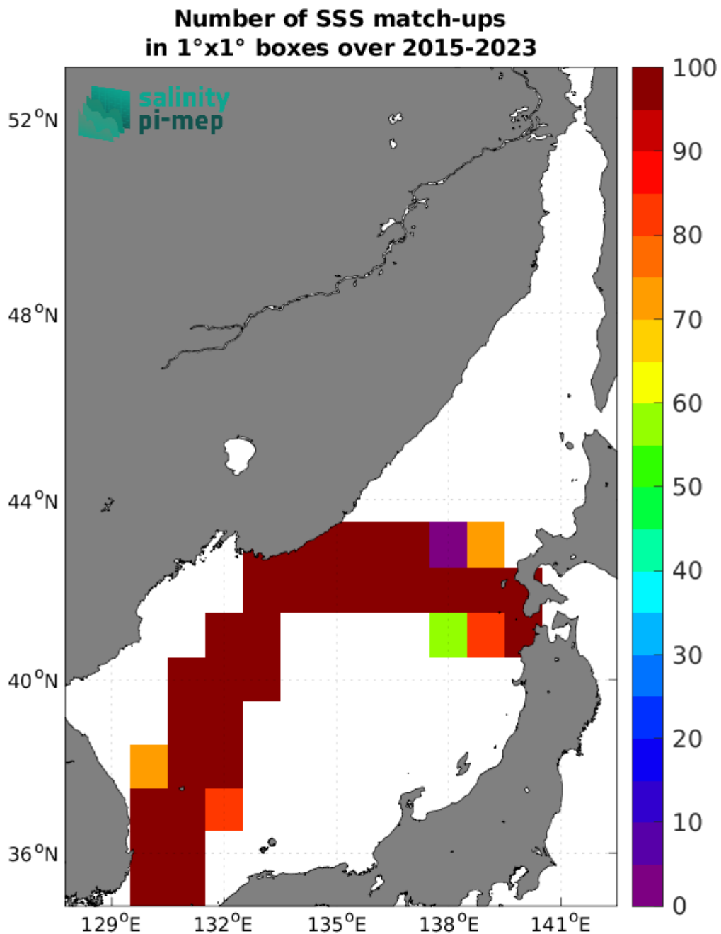
Figure 5: Number of SSS match-ups between TSG (LEGOS-DM) SSS and the SMAP SSS L2 v6 (RSS) SSS product for the Sea of Japan Pi-MEP region over 1°x1° boxes and for the full satellite product period.
