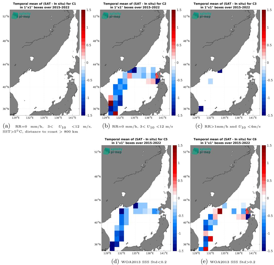
Figure 14: Temporal mean gridded over spatial boxes of size 1^\circ \times 1^\circ of \Delta\text{SSS} (SMAP SSS L2 v6 - 40 km (RSS) - TSG (LEGOS-DM)) for 5 different subdatasets corresponding to: RR=0 mm/h, 3 < U_{10} < 12 m/s, SST > 5^\circ\text{C} , distance to coast > 800 km (a), RR=0 mm/h, 3 < U_{10} < 12 m/s (b), RR > 1 mm/h and U_{10} < 4 m/s (c), WOA2013 SSS Std < 0.2 (d), WOA2013 SSS Std > 0.2 (e).
