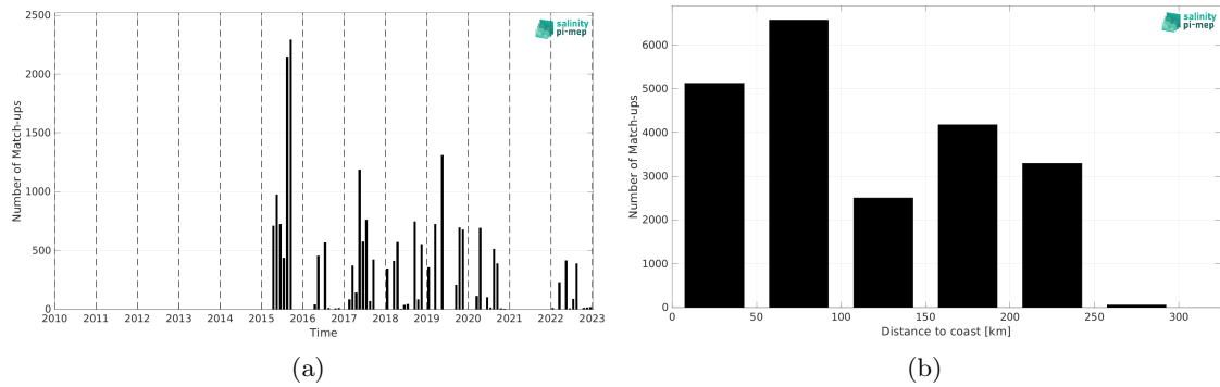
Figure 2: Number of match-ups between TSG (LEGOS-DM) and SMAP SSS L2 v6 - 40 km (RSS) SSS as a function of time (a) and as function of the distance to coast (b) over the Sea of Japan Pi-MEP region and for the full satellite product period.
