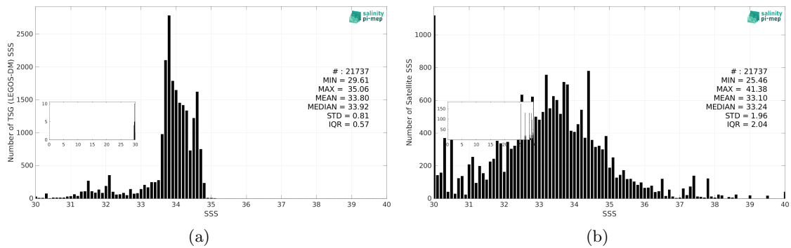
Figure 3: Histograms of SSS from TSG (LEGOS-DM) (a) and SMAP SSS L2 v6 - 40 km (RSS) (b) considering all match-up pairs per bins of 0.1 over the Sea of Japan Pi-MEP region and for the full satellite product period.
