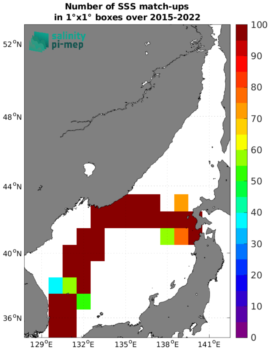
Figure 5: Number of SSS match-ups between TSG (LEGOS-DM) SSS and the SMAP SSS L2 v6 - 40 km (RSS) SSS product for the Sea of Japan Pi-MEP region over 1°x1° boxes and for the full satellite product period.
