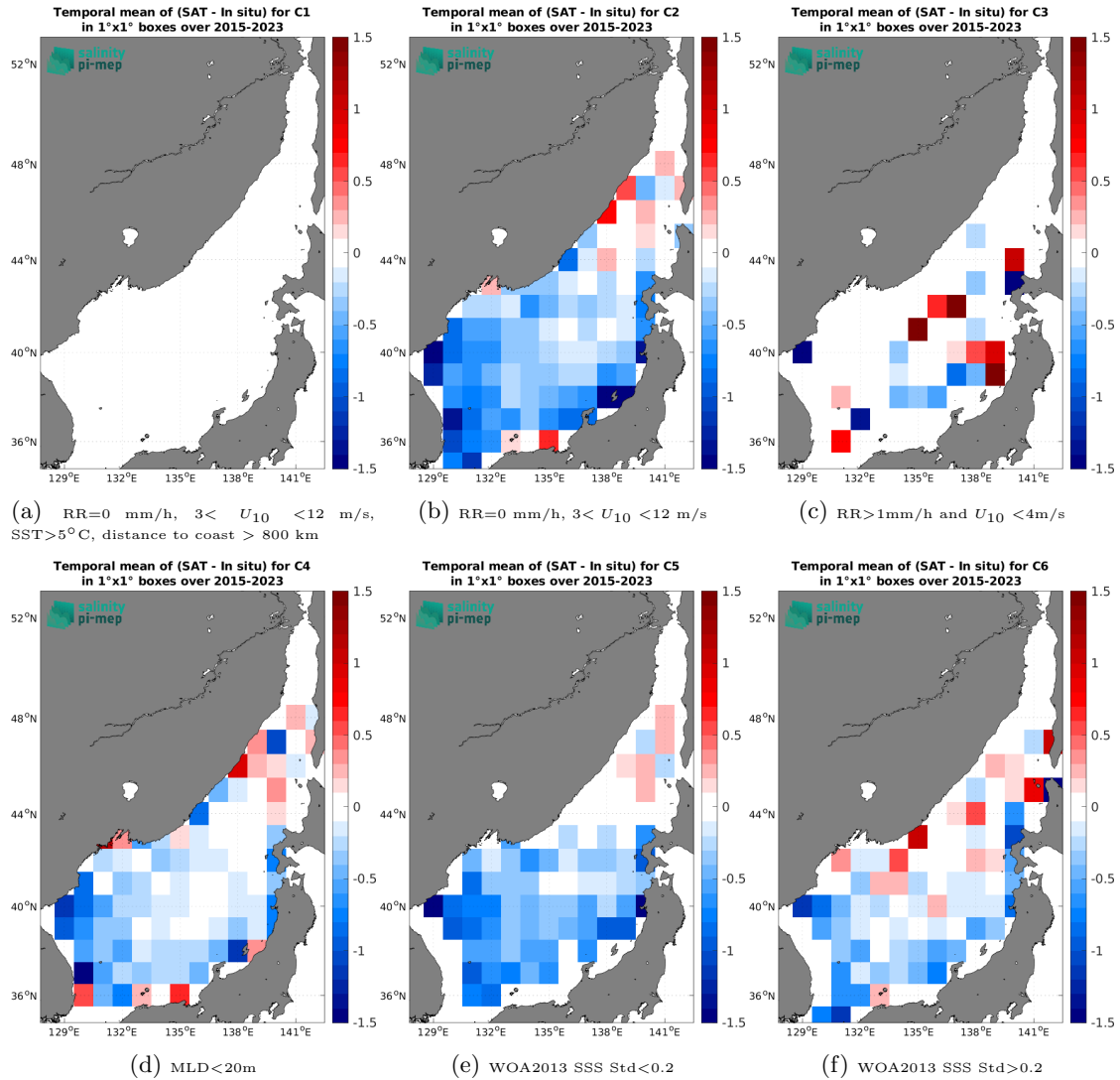
Figure 12: Temporal mean gridded over spatial boxes of size 1^\circ \times 1^\circ of \Delta SSS (SMAP SSS L2 v5 (RSS) - Argo) for 6 different subdatasets corresponding to: RR=0 mm/h, 3 < U_{10} < 12 m/s, SST > 5°C, distance to coast > 800 km (a), RR=0 mm/h, 3 < U_{10} < 12 m/s (b), RR > 1mm/h and U_{10} < 4 m/s (c), MLD < 20m (d), WOA2013 SSS Std < 0.2 (e), WOA2013 SSS Std > 0.2 (f).
