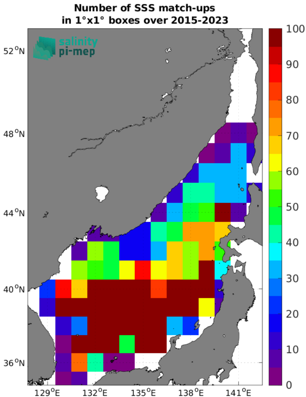
Figure 4: Number of SSS match-ups between Argo SSS and the SMAP SSS L2 v5 (RSS) SSS product for the Sea of Japan Pi-MEP region over 1°x1° boxes and for the full satellite product period.
