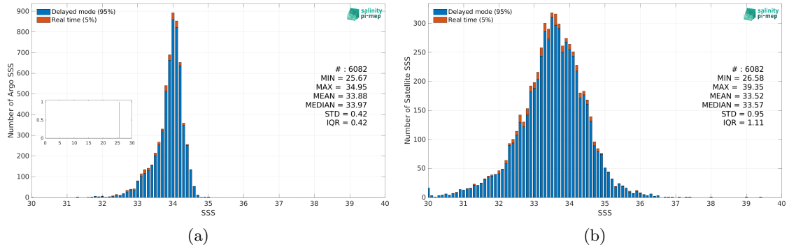
Figure 2: Histograms of SSS from Argo (a) and SMAP SSS L2 v5 (RSS) (b) considering all match-up pairs per bins of 0.1 over the Sea of Japan Pi-MEP region and for the full satellite product period.
