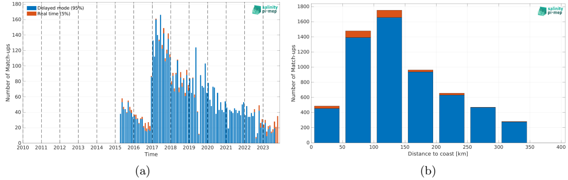
Figure 1: Number of match-ups between Argo and SMAP SSS L2 v5 (RSS) SSS as a function of time (a) and as function of the distance to coast (b) over the Sea of Japan Pi-MEP region and for the full satellite product period.
