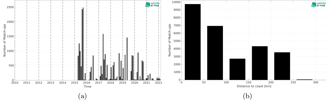
Figure 2: Number of match-ups between TSG (LEGOS-DM) and SMAP SSS L2 v5.3 (RSS) SSS as a function of time (a) and as function of the distance to coast (b) over the Sea of Japan Pi-MEP region and for the full satellite product period.
