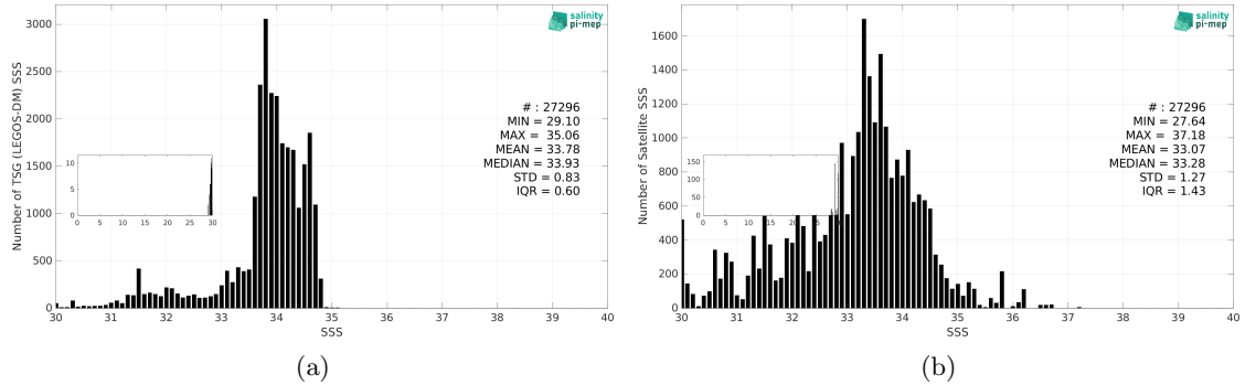
Figure 3: Histograms of SSS from TSG (LEGOS-DM) (a) and SMAP SSS L2 v5.3 (RSS) (b) considering all match-up pairs per bins of 0.1 over the Sea of Japan Pi-MEP region and for the full satellite product period.
