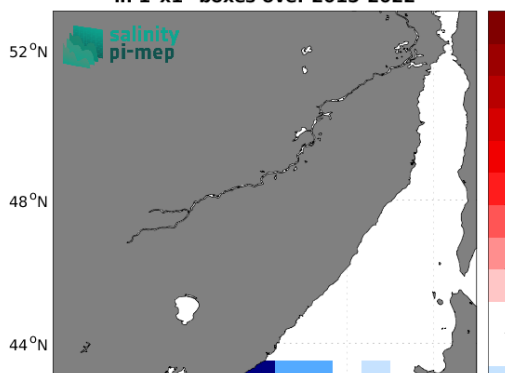
Temporal mean of (Sat - TSG (LEGOS-DM)) in 1°x1° boxes over 2015-2022
