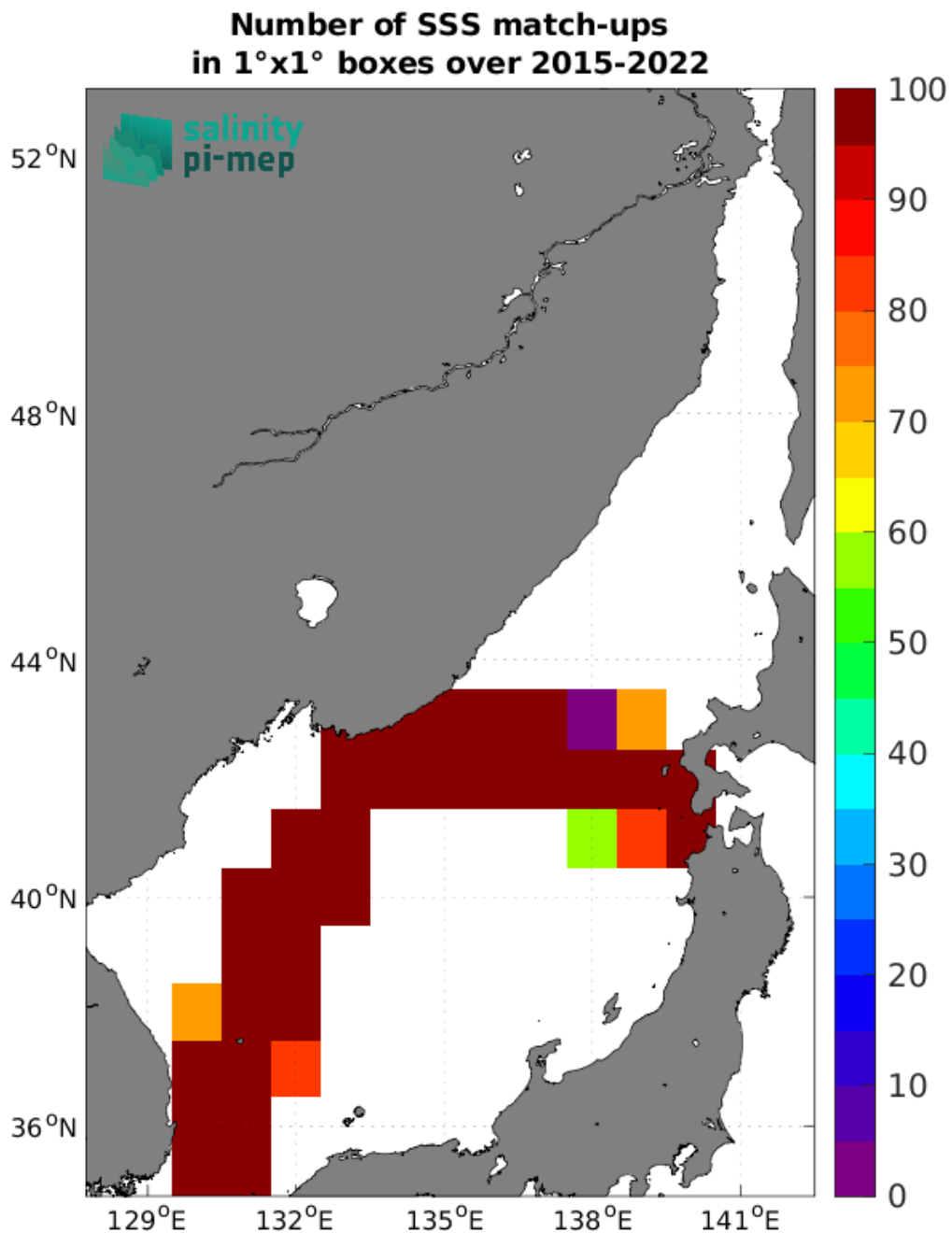
Figure 5: Number of SSS match-ups between TSG (LEGOS-DM) SSS and the SMAP SSS L2 v5.3 (RSS) SSS product for the Sea of Japan Pi-MEP region over 1°×1° boxes and for the full satellite product period.
