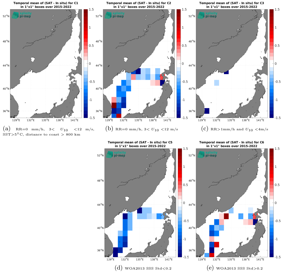
Figure 14: Temporal mean gridded over spatial boxes of size 1^\circ \times 1^\circ of \Delta SSS (SMAP SSS L2 v5.3 - 40 km (RSS) - TSG (LEGOS-DM)) for 5 different subdatasets corresponding to:RR=0 mm/h, 3 < U_{10} < 12 m/s, SST>5°C, distance to coast > 800 km (a), RR=0 mm/h, 3 < U_{10} < 12 m/s (b), RR>1mm/h and U_{10} < 4 m/s (c), WOA2013 SSS Std<0.2 (d), WOA2013 SSS Std>0.2 (e).
