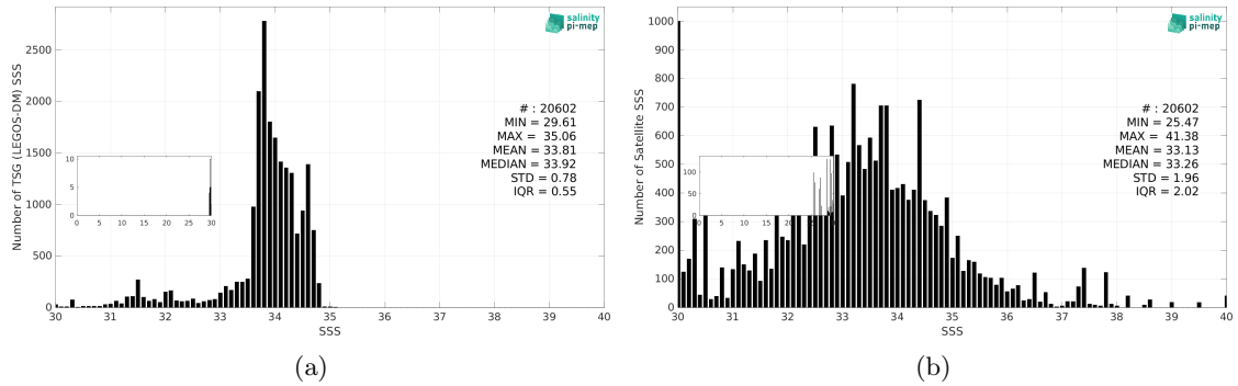
Figure 3: Histograms of SSS from TSG (LEGOS-DM) (a) and SMAP SSS L2 v5.3 - 40 km (RSS) (b) considering all match-up pairs per bins of 0.1 over the Sea of Japan Pi-MEP region and for the full satellite product period.
