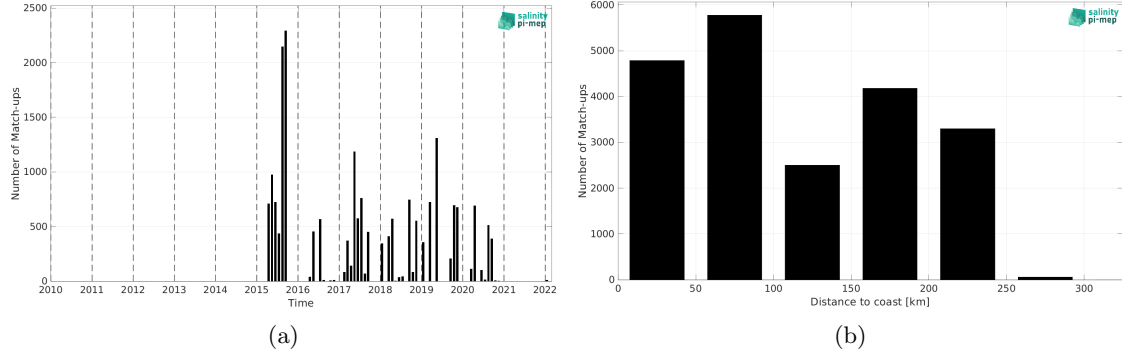
Figure 2: Number of match-ups between TSG (LEGOS-DM) and SMAP SSS L2 v5.3 - 40 km (RSS) SSS as a function of time (a) and as function of the distance to coast (b) over the Sea of Japan Pi-MEP region and for the full satellite product period.
