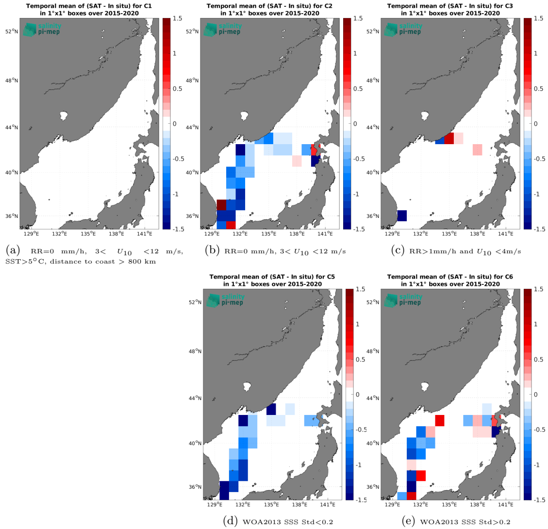
Figure 12: Temporal mean gridded over spatial boxes of size 1^\circ \times 1^\circ of \Delta\text{SSS} (SMAP SSS L2 v5 - 40 km (RSS) - TSG (LEGOS-DM)) for 5 different subdatasets corresponding to: RR=0 mm/h, 3 < U_{10} < 12 m/s, SST > 5^\circ\text{C} , distance to coast > 800 km (a), RR=0 mm/h, 3 < U_{10} < 12 m/s (b), RR > 1 mm/h and U_{10} < 4 m/s (c), WOA2013 SSS Std < 0.2 (d), WOA2013 SSS Std > 0.2 (e).
