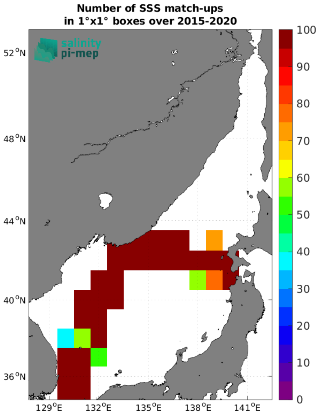
Figure 4: Number of SSS match-ups between TSG (LEGOS-DM) SSS and the SMAP SSS L2 v5 - 40 km (RSS) SSS product for the Sea of Japan Pi-MEP region over 1°x1° boxes and for the full satellite product period.
