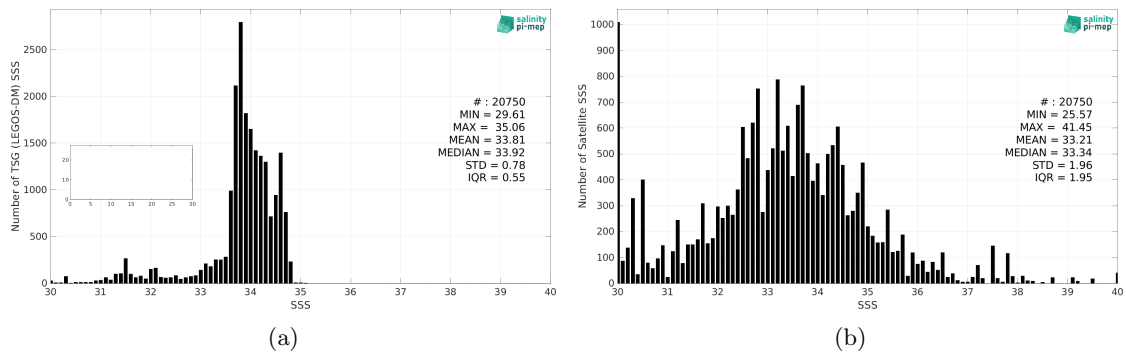
Figure 2: Histograms of SSS from TSG (LEGOS-DM) (a) and SMAP SSS L2 v5 - 40 km (RSS) (b) considering all match-up pairs per bins of 0.1 over the Sea of Japan Pi-MEP region and for the full satellite product period.
