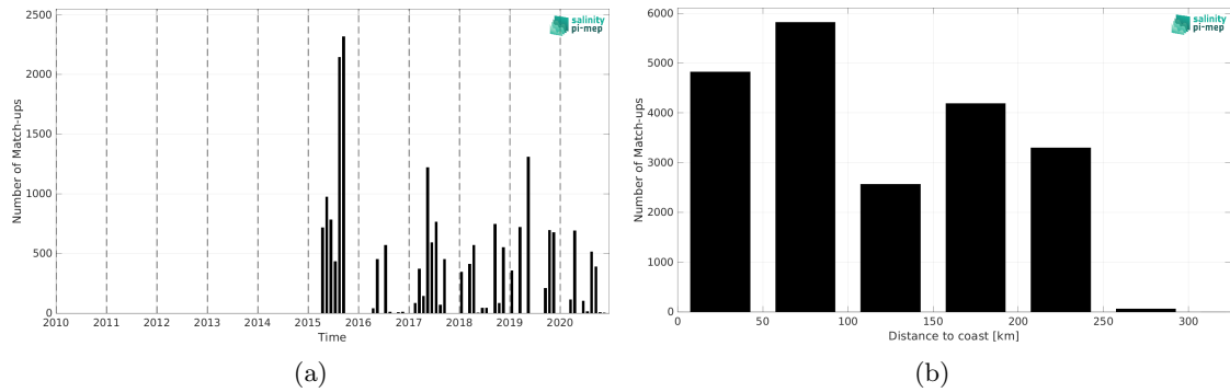
Figure 1: Number of match-ups between TSG (LEGOS-DM) and SMAP SSS L2 v5 - 40 km (RSS) SSS as a function of time (a) and as function of the distance to coast (b) over the Sea of Japan Pi-MEP region and for the full satellite product period.
