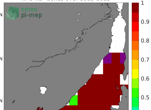
Temporal STD of (Sat - Argo) in 1°x1° boxes over 2015-2023
