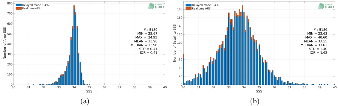
Figure 2: Histograms of SSS from Argo (a) and SMAP SSS L2 v5 - 40 km (RSS) (b) considering all match-up pairs per bins of 0.1 over the Sea of Japan Pi-MEP region and for the full satellite product period.
