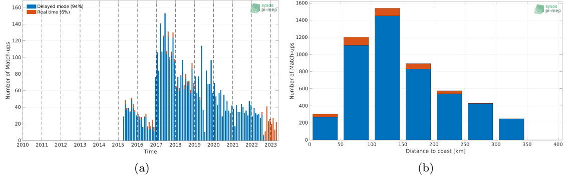
Figure 1: Number of match-ups between Argo and SMAP SSS L2 v5 - 40 km (RSS) SSS as a function of time (a) and as function of the distance to coast (b) over the Sea of Japan Pi-MEP region and for the full satellite product period.
