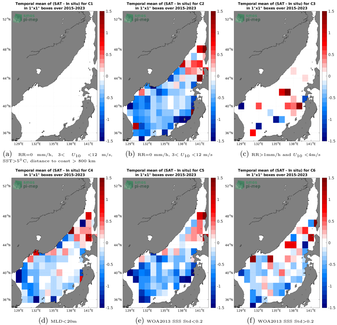
Figure 12: Temporal mean gridded over spatial boxes of size 1^\circ \times 1^\circ of \Delta SSS (SMAP SSS L2 v5 - 40 km (RSS) - Argo) for 6 different subdatasets corresponding to:RR=0 mm/h, 3 < U_{10} < 12 m/s, SST>5°C, distance to coast > 800 km (a), RR=0 mm/h, 3 < U_{10} < 12 m/s (b), RR>1mm/h and U_{10} < 4 m/s (c),MLD<20m (d),WOA2013 SSS Std<0.2 (e),WOA2013 SSS Std>0.2 (f).
