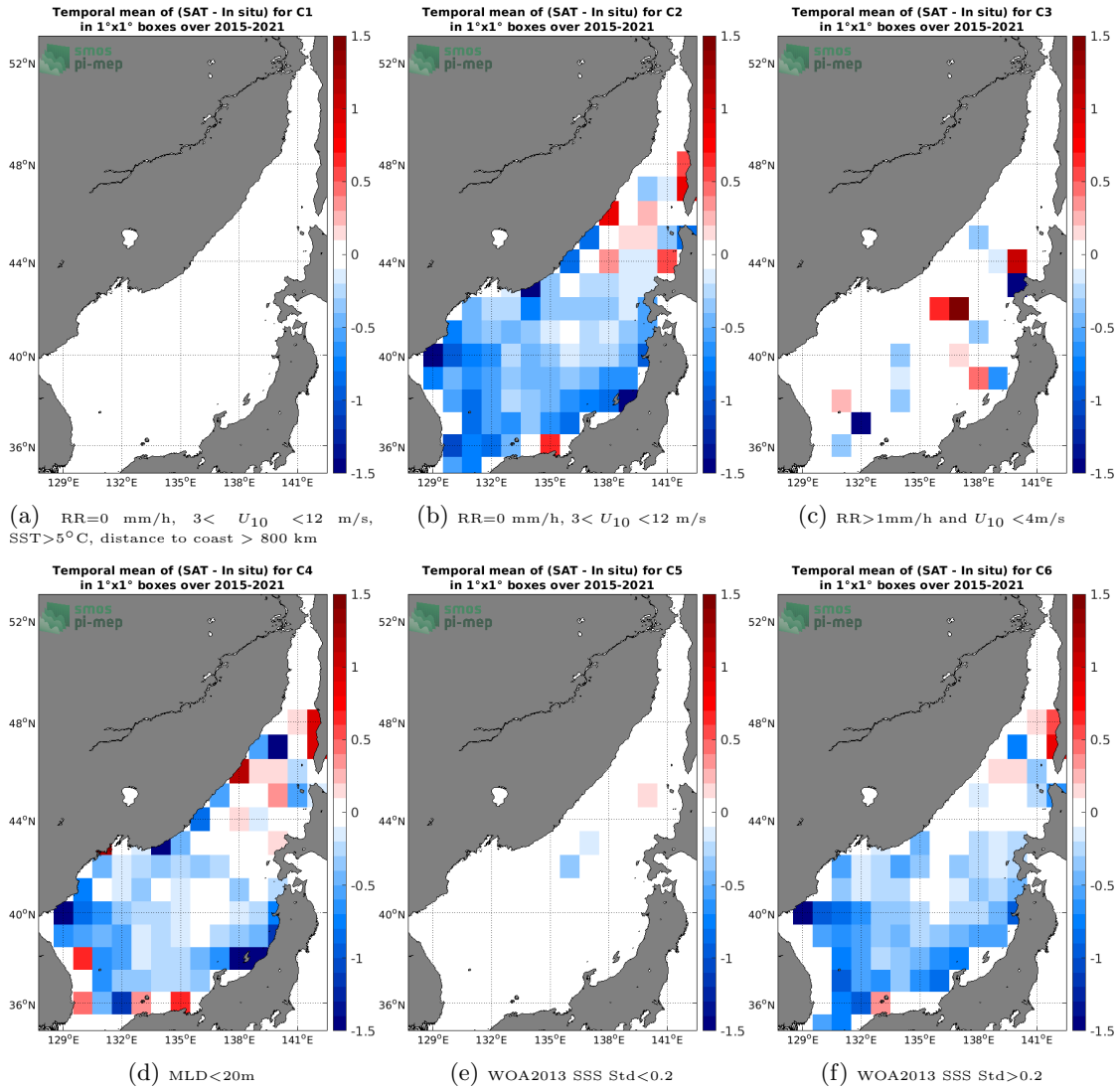
Figure 12: Temporal mean gridded over spatial boxes of size 1°x1° of \Delta SSS (SMAP SSS L2 v4 (RSS) - Argo) for 6 different subdatasets corresponding to:RR=0 mm/h, 3 < U_{10} < 12 m/s, SST>5°C, distance to coast > 800 km (a), RR=0 mm/h, 3 < U_{10} < 12 m/s (b), RR>1mm/h and U_{10} < 4 m/s (c),MLD<20m (d),WOA2013 SSS Std<0.2 (e),WOA2013 SSS Std>0.2 (f).
