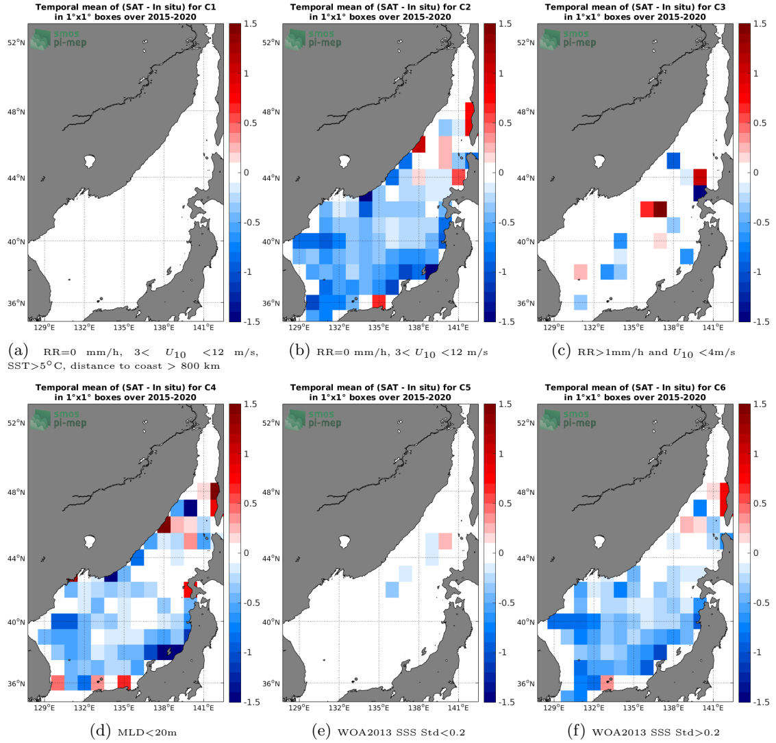
Figure 12: Temporal mean gridded over spatial boxes of size 1^\circ \times 1^\circ of \Delta SSS (SMAP SSS L2 v4 (RSS) - Argo) for 6 different subdatasets corresponding to: RR=0 mm/h, 3 < U_{10} < 12 m/s, SST>5°C, distance to coast > 800 km (a), RR=0 mm/h, 3 < U_{10} < 12 m/s (b), RR>1mm/h and U_{10} < 4 m/s (c),MLD<20m (d),WOA2013 SSS Std<0.2 (e),WOA2013 SSS Std>0.2 (f).
