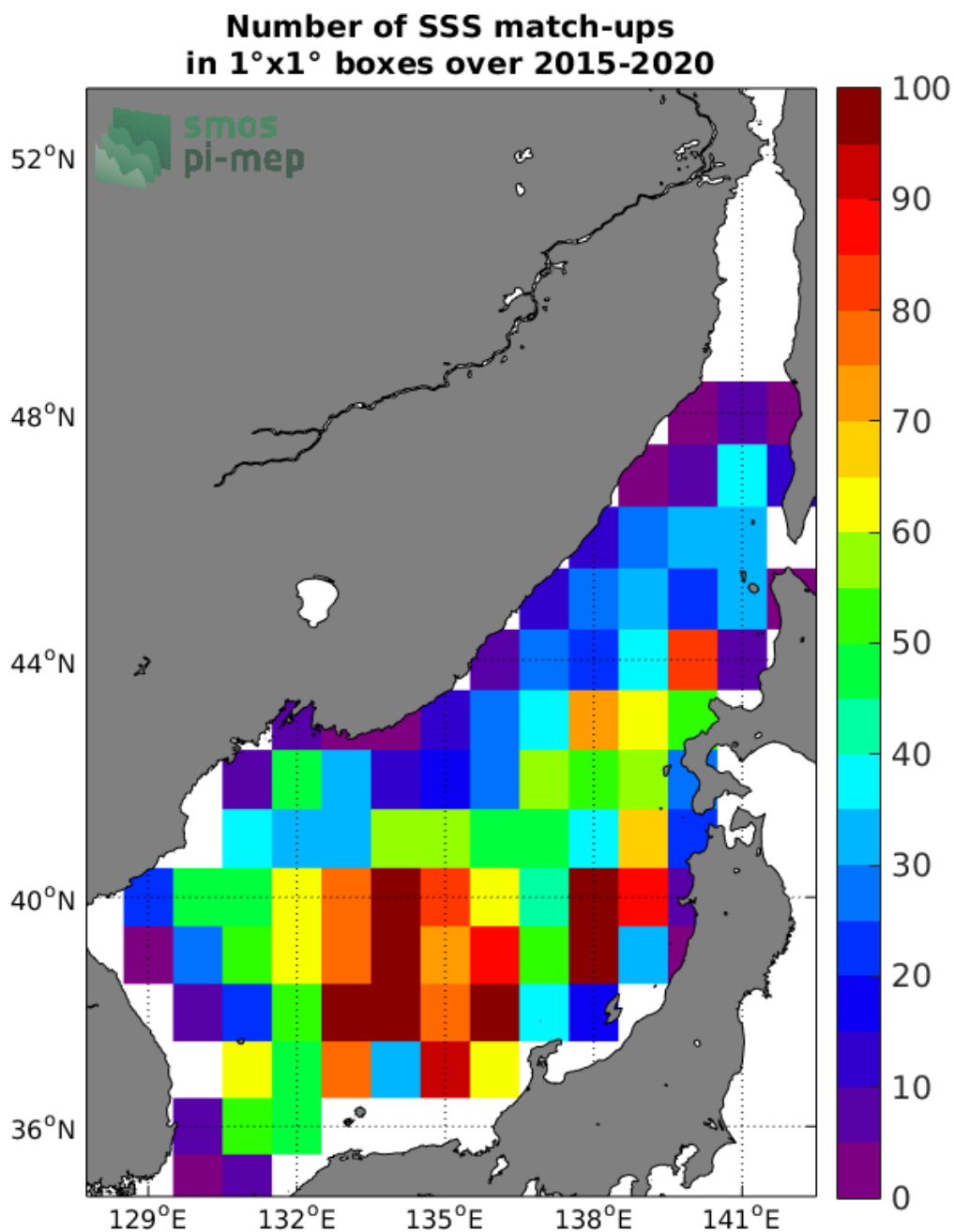
Figure 4: Number of SSS match-ups between Argo SSS and the SMAP SSS L2 v4 (RSS) SSS product for the Sea of Japan Pi-MEP region over 1°x1° boxes and for the full satellite product period.
