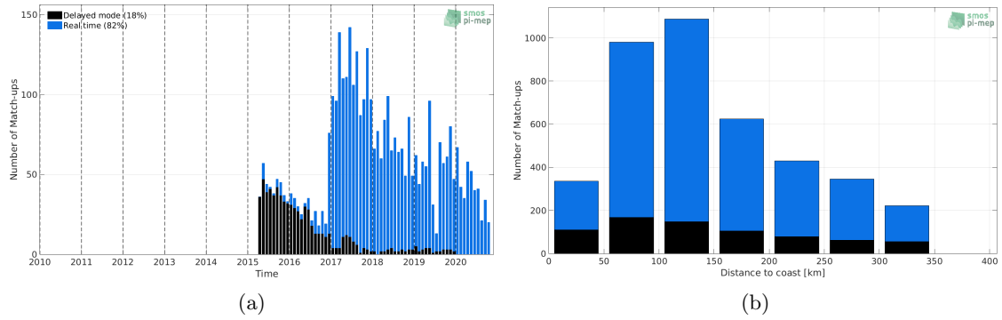
Figure 1: Number of match-ups between Argo and SMAP SSS L2 v4 (RSS) SSS as a function of time (a) and as function of the distance to coast (b) over the Sea of Japan Pi-MEP region and for the full satellite product period.
