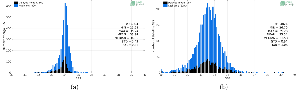
Figure 2: Histograms of SSS from Argo (a) and SMAP SSS L2 v4 (RSS) (b) considering all match-up pairs per bins of 0.1 over the Sea of Japan Pi-MEP region and for the full satellite product period.
