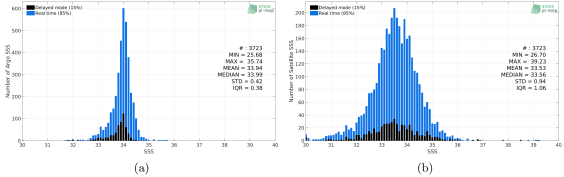
Figure 2: Histograms of SSS from Argo (a) and SMAP-L2-RSS-V4 (b) considering all match-up pairs per bins of 0.1 over the Sea of Japan Pi-MEP region and for the full satellite product period.
