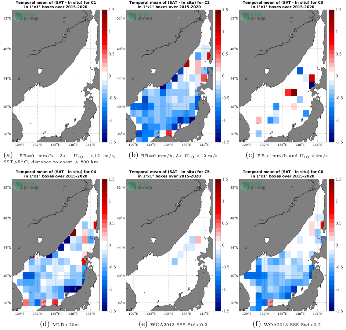
Figure 12: Temporal mean gridded over spatial boxes of size 1°x1° of \Delta SSS (SMAP-L2-RSS-V4 - Argo) for 6 different subdatasets corresponding to: RR=0 mm/h, 3 < U_{10} < 12 m/s, SST > 5°C, distance to coast > 800 km (a), RR=0 mm/h, 3 < U_{10} < 12 m/s (b), RR > 1 mm/h and U_{10} < 4 m/s (c), MLD < 20m (d), WOA2013 SSS Std < 0.2 (e), WOA2013 SSS Std > 0.2 (f).
