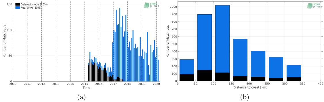
Figure 1: Number of match-ups between Argo and SMAP-L2-RSS-V4 SSS as a function of time (a) and as function of the distance to coast (b) over the Sea of Japan Pi-MEP region and for the full satellite product period.
