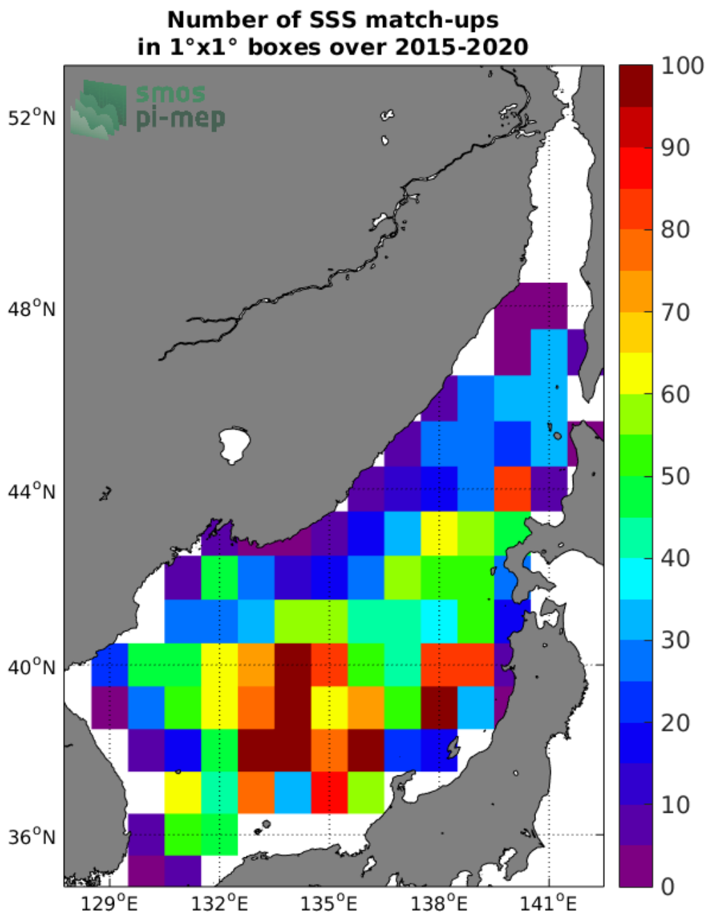
Figure 4: Number of SSS match-ups between Argo SSS and the SMAP-L2-RSS-V4 SSS product for the Sea of Japan Pi-MEP region over 1°x1° boxes and for the full satellite product period.
