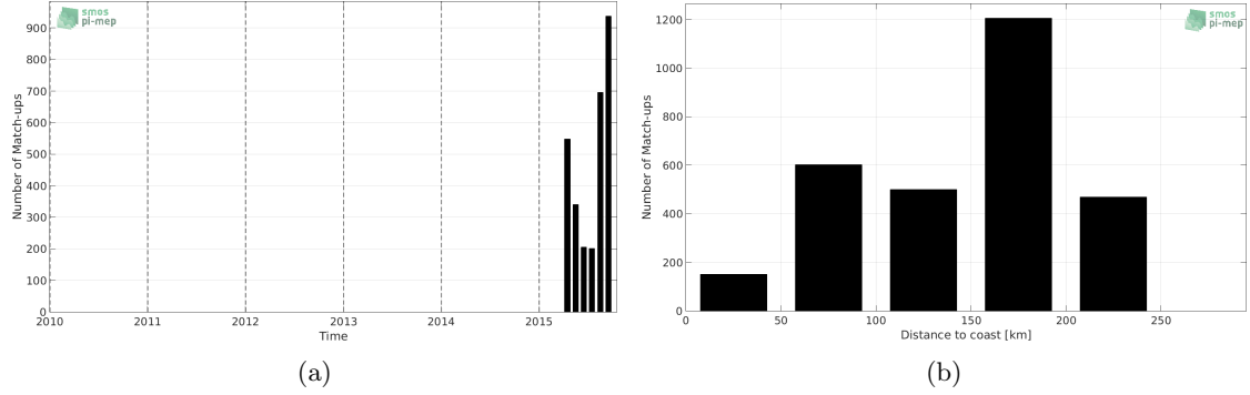
Figure 1: Number of match-ups between TSG-LEGOS-DM and SMAP-L2-RSS-V3-70KM SSS as a function of time (a) and as function of the distance to coast (b) over the Sea of Japan Pi-MEP region and for the full satellite product period.
