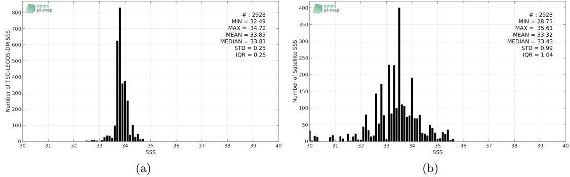
Figure 2: Histograms of SSS from TSG-LEGOS-DM (a) and SMAP-L2-RSS-V3-70KM (b) considering all match-up pairs per bins of 0.1 over the Sea of Japan Pi-MEP region and for the full satellite product period.
