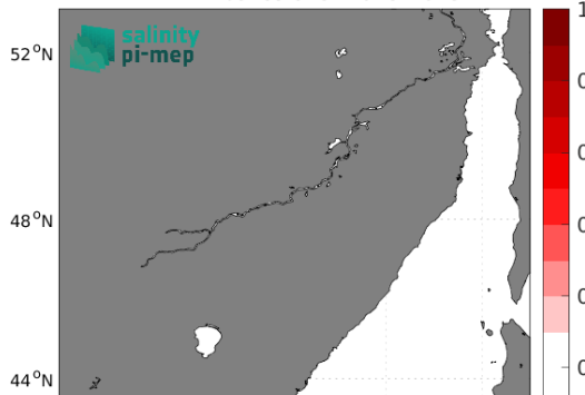
Temporal mean of (Sat - TSG (LEGOS-DM)) in 1°x1° boxes over 2015-2023
