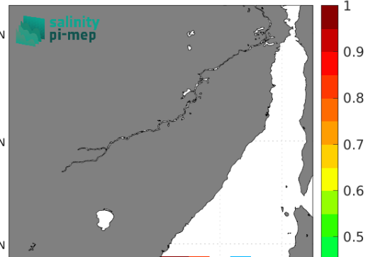
Temporal STD of (Sat - TSG (LEGOS-DM)) in 1°x1° boxes over 2015-2023
