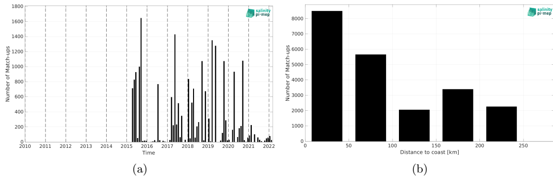
Figure 2: Number of match-ups between TSG (LEGOS-DM) and SMAP SSS L2 v5.0 (JPL) SSS as a function of time (a) and as function of the distance to coast (b) over the Sea of Japan Pi-MEP region and for the full satellite product period.
