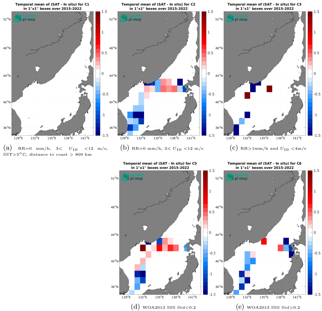
Figure 14: Temporal mean gridded over spatial boxes of size 1^\circ \times 1^\circ of \Delta\text{SSS} (SMAP SSS L2 v5.0 (JPL) - TSG (LEGOS-DM)) for 5 different subdatasets corresponding to: RR=0 mm/h, 3 < U_{10} < 12 m/s, SST > 5^\circ\text{C} , distance to coast > 800 km (a), RR=0 mm/h, 3 < U_{10} < 12 m/s (b), RR > 1 mm/h and U_{10} < 4 m/s (c), WOA2013 SSS Std < 0.2 (d), WOA2013 SSS Std > 0.2 (e).
