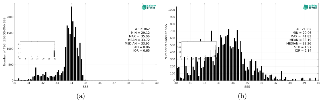
Figure 3: Histograms of SSS from TSG (LEGOS-DM) (a) and SMAP SSS L2 v5.0 (JPL) (b) considering all match-up pairs per bins of 0.1 over the Sea of Japan Pi-MEP region and for the full satellite product period.
