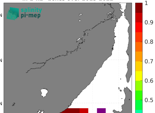
Temporal STD of (Sat - TSG (LEGOS-DM)) in 1°x1° boxes over 2015-2022
