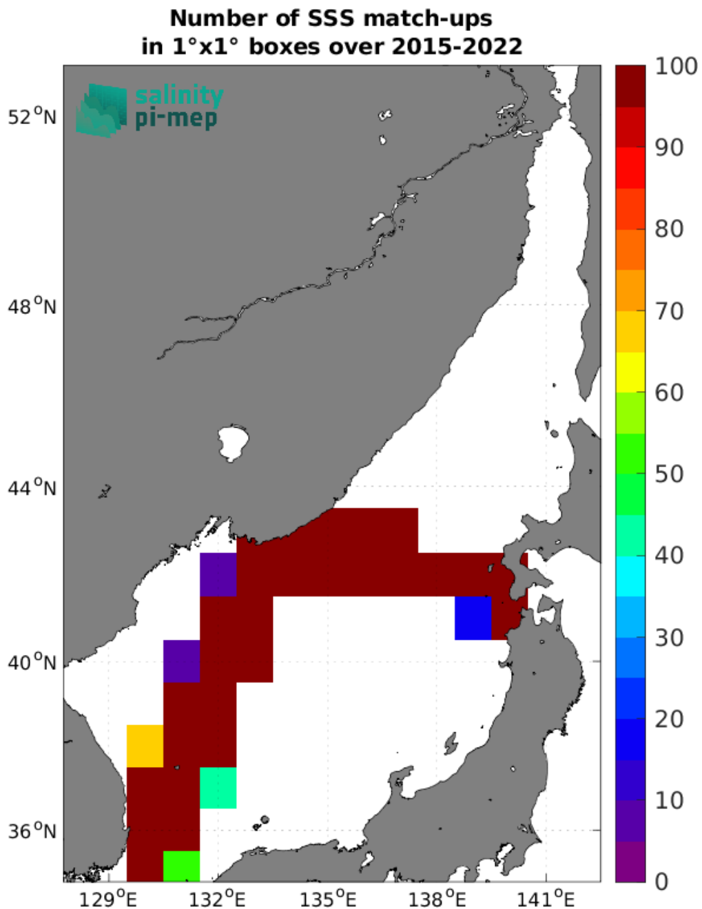
Figure 5: Number of SSS match-ups between TSG (LEGOS-DM) SSS and the SMAP SSS L2 v5.0 (JPL) SSS product for the Sea of Japan Pi-MEP region over 1°×1° boxes and for the full satellite product period.
