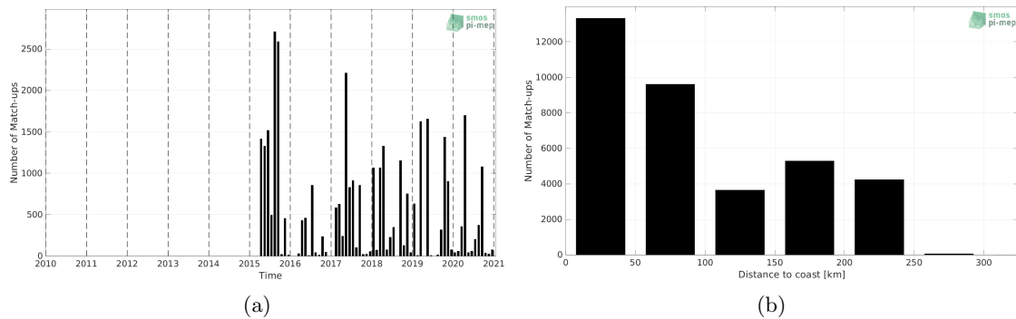
Figure 1: Number of match-ups between TSG (LEGOS-DM) and SMAP SSS L2 v5.0 (JPL) SSS as a function of time (a) and as function of the distance to coast (b) over the Sea of Japan Pi-MEP region and for the full satellite product period.
