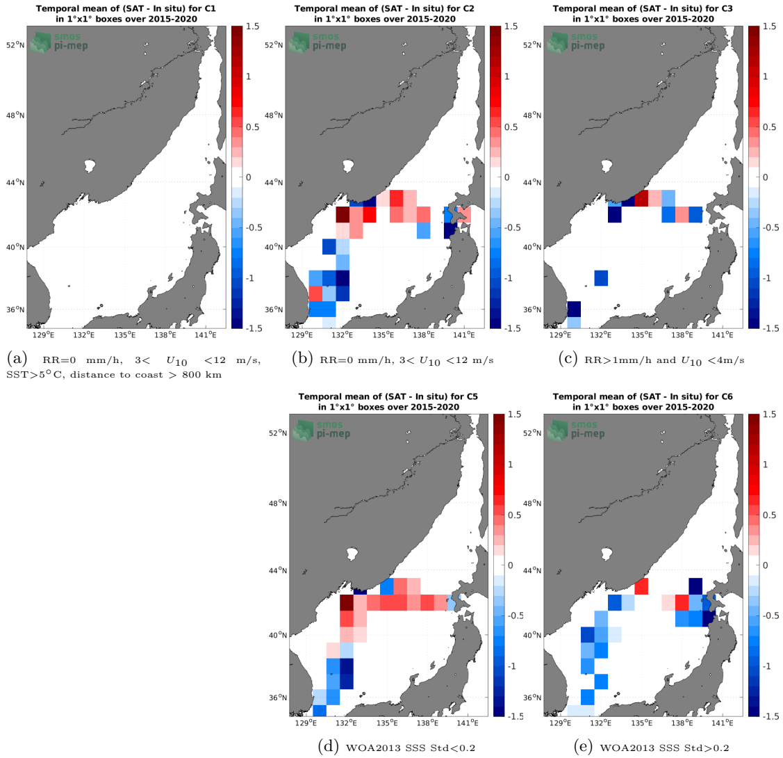
Figure 12: Temporal mean gridded over spatial boxes of size 1^\circ \times 1^\circ of \Delta SSS (SMAP SSS L2 v5.0 (JPL) - TSG (LEGOS-DM)) for 5 different subdatasets corresponding to: RR=0 mm/h, 3 < U_{10} < 12 m/s, SST > 5^\circ C , distance to coast > 800 km (a), RR=0 mm/h, 3 < U_{10} < 12 m/s (b), RR > 1 mm/h and U_{10} < 4 m/s (c), WOA2013 SSS Std < 0.2 (d), WOA2013 SSS Std > 0.2 (e).
