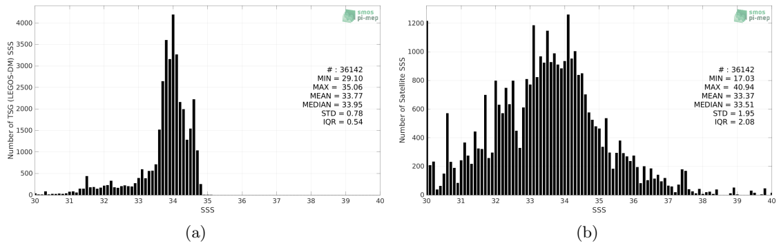
Figure 2: Histograms of SSS from TSG (LEGOS-DM) (a) and SMAP SSS L2 v5.0 (JPL) (b) considering all match-up pairs per bins of 0.1 over the Sea of Japan Pi-MEP region and for the full satellite product period.
