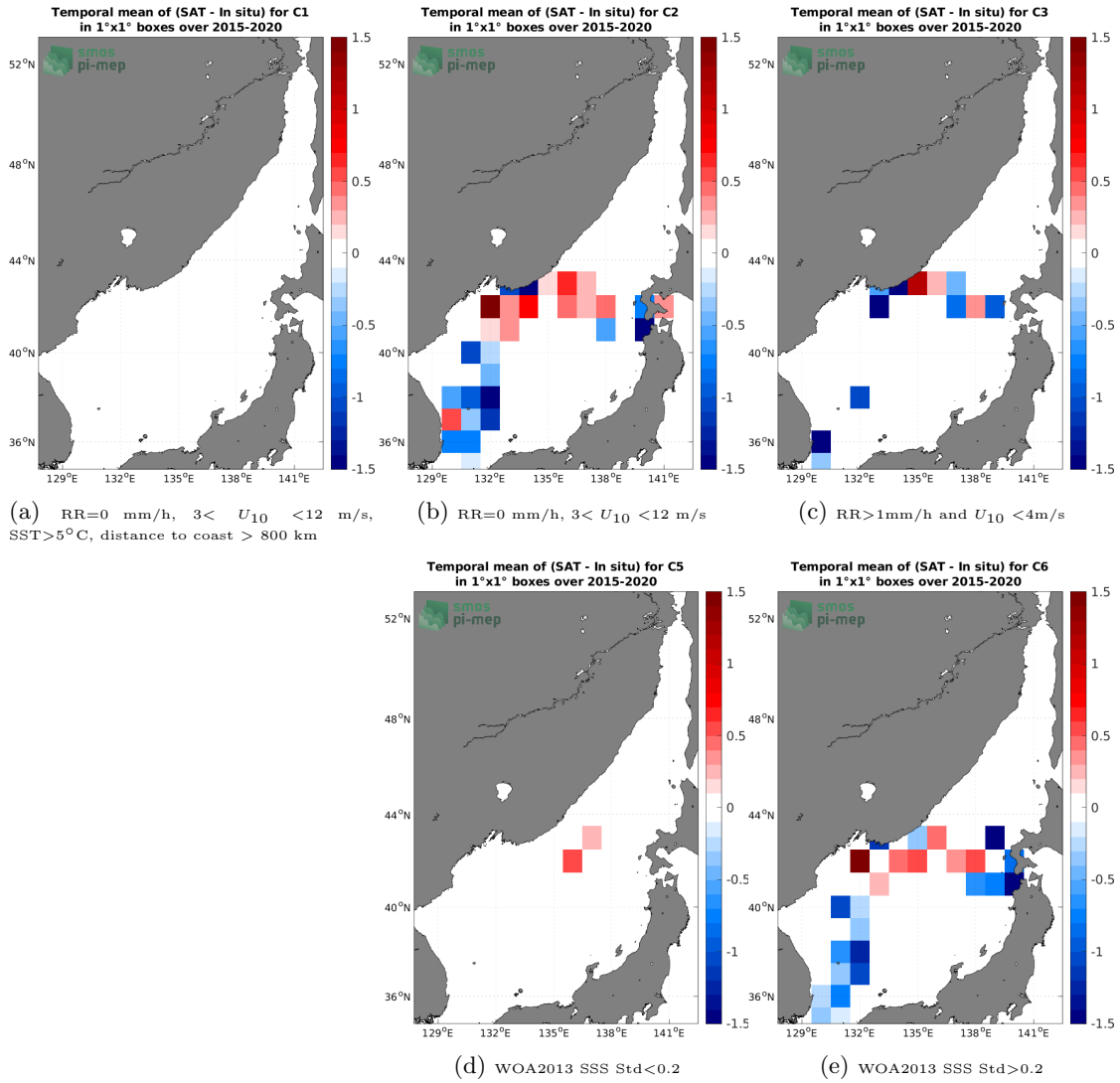
Figure 12: Temporal mean gridded over spatial boxes of size 1^\circ \times 1^\circ of \Delta\text{SSS} (SMAP SSS L2 v5.0 (JPL) - TSG (LEGOS-DM)) for 5 different subdatasets corresponding to: RR=0 mm/h, 3 < U_{10} < 12 m/s, SST > 5^\circ\text{C} , distance to coast > 800 km (a), RR=0 mm/h, 3 < U_{10} < 12 m/s (b), RR > 1 mm/h and U_{10} < 4 m/s (c), WOA2013 SSS Std < 0.2 (d), WOA2013 SSS Std > 0.2 (e).
