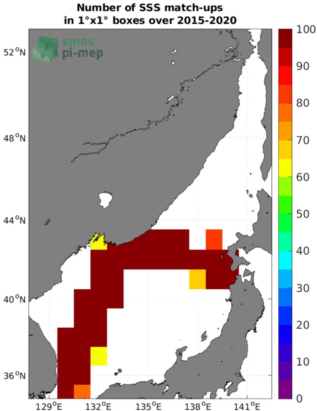
Figure 4: Number of SSS match-ups between TSG (LEGOS-DM) SSS and the SMAP SSS L2 v5.0 (JPL) SSS product for the Sea of Japan Pi-MEP region over 1°×1° boxes and for the full satellite product period.
