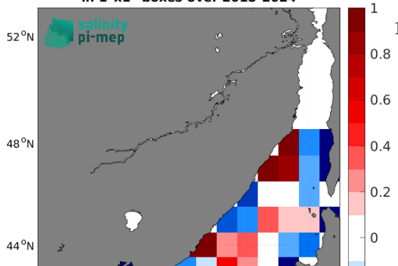
Temporal mean of (Sat - Argo) in 1°x1° boxes over 2015-2024
