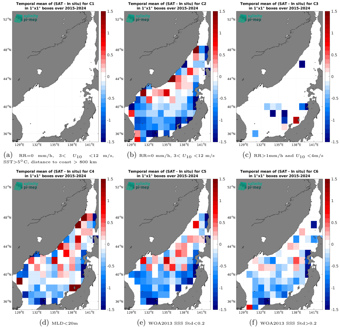
Figure 14: Temporal mean gridded over spatial boxes of size 1^\circ \times 1^\circ of \Delta SSS (SMAP SSS L2 v5.0 (JPL) - Argo) for 6 different subdatasets corresponding to: RR=0 mm/h, 3 < U_{10} < 12 m/s, SST > 5°C, distance to coast > 800 km (a), RR=0 mm/h, 3 < U_{10} < 12 m/s (b), RR > 1mm/h and U_{10} < 4 m/s (c), MLD < 20m (d), WOA2013 SSS Std < 0.2 (e), WOA2013 SSS Std > 0.2 (f).
