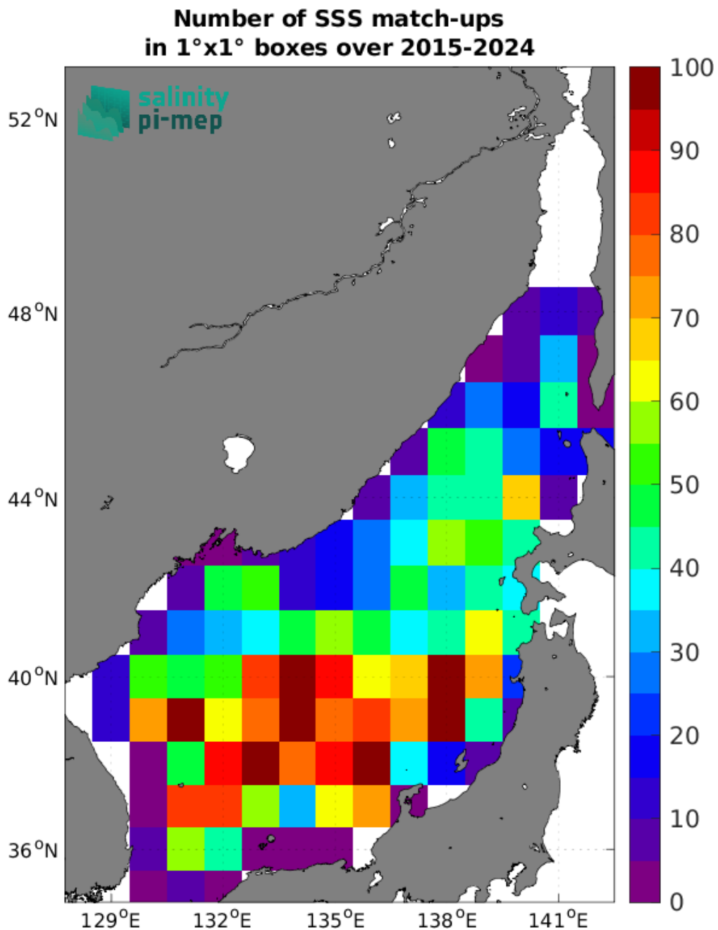
Figure 5: Number of SSS match-ups between Argo SSS and the SMAP SSS L2 v5.0 (JPL) SSS product for the Sea of Japan Pi-MEP region over 1°x1° boxes and for the full satellite product period.
