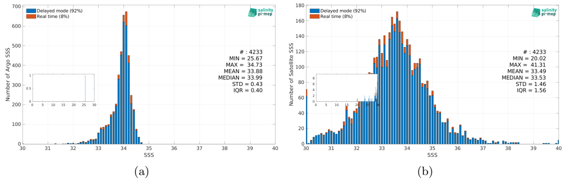
Figure 3: Histograms of SSS from Argo (a) and SMAP SSS L2 v5.0 (JPL) (b) considering all match-up pairs per bins of 0.1 over the Sea of Japan Pi-MEP region and for the full satellite product period.
