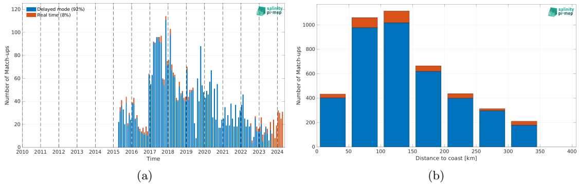
Figure 2: Number of match-ups between Argo and SMAP SSS L2 v5.0 (JPL) SSS as a function of time (a) and as function of the distance to coast (b) over the Sea of Japan Pi-MEP region and for the full satellite product period.
