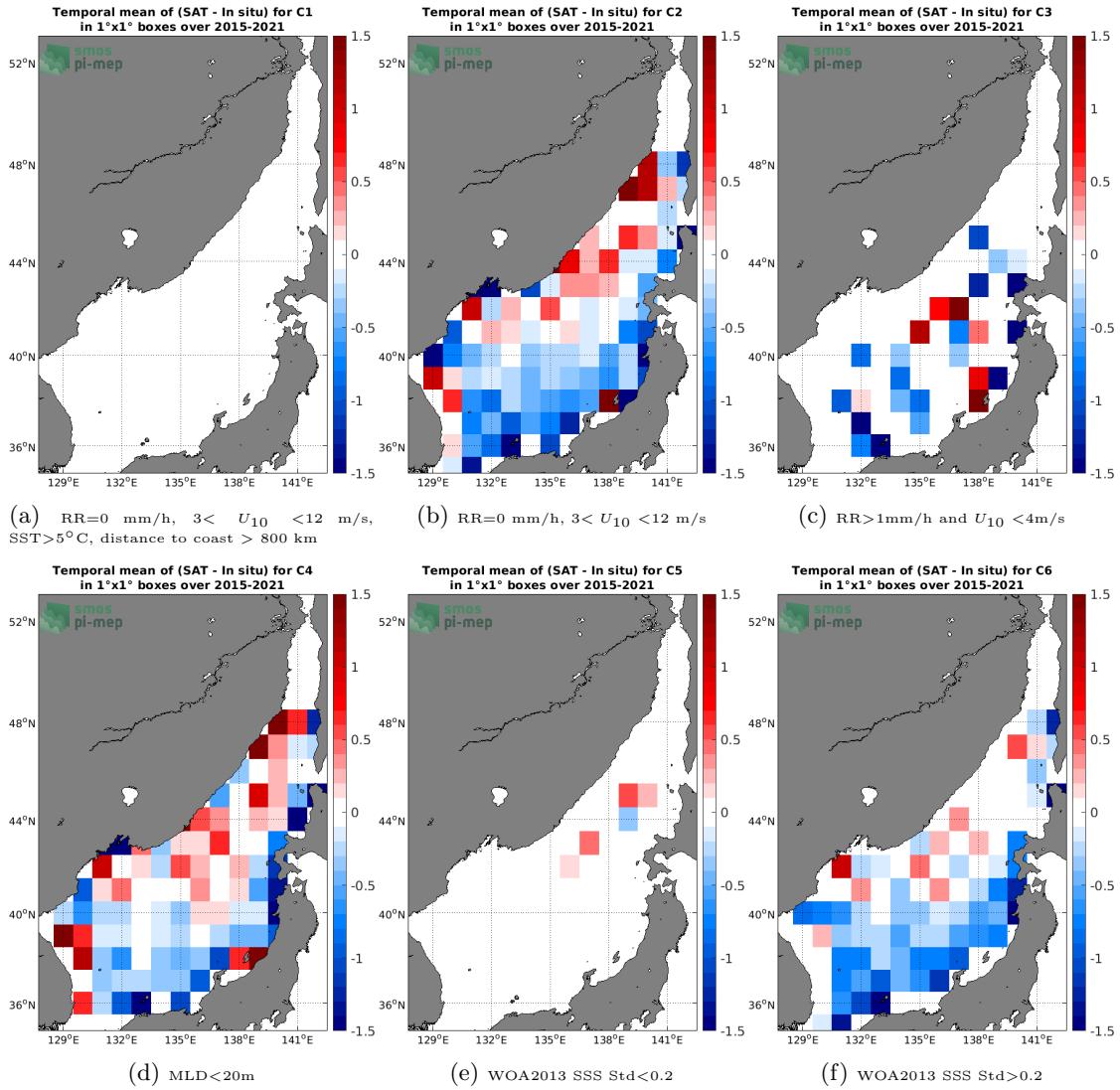
Figure 12: Temporal mean gridded over spatial boxes of size 1°x1° of \Delta SSS (SMAP SSS L2 v5.0 (JPL) - Argo) for 6 different subdatasets corresponding to:RR=0 mm/h, 3 < U_{10} < 12 m/s, SST>5°C, distance to coast > 800 km (a), RR=0 mm/h, 3 < U_{10} < 12 m/s (b), RR>1mm/h and U_{10} < 4 m/s (c),MLD<20m (d),WOA2013 SSS Std<0.2 (e),WOA2013 SSS Std>0.2 (f).
