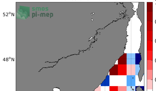
Temporal mean of (Sat - Argo) in 1°x1° boxes over 2015-2021
