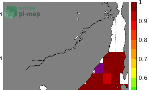
Temporal STD of (Sat - Argo) in 1°x1° boxes over 2015-2021
