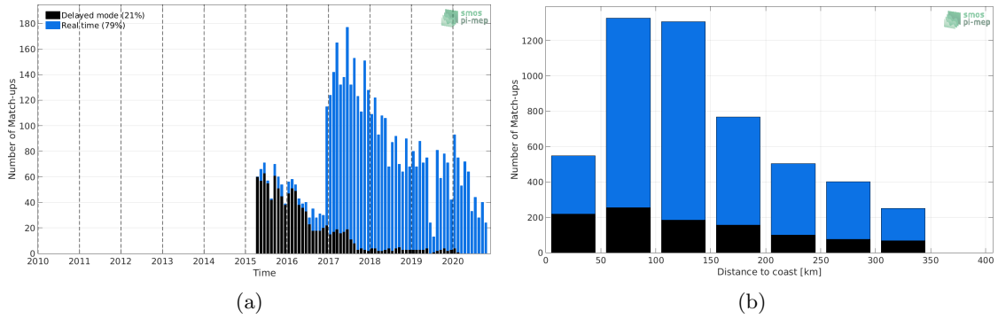
Figure 1: Number of match-ups between Argo and SMAP SSS L2 v5.0 (JPL) SSS as a function of time (a) and as function of the distance to coast (b) over the Sea of Japan Pi-MEP region and for the full satellite product period.
