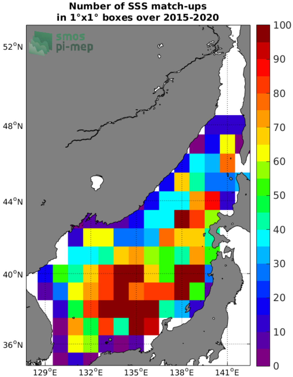
Figure 4: Number of SSS match-ups between Argo SSS and the SMAP SSS L2 v5.0 (JPL) SSS product for the Sea of Japan Pi-MEP region over 1°x1° boxes and for the full satellite product period.
