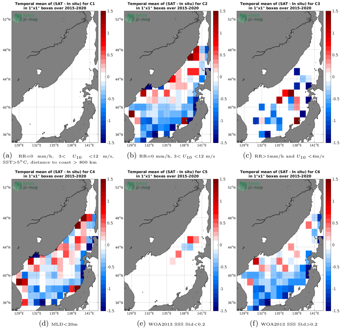
Figure 12: Temporal mean gridded over spatial boxes of size 1^\circ \times 1^\circ of \Delta\text{SSS} (SMAP SSS L2 v5.0 (JPL) - Argo) for 6 different subdatasets corresponding to: RR=0 mm/h, 3 < U_{10} < 12 m/s, SST > 5^\circ\text{C} , distance to coast > 800 km (a), RR=0 mm/h, 3 < U_{10} < 12 m/s (b), RR > 1\text{mm/h} and U_{10} < 4\text{m/s} (c), MLD < 20\text{m} (d), WOA2013 SSS Std < 0.2 (e), WOA2013 SSS Std > 0.2 (f).
