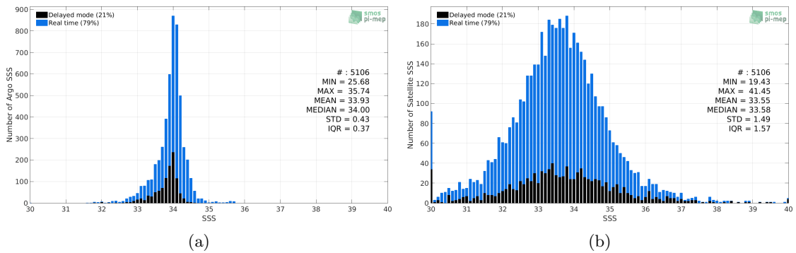
Figure 2: Histograms of SSS from Argo (a) and SMAP SSS L2 v5.0 (JPL) (b) considering all match-up pairs per bins of 0.1 over the Sea of Japan Pi-MEP region and for the full satellite product period.
