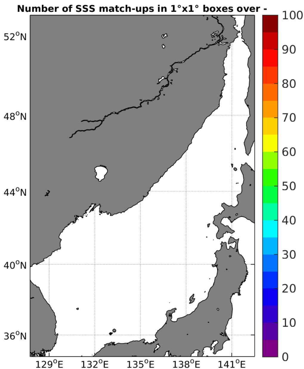
Figure 4: Number of SSS match-ups between TSG-SAMOS SSS and the SMAP-L2-JPL-V4 SSS product for the Sea of Japan Pi-MEP region over 1°x1° boxes and for the full satellite product period.
