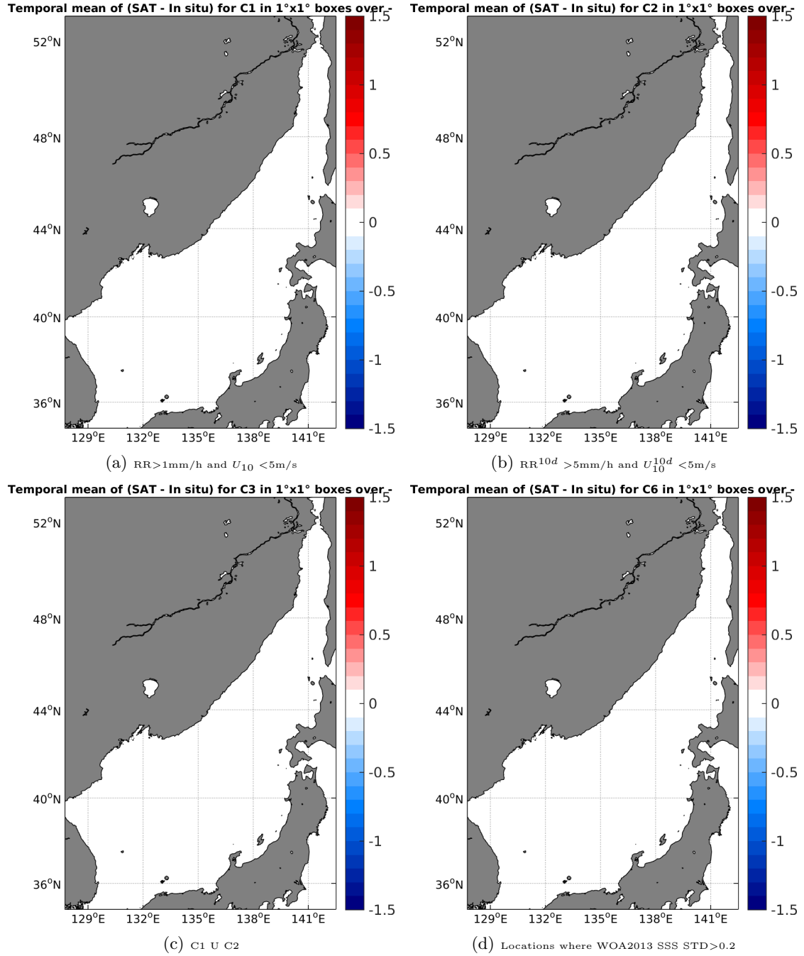
Figure 12: Temporal mean gridded over spatial boxes of size 1°x1° of \Delta\text{SSS} (SMAP-L2-JPL-V4 - TSG-SAMOS) for 4 different subdatasets corresponding to: RR > 1mm/h and U_{10} < 5\text{m/s} (a), RR^{10d} > 5\text{mm/h} and U_{10}^{10d} < 5\text{m/s} (b), C1 U C2 (c), Locations where WOA2013 SSS STD > 0.2 (d).
