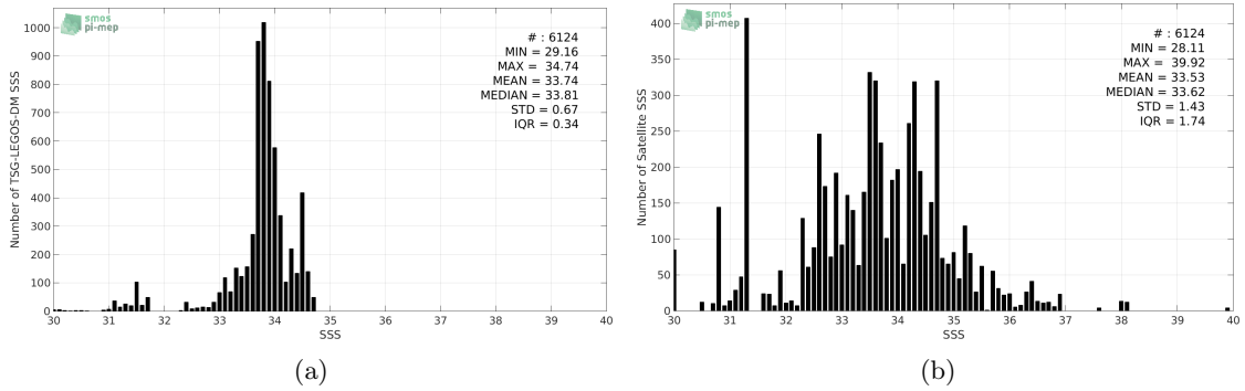
Figure 2: Histograms of SSS from TSG-LEGOS-DM (a) and SMAP-L2-JPL-V4 (b) considering all match-up pairs per bins of 0.1 over the Sea of Japan Pi-MEP region and for the full satellite product period.
