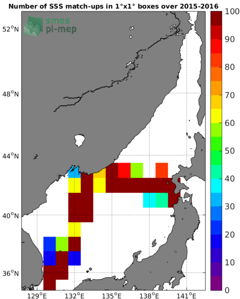
Figure 4: Number of SSS match-ups between TSG-LEGOS-DM SSS and the SMAP-L2-JPL-V4 SSS product for the Sea of Japan Pi-MEP region over 1°x1° boxes and for the full satellite product period.
