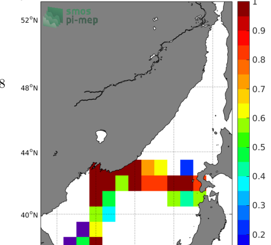
Temporal STD of (Sat-TSG-LEGOS-DM) in 1°x1° boxes over 2015-2016
