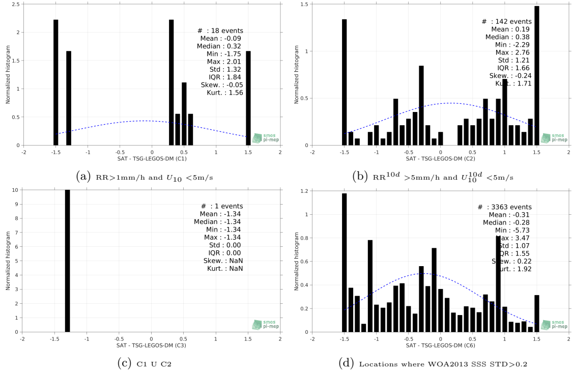
Figure 13: Normalized histogram of \Delta SSS (SMAP-L2-JPL-V4 - TSG-LEGOS-DM) for 6 different subdatasets corresponding to: RR > 1mm/h and U_{10} < 5 m/s (a), RR^{10d} > 5 mm/h and U_{10}^{10d} < 5 m/s (b), C1 U C2 (c), Locations where WOA2013 SSS STD > 0.2 (d).
