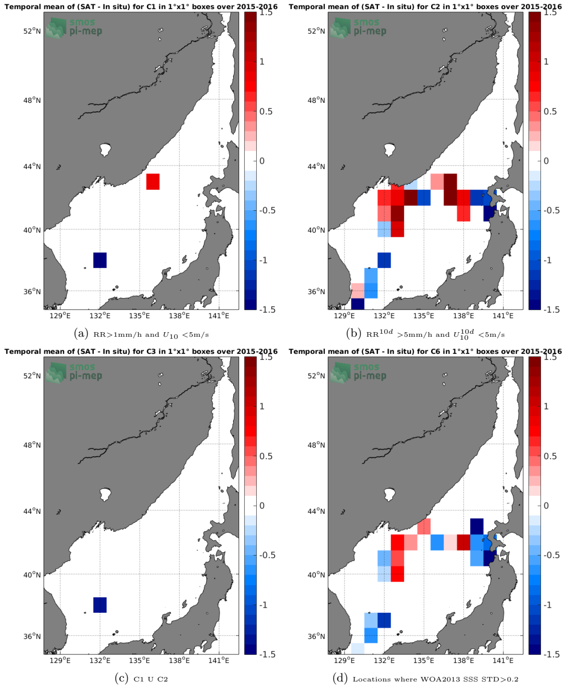
Figure 12: Temporal mean gridded over spatial boxes of size 1°x1° of \Delta\text{SSS} (SMAP-L2-JPL-V4 - TSG-LEGOS-DM) for 4 different subdatasets corresponding to: RR > 1\text{mm/h} and U_{10} < 5\text{m/s} (a), RR^{10d} > 5\text{mm/h} and U_{10}^{10d} < 5\text{m/s} (b), C1 U C2 (c), Locations where WOA2013 SSS STD > 0.2 (d).
