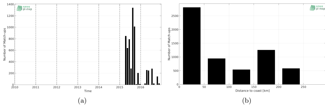
Figure 1: Number of match-ups between TSG-LEGOS-DM and SMAP-L2-JPL-V4 SSS as a function of time (a) and as function of the distance to coast (b) over the Sea of Japan Pi-MEP region and for the full satellite product period.
