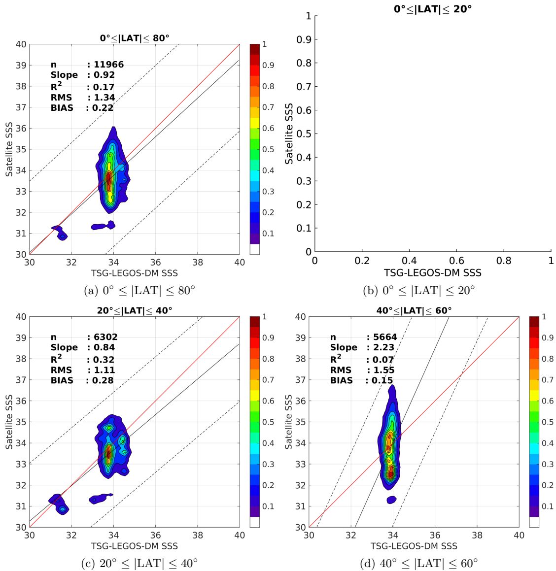
Figure 9: Contour maps of the concentration of SMAP-L2-JPL-V4 SSS (y-axis) versus TSG-LEGOS-DM SSS (x-axis) at match-up pairs for different latitude bands. For each plot, the red line shows x=y . The black thin and dashed lines indicate a linear fit through the data cloud and the \pm 95\% confidence levels, respectively. The number match-up pairs n , the slope and R^2 coefficient of the linear fit, the root mean square (RMS) and the mean bias between satellite and in situ data are indicated for each latitude band in each plots.
