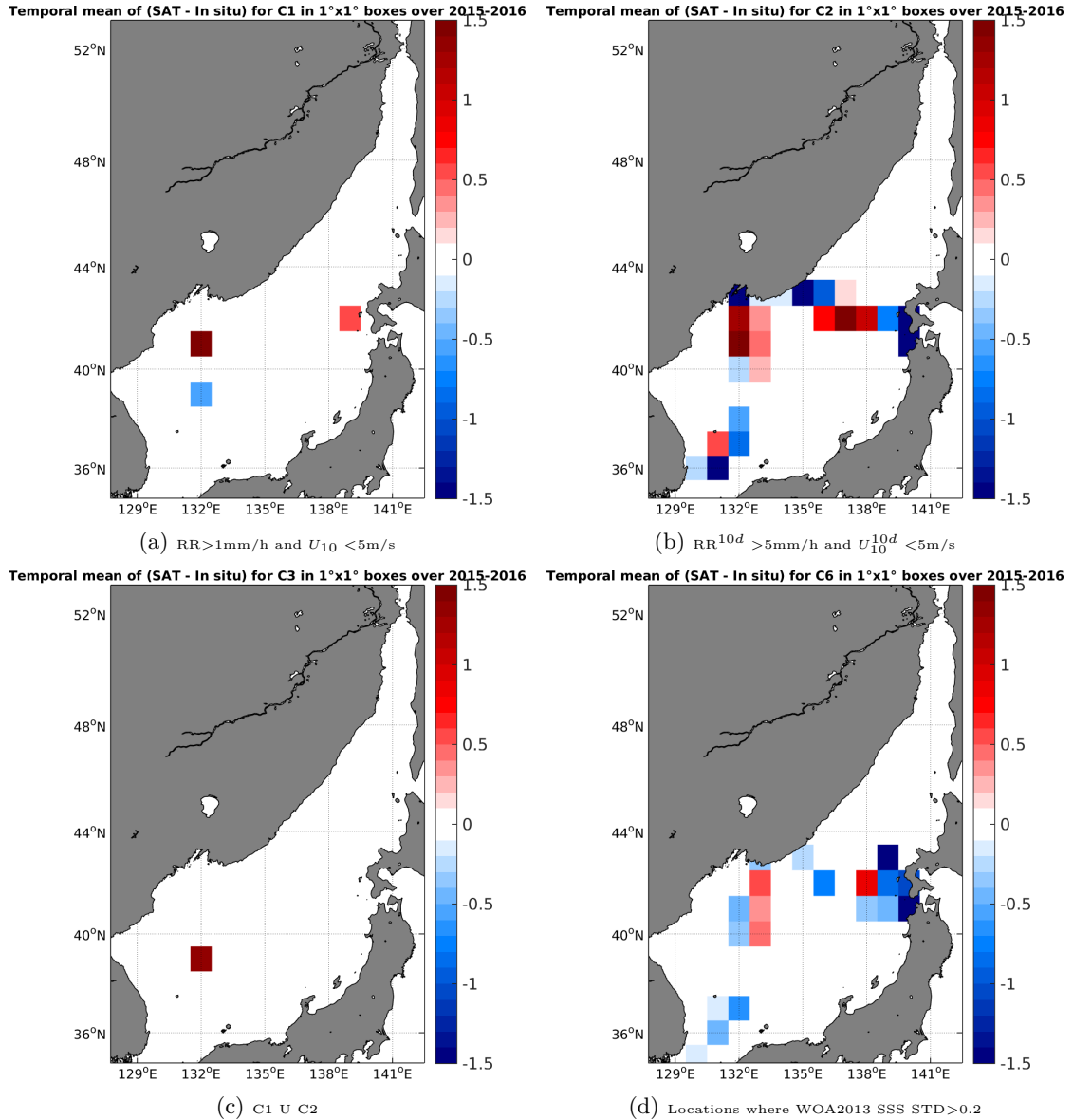
Figure 12: Temporal mean gridded over spatial boxes of size 1°x1° of \Delta SSS (SMAP-L2-JPL-V4 - TSG-LEGOS-DM) for 4 different subdatasets corresponding to:RR>1mm/h and U_{10} < 5\text{m/s} (a), RR^{10d} > 5\text{mm/h} and U_{10}^{10d} < 5\text{m/s} (b), C1 U C2 (c),Locations where WOA2013 SSS STD>0.2 (d).
