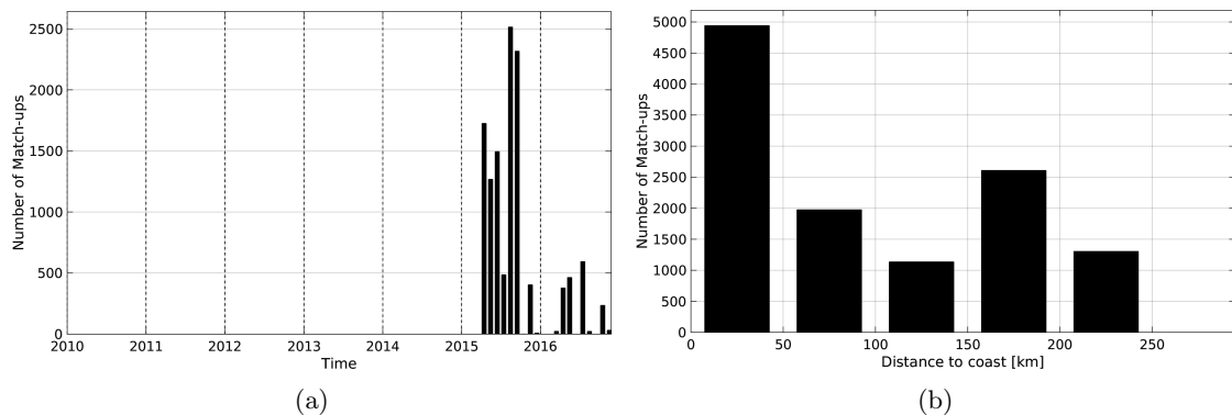
Figure 1: Number of match-ups between TSG-LEGOS-DM and SMAP-L2-JPL-V4 SSS as a function of time (a) and as function of the distance to coast (b) over the Sea of Japan Pi-MEP region and for the full satellite product period.
