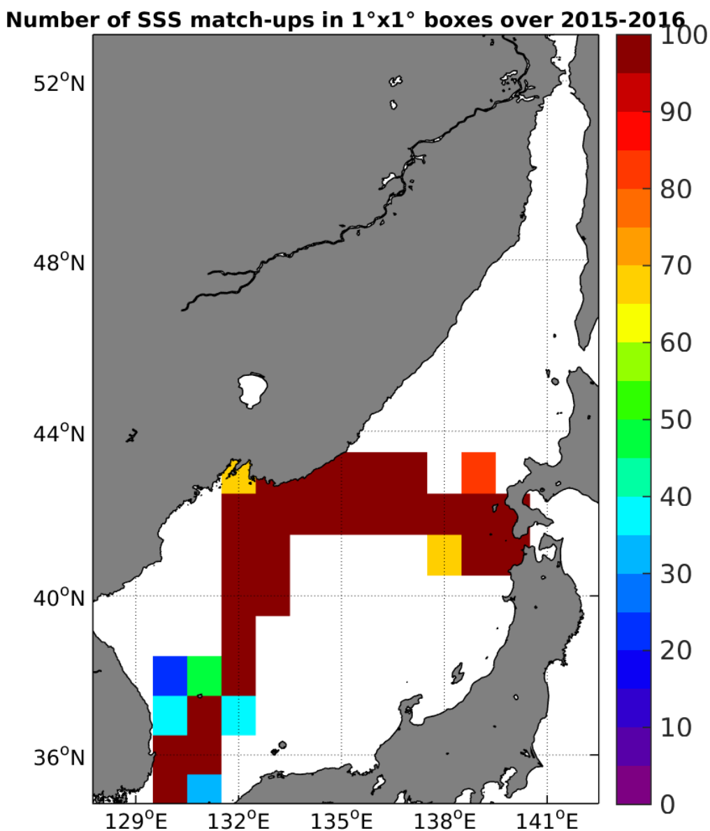
Figure 4: Number of SSS match-ups between TSG-LEGOS-DM SSS and the SMAP-L2-JPL-V4 SSS product for the Sea of Japan Pi-MEP region over 1°x1° boxes and for the full satellite product period.
