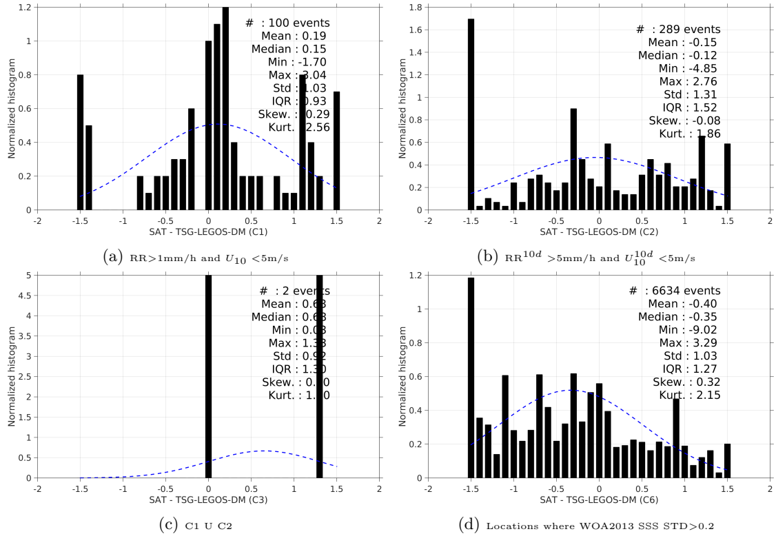
Figure 13: Normalized histogram of \Delta\text{SSS} (SMAP-L2-JPL-V4 - TSG-LEGOS-DM) for 6 different subdatasets corresponding to: \text{RR} > 1\text{mm/h} and U_{10} < 5\text{m/s} (a), \text{RR}^{10d} > 5\text{mm/h} and U_{10}^{10d} < 5\text{m/s} (b), C1 U C2 (c), Locations where WOA2013 SSS STD > 0.2 (d).
