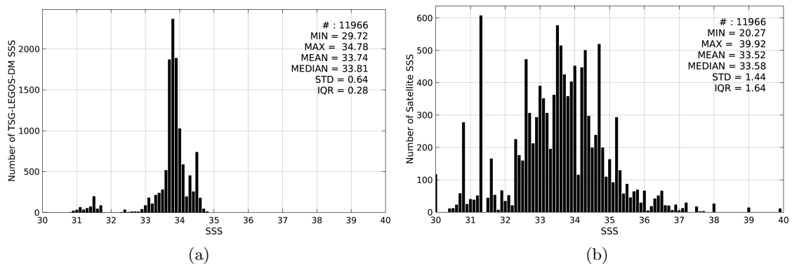
Figure 2: Histograms of SSS from TSG-LEGOS-DM (a) and SMAP-L2-JPL-V4 (b) considering all match-up pairs per bins of 0.1 over the Sea of Japan Pi-MEP region and for the full satellite product period.
