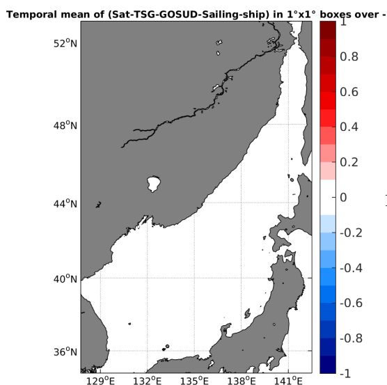
(e) MEAN( \Delta SSS) (Satellite - TSG-GOSUD-Sailing-ship)
