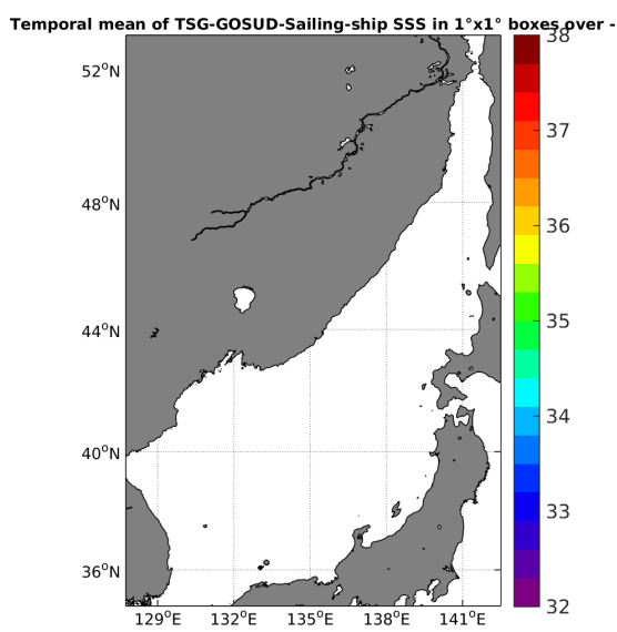
(c) MEAN(TSG-GOSUD-Sailing-ship SSS)
