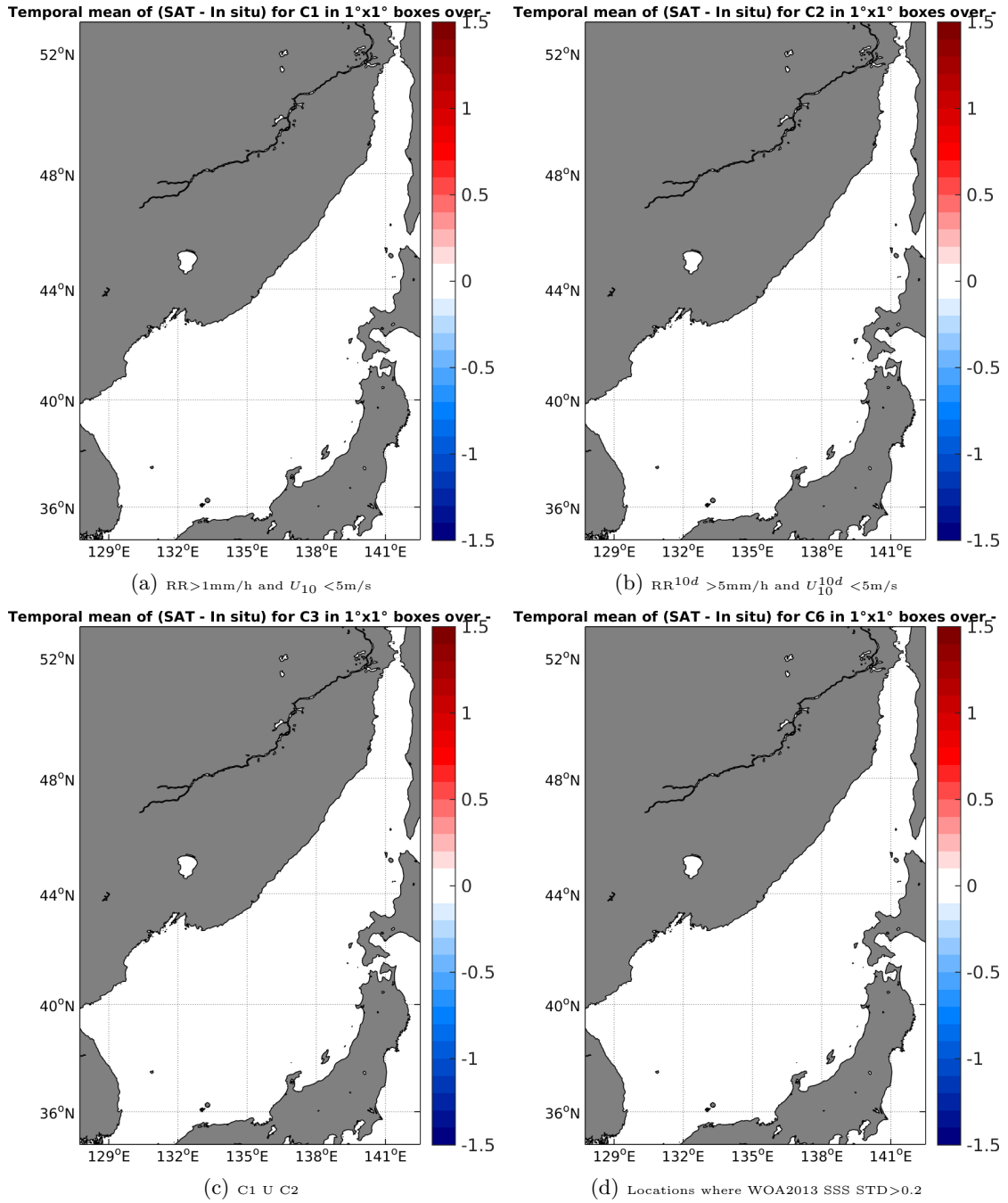
Figure 12: Temporal mean gridded over spatial boxes of size 1°x1° of \Delta\text{SSS} (SMAP-L2-JPL-V4 - TSG-GOSUD-Sailing-ship) for 4 different subdatasets corresponding to: RR > 1\text{mm/h} and U_{10} < 5\text{m/s} (a), RR^{10d} > 5\text{mm/h} and U_{10}^{10d} < 5\text{m/s} (b), C1 U C2 (c), Locations where WOA2013 SSS STD > 0.2 (d).
