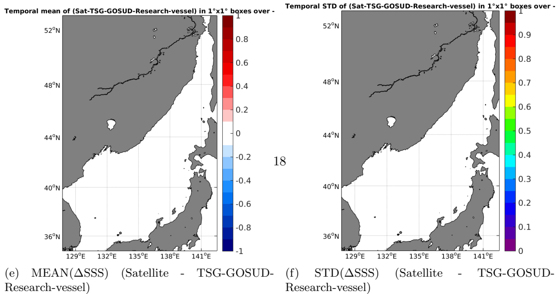
Figure 6: Temporal mean (left) and STD (right) of SSS from SMAP-L2-JPL-V4 (top), TSG-GOSUD-Research-vessel (middle), and of \Delta SSS (Satellite - TSG-GOSUD-Research-vessel). Only
