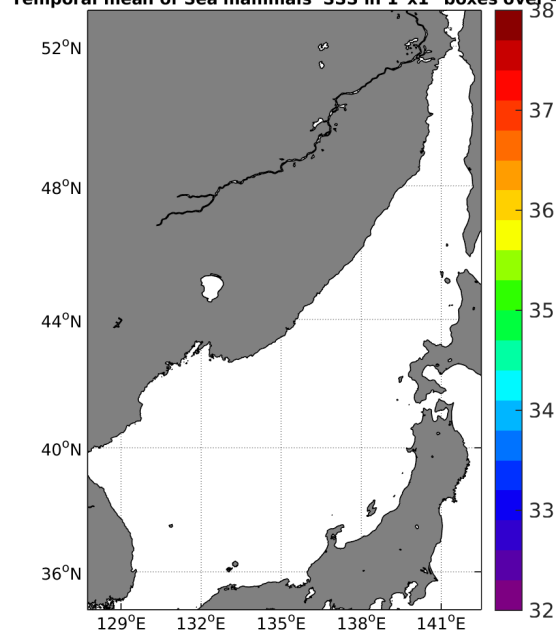
(c) MEAN(Sea mammals SSS)
