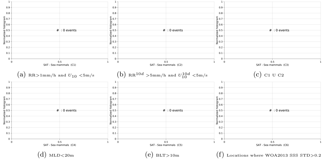
Figure 13: Normalized histogram of \Delta\text{SSS} (SMAP-L2-JPL-V4 - Sea mammals) for 6 different sub-datasets corresponding to: RR > 1\text{mm/h} and U_{10} < 5\text{m/s} (a), RR^{10d} > 5\text{mm/h} and U_{10}^{10d} < 5\text{m/s} (b), C1 U C2 (c), MLD < 20\text{m} (d), BLT > 10\text{m} (e), Locations where WOA2013 SSS STD > 0.2 (f).
