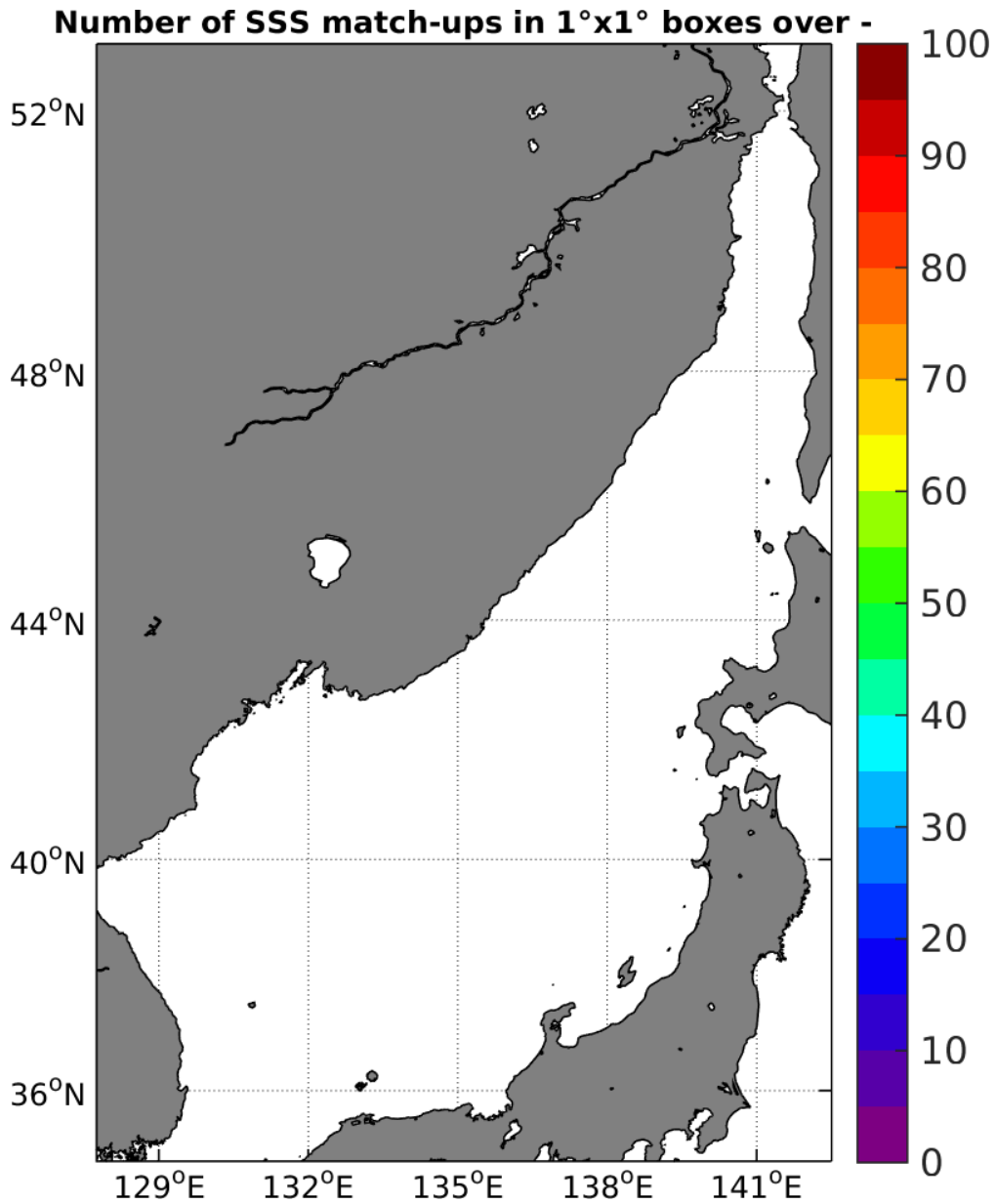
Figure 4: Number of SSS match-ups between Sea mammals SSS and the SMAP-L2-JPL-V4 SSS product for the Sea of Japan Pi-MEP region over 1°x1° boxes and for the full satellite product period.
