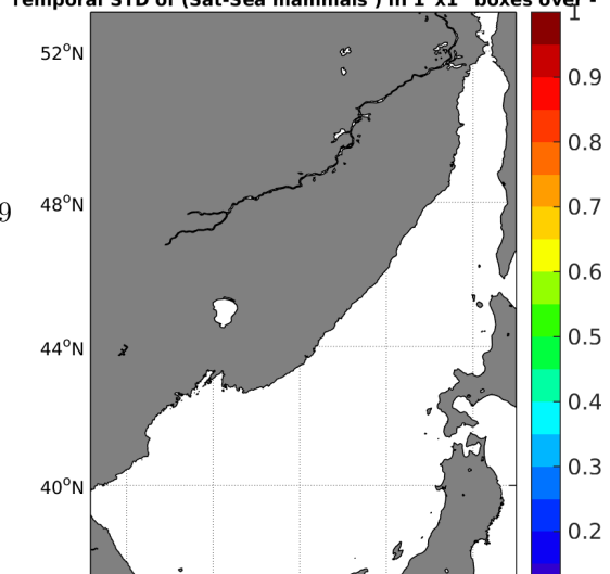
Temporal STD of (Sat-Sea mammals ) in 1°x1° boxes over -
