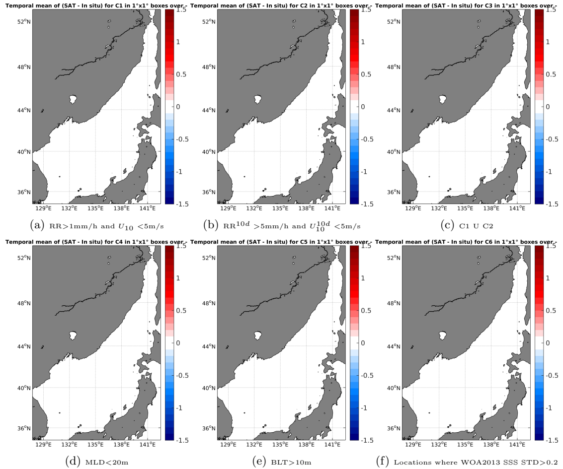
Figure 12: Temporal mean gridded over spatial boxes of size 1^\circ \times 1^\circ of \Delta SSS (SMAP-L2-JPL-V4 - Sea mammals) for 6 different subdatasets corresponding to: RR > 1mm/h and U_{10} < 5\text{m/s} (a), RR^{10d} > 5\text{mm/h} and U_{10}^{10d} < 5\text{m/s} (b), C1 U C2 (c), MLD < 20m (d), BLT > 10m (e), Locations where WOA2013 SSS STD > 0.2 (f).
