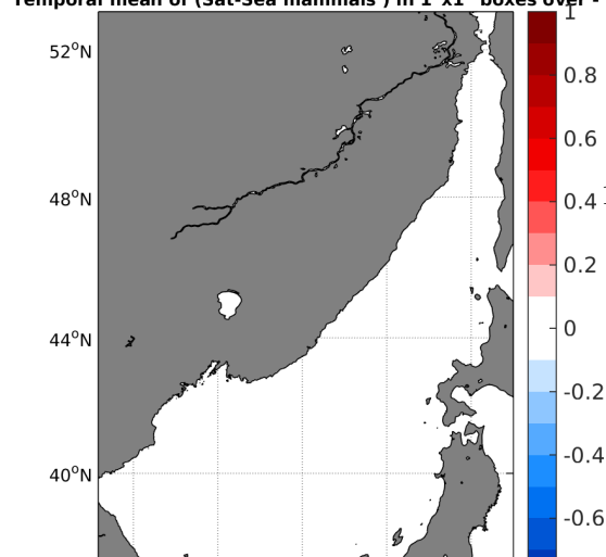
Temporal mean of (Sat-Sea mammals ) in 1°x1° boxes over -
