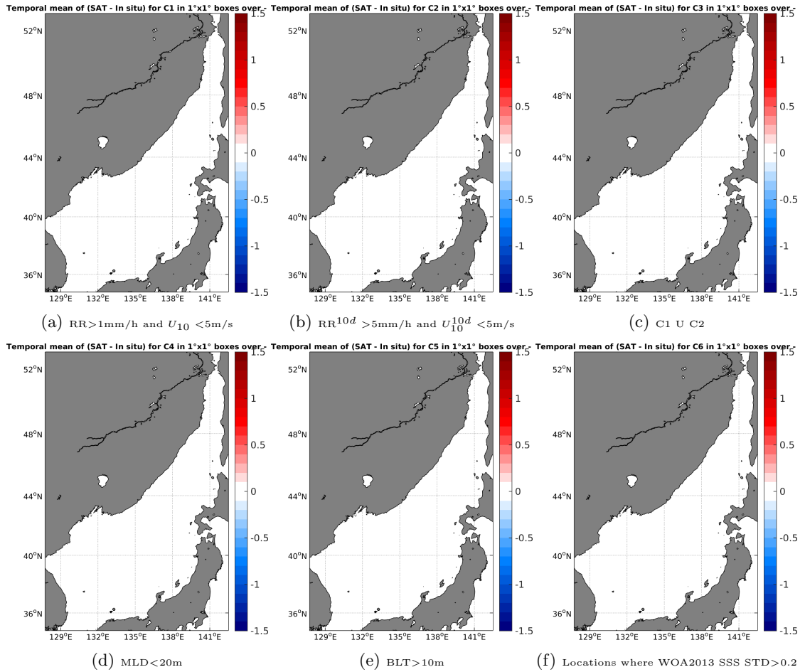
Figure 12: Temporal mean gridded over spatial boxes of size 1^\circ \times 1^\circ of \Delta SSS (SMAP-L2-JPL-V4 - Sea mammals) for 6 different subdatasets corresponding to:RR>1mm/h and U_{10} < 5\text{m/s} (a), RR^{10d} > 5\text{mm/h} and U_{10}^{10d} < 5\text{m/s} (b), C1 U C2 (c),MLD<20m (d),BLT>10m (e),Locations where WOA2013 SSS STD>0.2 (f).
