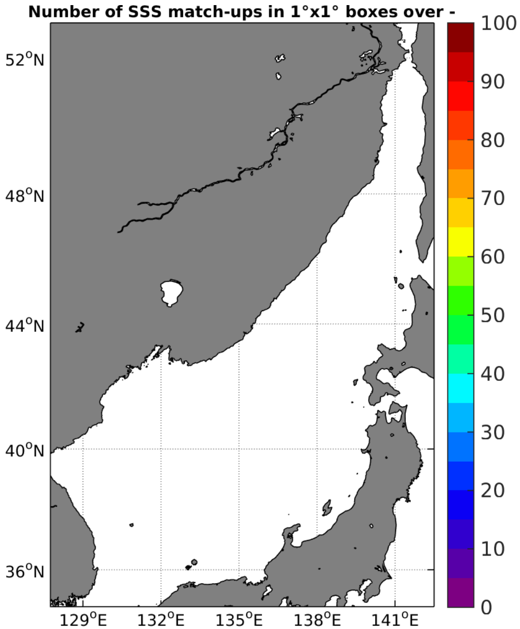
Figure 3: Number of SSS match-ups between Surface drifters SSS and the SMAP-L2-JPL-V4 SSS product for the Sea of Japan Pi-MEP region over 1°x1° boxes and for the full satellite product period.
