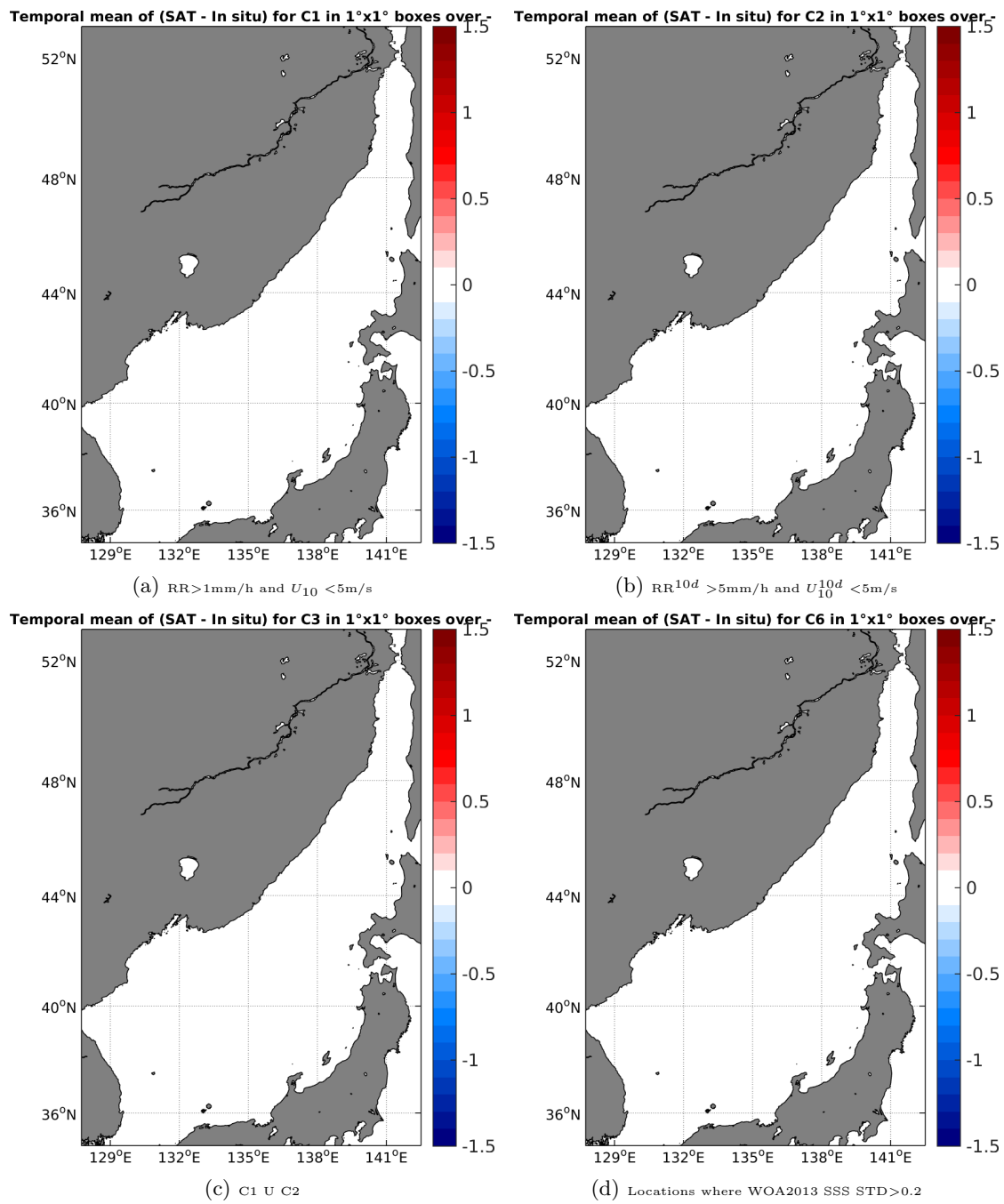
Figure 11: Temporal mean gridded over spatial boxes of size 1°x1° of \Delta\text{SSS} (SMAP-L2-JPL-V4 - Surface drifters) for 4 different subdatasets corresponding to: RR > 1\text{mm/h} and U_{10} < 5\text{m/s} (a), RR^{10d} > 5\text{mm/h} and U_{10}^{10d} < 5\text{m/s} (b), C1 U C2 (c), Locations where WOA2013 SSS STD > 0.2 (d).
