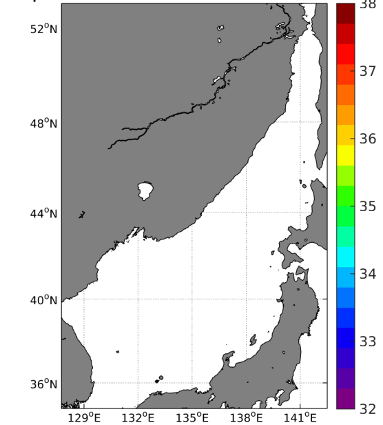
(c) MEAN(Surface drifters SSS)
