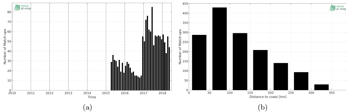
Figure 1: Number of match-ups between Argo and SMAP-L2-JPL-V4 SSS as a function of time (a) and as function of the distance to coast (b) over the Sea of Japan Pi-MEP region and for the full satellite product period.
