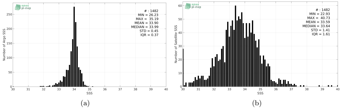
Figure 2: Histograms of SSS from Argo (a) and SMAP-L2-JPL-V4 (b) considering all match-up pairs per bins of 0.1 over the Sea of Japan Pi-MEP region and for the full satellite product period.
