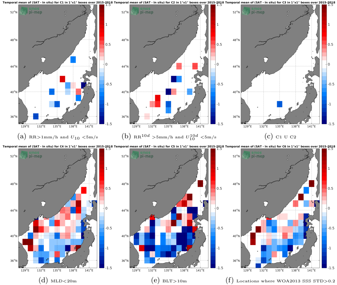
Figure 12: Temporal mean gridded over spatial boxes of size 1°x1° of \Delta SSS (SMAP-L2-JPL-V4 - Argo) for 6 different subdatasets corresponding to:RR>1mm/h and U_{10} < 5m/s (a), RR^{10d} > 5mm/h and U_{10}^{10d} < 5m/s (b), C1 U C2 (c),MLD<20m (d),BLT>10m (e),Locations where WOA2013 SSS STD>0.2 (f).
