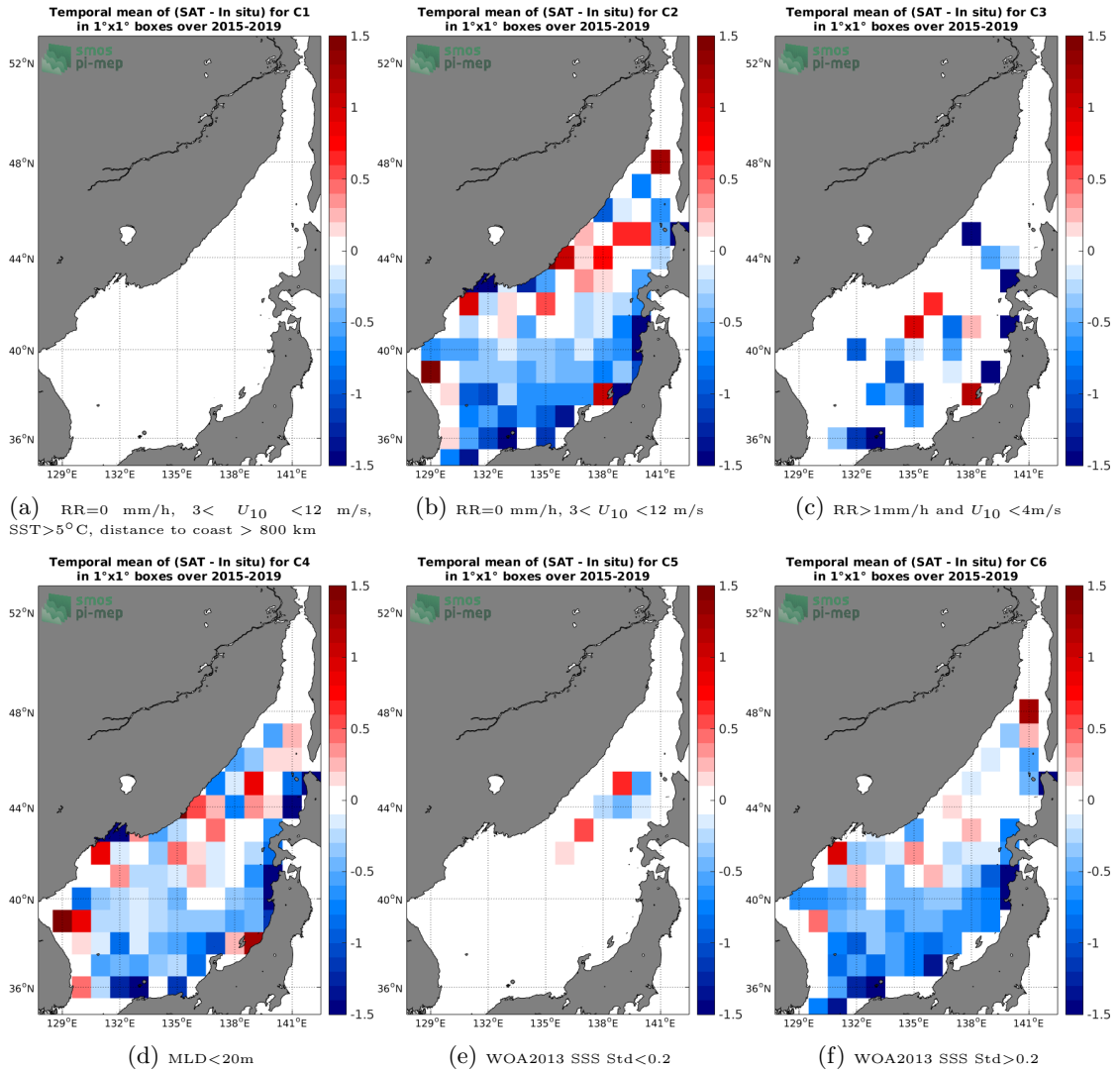
Figure 12: Temporal mean gridded over spatial boxes of size 1°x1° of \Delta SSS (SMAP-L2-JPL-V4.3 - Argo) for 6 different subdatasets corresponding to:RR=0 mm/h, 3 < U_{10} < 12 m/s, SST > 5°C, distance to coast > 800 km (a), RR=0 mm/h, 3 < U_{10} < 12 m/s (b), RR > 1mm/h and U_{10} < 4 m/s (c),MLD < 20m (d),WOA2013 SSS Std < 0.2 (e),WOA2013 SSS Std > 0.2 (f).
