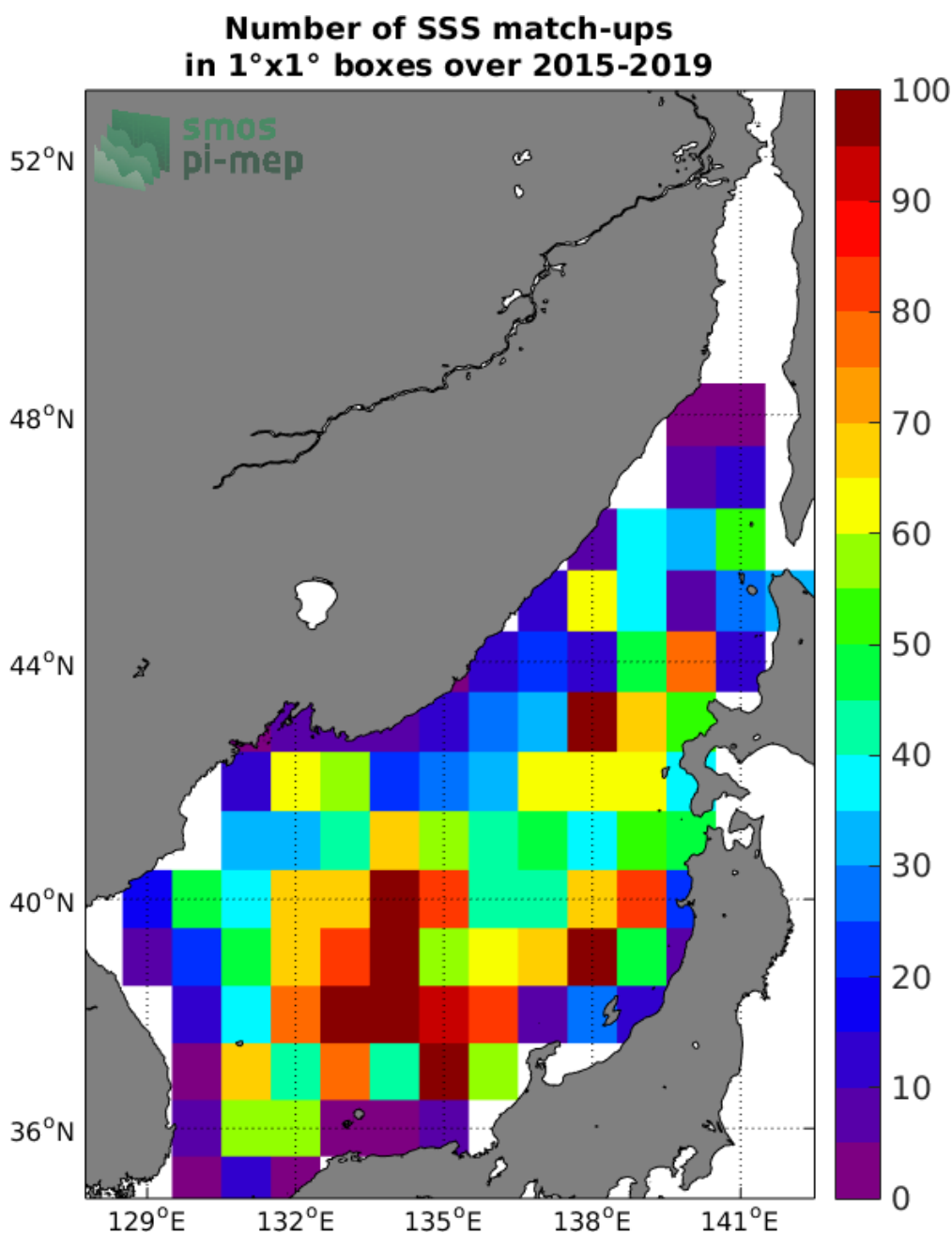
Figure 4: Number of SSS match-ups between Argo SSS and the SMAP-L2-JPL-V4.3 SSS product for the Sea of Japan Pi-MEP region over 1°x1° boxes and for the full satellite product period.
