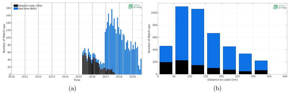
Figure 1: Number of match-ups between Argo and SMAP-L2-JPL-V4.3 SSS as a function of time (a) and as function of the distance to coast (b) over the Sea of Japan Pi-MEP region and for the full satellite product period.
