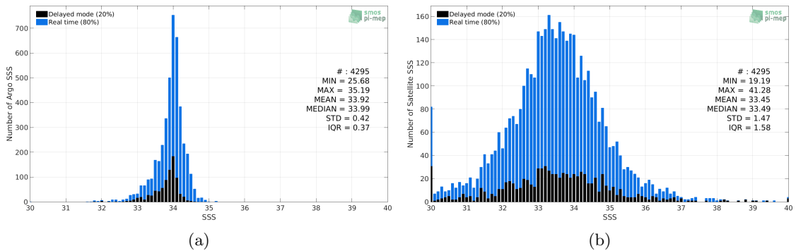
Figure 2: Histograms of SSS from Argo (a) and SMAP-L2-JPL-V4.3 (b) considering all match-up pairs per bins of 0.1 over the Sea of Japan Pi-MEP region and for the full satellite product period.
