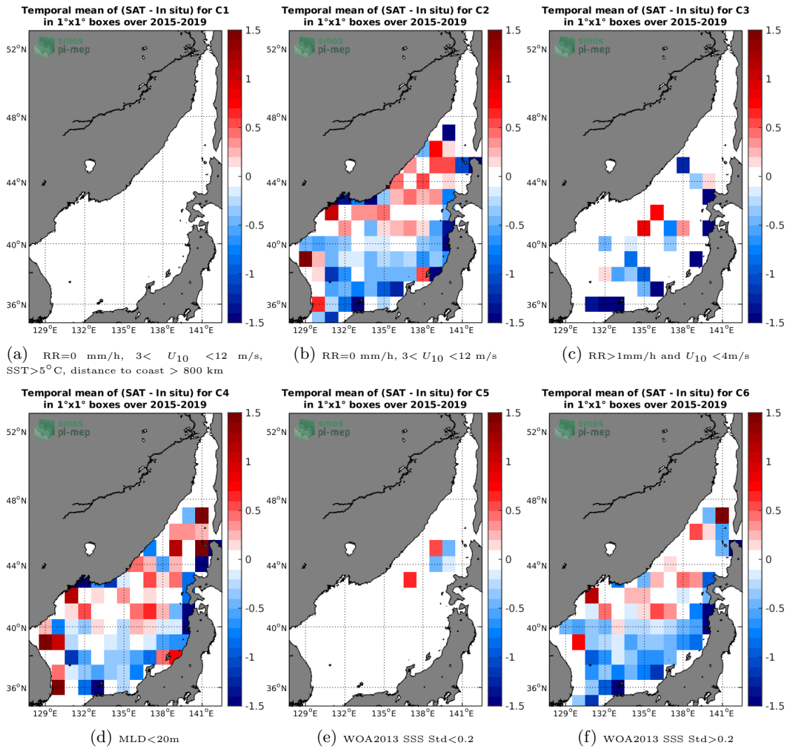
Figure 12: Temporal mean gridded over spatial boxes of size 1^\circ \times 1^\circ of \Delta SSS (SMAP-L2-JPL-V4.2 - Argo) for 6 different subdatasets corresponding to:RR=0 mm/h, 3 < U_{10} < 12 m/s, SST >5^\circ C, distance to coast > 800 km (a), RR=0 mm/h, 3 < U_{10} < 12 m/s (b), RR >1 mm/h and U_{10} < 4 m/s (c),MLD <20 m (d),WOA2013 SSS Std <0.2 (e),WOA2013 SSS Std >0.2 (f).
