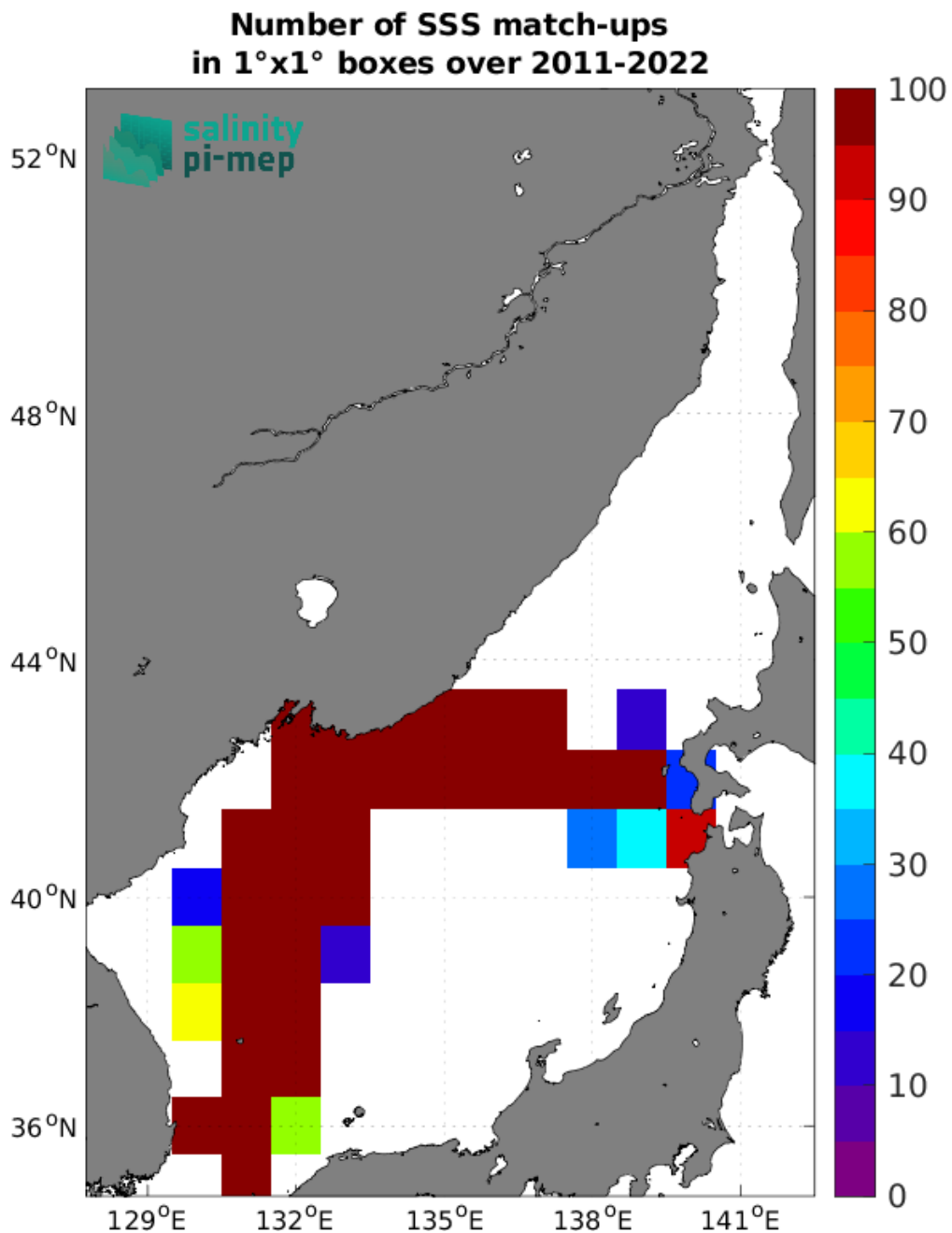
Figure 5: Number of SSS match-ups between TSG (LEGOS-DM) SSS and the CCI SSS L4 Merged-OI v5.5 - 7-day running (ESA) SSS product for the Sea of Japan Pi-MEP region over 1°x1° boxes and for the full satellite product period.
