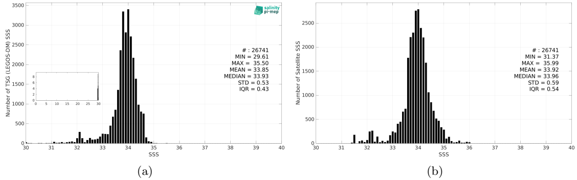
Figure 3: Histograms of SSS from TSG (LEGOS-DM) (a) and CCI SSS L4 Merged-OI v5.5 - 7-day running (ESA) (b) considering all match-up pairs per bins of 0.1 over the Sea of Japan Pi-MEP region and for the full satellite product period.
