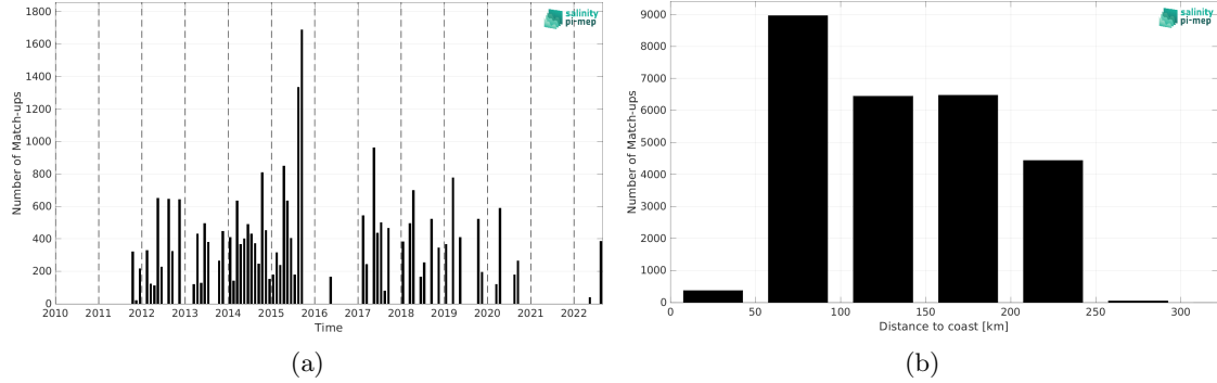
Figure 2: Number of match-ups between TSG (LEGOS-DM) and CCI SSS L4 Merged-OI v5.5 - 7-day running (ESA) SSS as a function of time (a) and as function of the distance to coast (b) over the Sea of Japan Pi-MEP region and for the full satellite product period.
