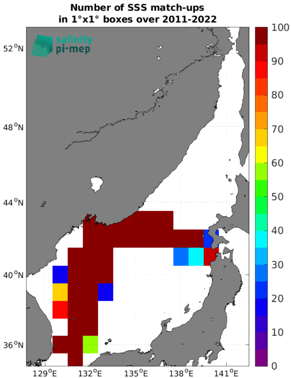
Figure 5: Number of SSS match-ups between TSG (LEGOS-DM) SSS and the CCI SSS L4 Merged-OI v5.5 - 30-day running (ESA) SSS product for the Sea of Japan Pi-MEP region over 1°x1° boxes and for the full satellite product period.
