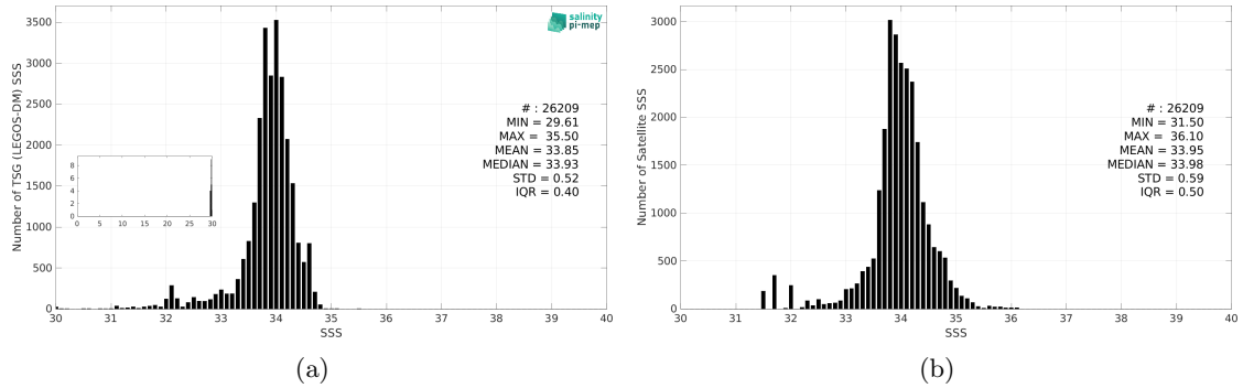
Figure 3: Histograms of SSS from TSG (LEGOS-DM) (a) and CCI SSS L4 Merged-OI v5.5 - 30-day running (ESA) (b) considering all match-up pairs per bins of 0.1 over the Sea of Japan Pi-MEP region and for the full satellite product period.
