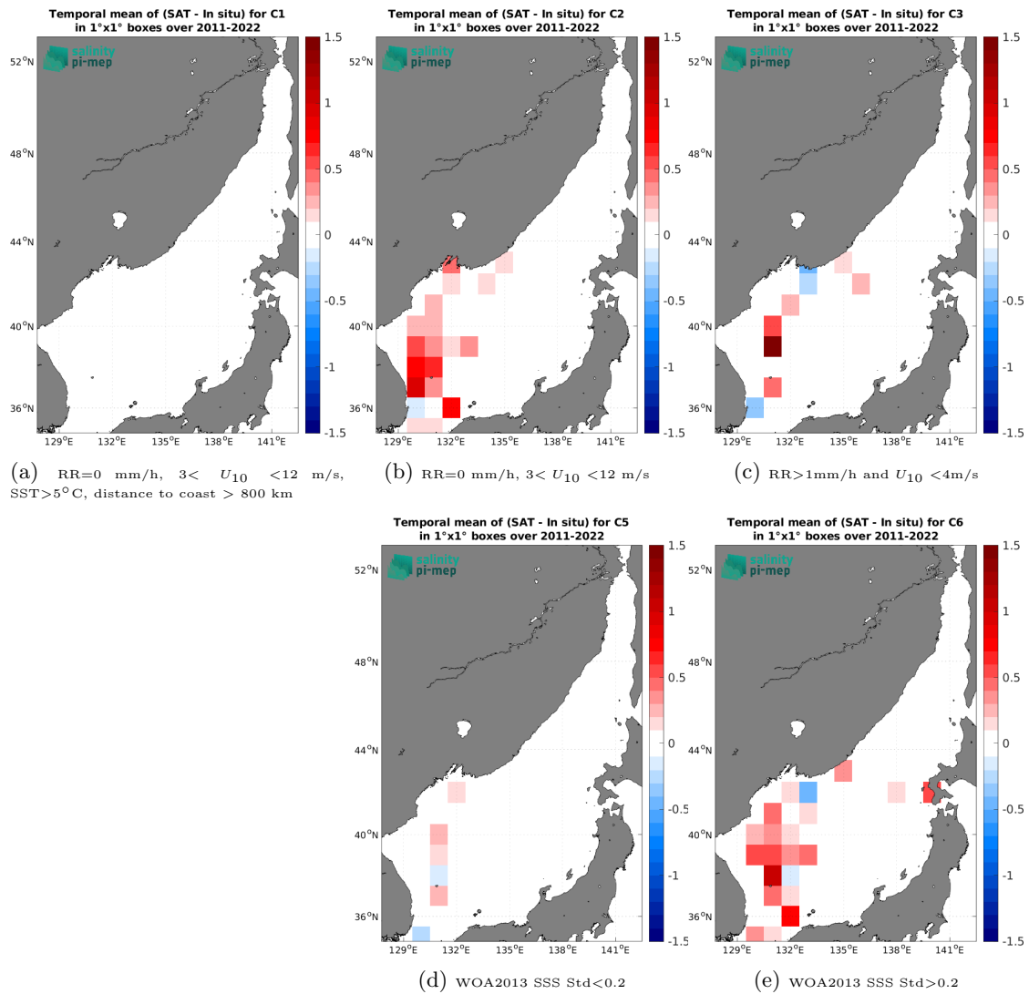
Figure 14: Temporal mean gridded over spatial boxes of size 1^\circ \times 1^\circ of \Delta SSS (CCI SSS L4 Merged-OI v5.5 - 30-day running (ESA) - TSG (LEGOS-DM)) for 5 different subdatasets corresponding to:RR=0 mm/h, 3 < U_{10} < 12 m/s, SST>5°C, distance to coast > 800 km (a), RR=0 mm/h, 3 < U_{10} < 12 m/s (b), RR>1mm/h and U_{10} < 4 m/s (c), WOA2013 SSS Std<0.2 (d), WOA2013 SSS Std>0.2 (e).
