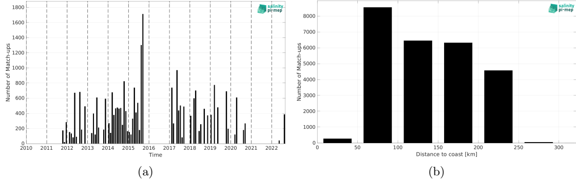
Figure 2: Number of match-ups between TSG (LEGOS-DM) and CCI SSS L4 Merged-OI v5.5 - 30-day running (ESA) SSS as a function of time (a) and as function of the distance to coast (b) over the Sea of Japan Pi-MEP region and for the full satellite product period.
