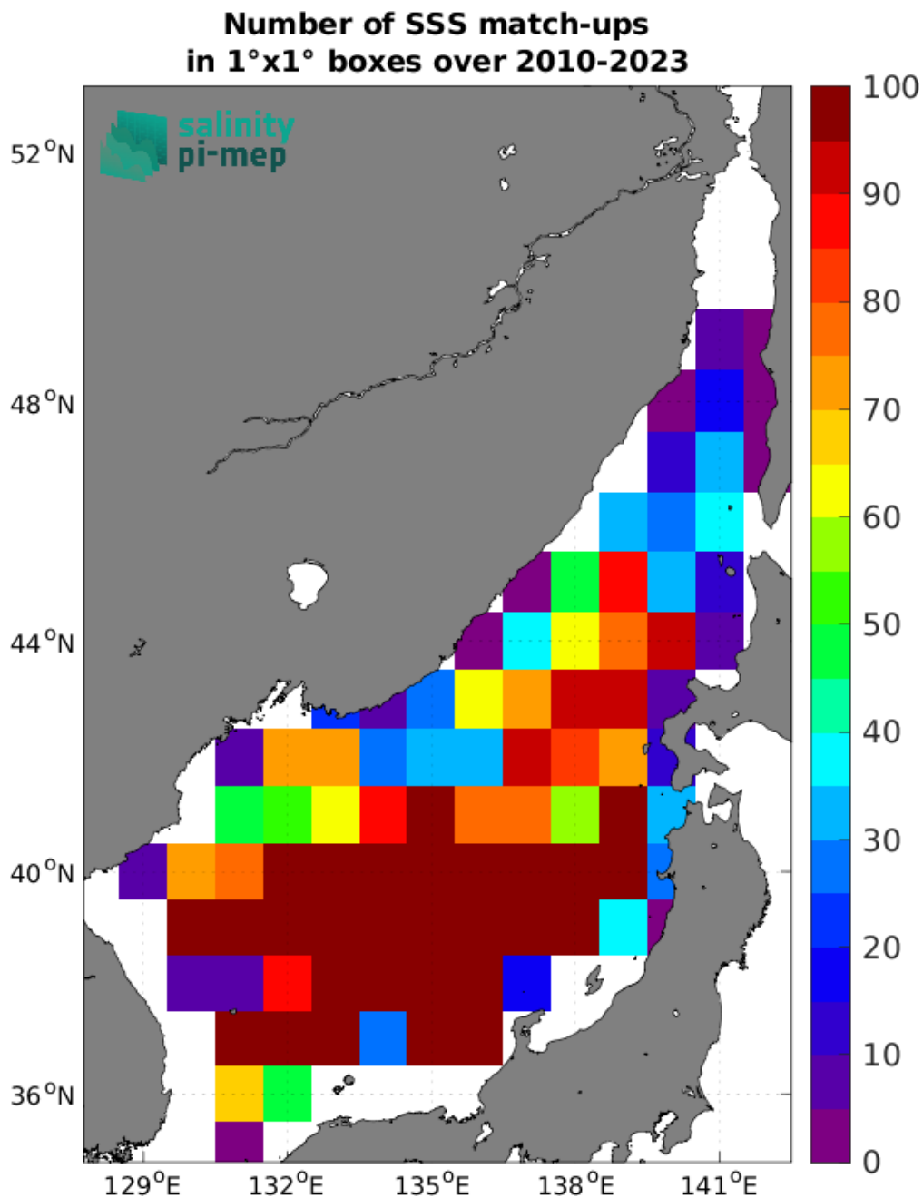
Figure 5: Number of SSS match-ups between Argo SSS and the CCI SSS L4 Merged-OI v5.5 - 30-day running (ESA) SSS product for the Sea of Japan Pi-MEP region over 1^\circ \times 1^\circ boxes and for the full satellite product period.
