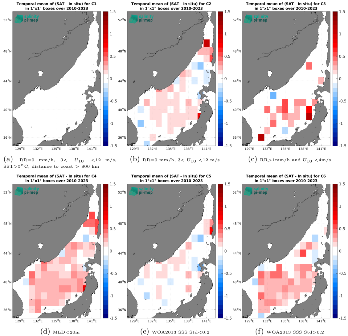
Figure 14: Temporal mean gridded over spatial boxes of size 1^\circ \times 1^\circ of \Delta\text{SSS} (CCI SSS L4 Merged-OI v5.5 - 30-day running (ESA) - Argo) for 6 different subdatasets corresponding to: RR=0 mm/h, 3 < U_{10} < 12 m/s, SST > 5^\circ\text{C} , distance to coast > 800 km (a), RR=0 mm/h, 3 < U_{10} < 12 m/s (b), RR > 1 mm/h and U_{10} < 4 m/s (c), MLD < 20 m (d), WOA2013 SSS Std < 0.2 (e), WOA2013 SSS Std > 0.2 (f).
