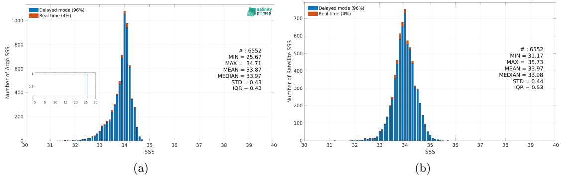
Figure 3: Histograms of SSS from Argo (a) and CCI SSS L4 Merged-OI v5.5 - 30-day running (ESA) (b) considering all match-up pairs per bins of 0.1 over the Sea of Japan Pi-MEP region and for the full satellite product period.
