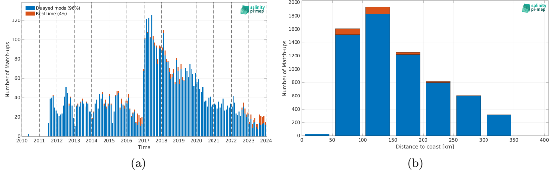
Figure 2: Number of match-ups between Argo and CCI SSS L4 Merged-OI v5.5 - 30-day running (ESA) SSS as a function of time (a) and as function of the distance to coast (b) over the Sea of Japan Pi-MEP region and for the full satellite product period.
