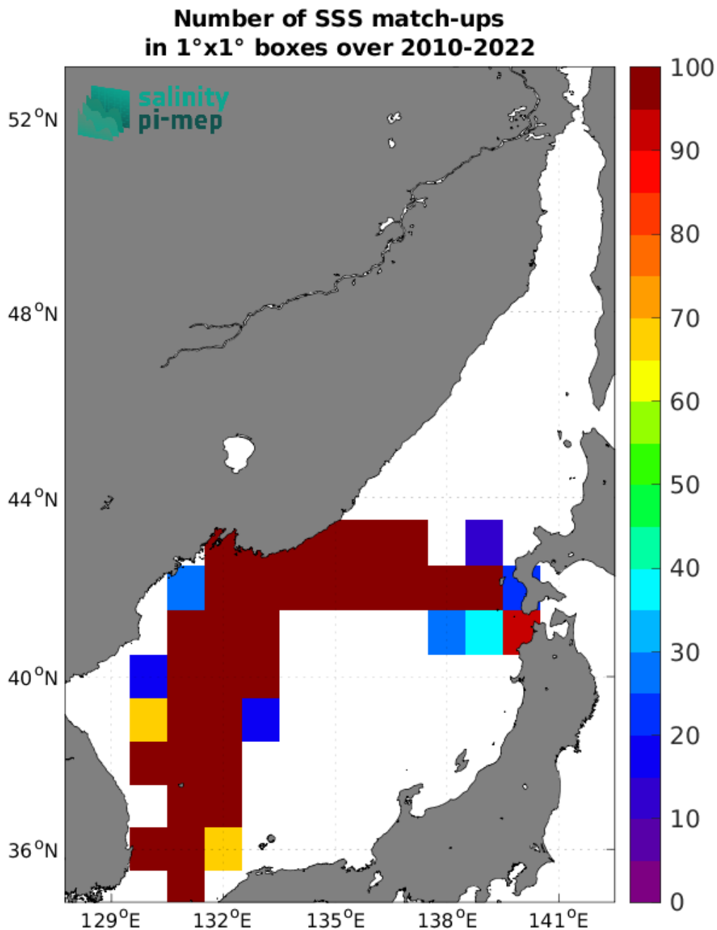
Figure 5: Number of SSS match-ups between TSG (LEGOS-DM) SSS and the CCI SSS L4 Merged-OI v4.41 - 7-day running (ESA) SSS product for the Sea of Japan Pi-MEP region over 1°x1° boxes and for the full satellite product period.
