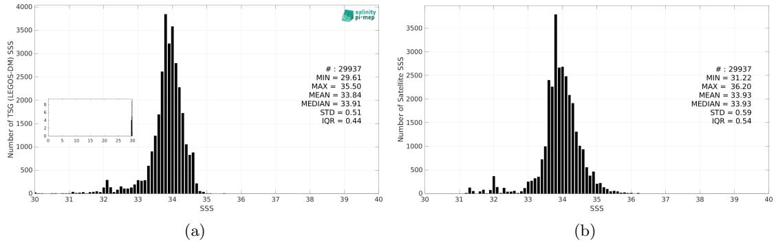
Figure 3: Histograms of SSS from TSG (LEGOS-DM) (a) and CCI SSS L4 Merged-OI v4.41 - 7-day running (ESA) (b) considering all match-up pairs per bins of 0.1 over the Sea of Japan Pi-MEP region and for the full satellite product period.
