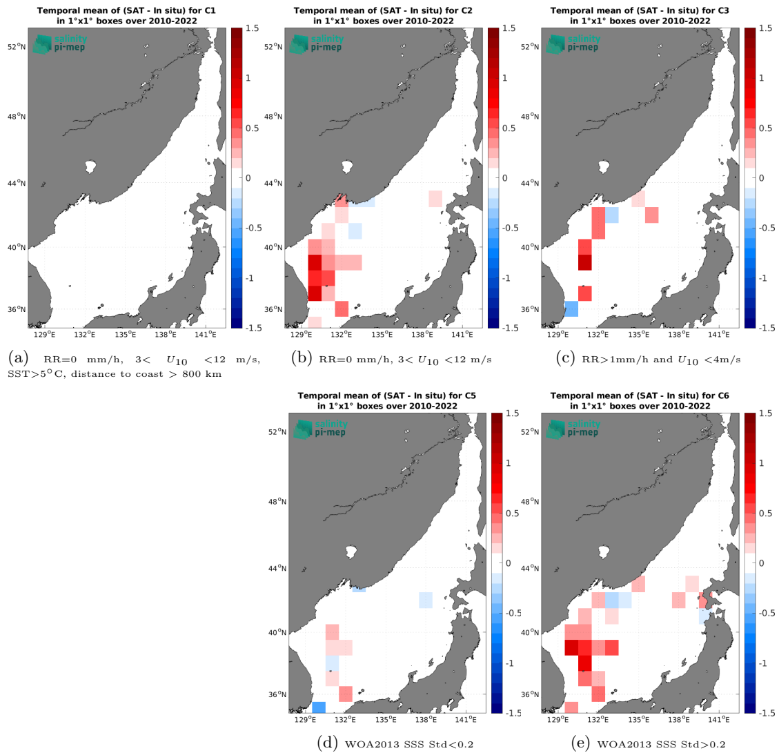
Figure 14: Temporal mean gridded over spatial boxes of size 1^\circ \times 1^\circ of \Delta SSS (CCI SSS L4 Merged-OI v4.41 - 7-day running (ESA) - TSG (LEGOS-DM)) for 5 different subdatasets corresponding to: RR=0 mm/h, 3 < U_{10} < 12 m/s, SST>5°C, distance to coast > 800 km (a), RR=0 mm/h, 3 < U_{10} < 12 m/s (b), RR>1mm/h and U_{10} < 4 m/s (c), WOA2013 SSS Std<0.2 (d), WOA2013 SSS Std>0.2 (e).
