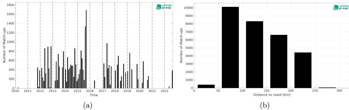
Figure 2: Number of match-ups between TSG (LEGOS-DM) and CCI SSS L4 Merged-OI v4.41 - 7-day running (ESA) SSS as a function of time (a) and as function of the distance to coast (b) over the Sea of Japan Pi-MEP region and for the full satellite product period.
