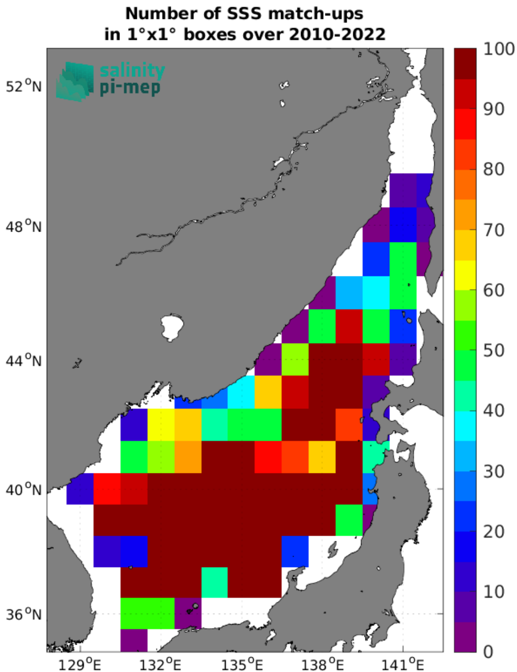
Figure 5: Number of SSS match-ups between Argo SSS and the CCI SSS L4 Merged-OI v4.41 - 7-day running (ESA) SSS product for the Sea of Japan Pi-MEP region over 1°×1° boxes and for the full satellite product period.
