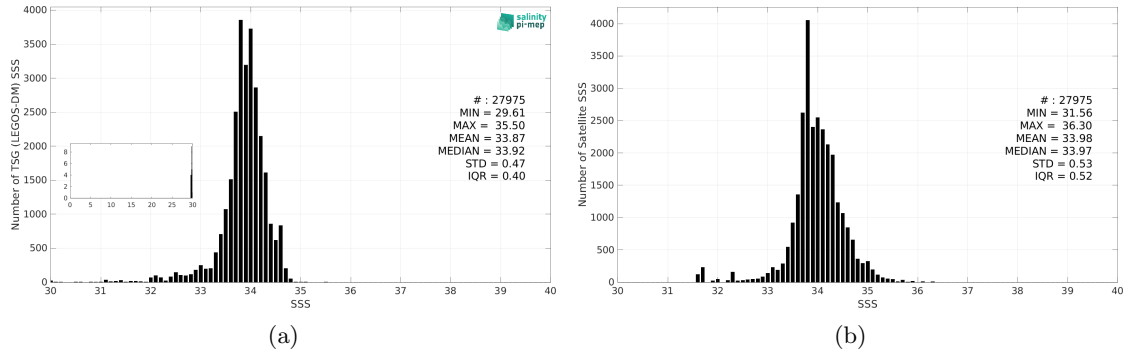
Figure 3: Histograms of SSS from TSG (LEGOS-DM) (a) and CCI SSS L4 Merged-OI v4.41 - 30-day running (ESA) (b) considering all match-up pairs per bins of 0.1 over the Sea of Japan Pi-MEP region and for the full satellite product period.
