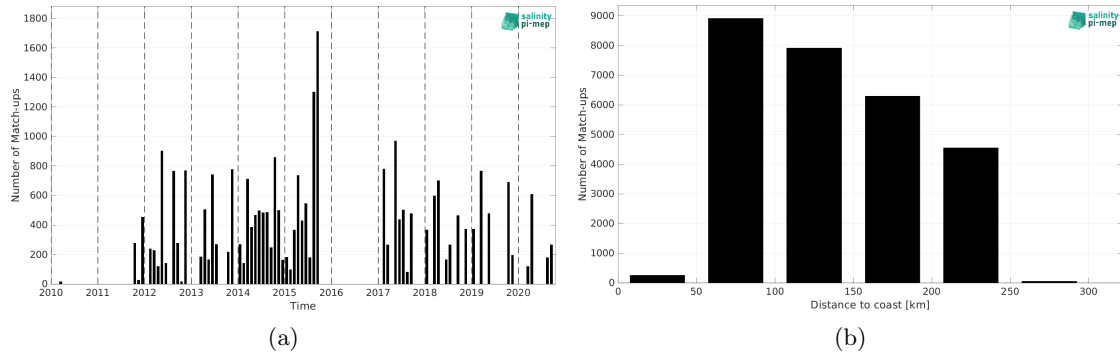
Figure 2: Number of match-ups between TSG (LEGOS-DM) and CCI SSS L4 Merged-OI v4.41 - 30-day running (ESA) SSS as a function of time (a) and as function of the distance to coast (b) over the Sea of Japan Pi-MEP region and for the full satellite product period.
