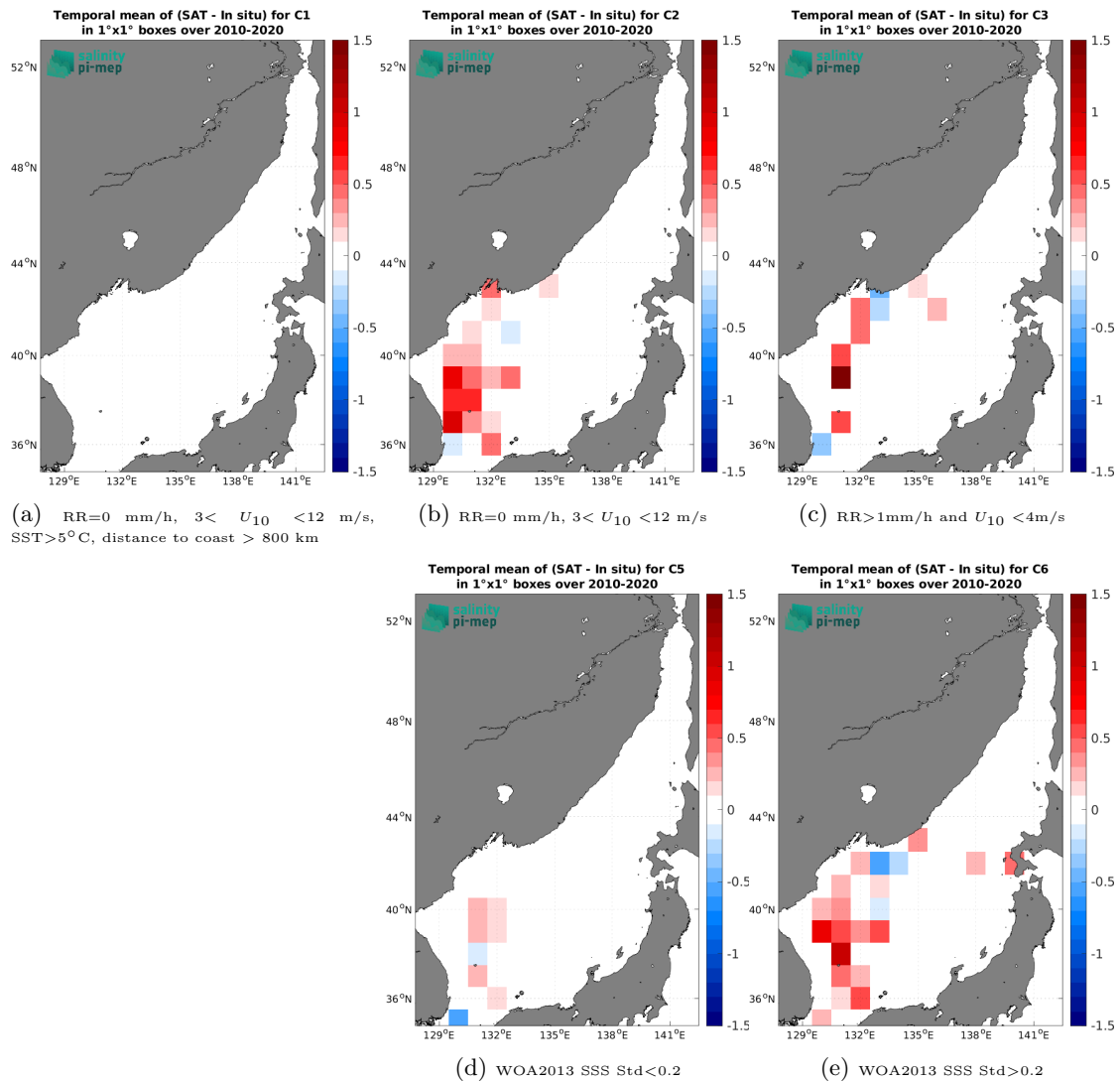
Figure 14: Temporal mean gridded over spatial boxes of size 1^\circ \times 1^\circ of \Delta\text{SSS} (CCI SSS L4 Merged-OI v4.41 - 30-day running (ESA) - TSG (LEGOS-DM)) for 5 different subdatasets corresponding to: RR=0 mm/h, 3 < U_{10} < 12 m/s, SST > 5^\circ\text{C} , distance to coast > 800 km (a), RR=0 mm/h, 3 < U_{10} < 12 m/s (b), RR > 1\text{mm/h} and U_{10} < 4\text{m/s} (c), WOA2013 SSS Std < 0.2 (d), WOA2013 SSS Std > 0.2 (e).
