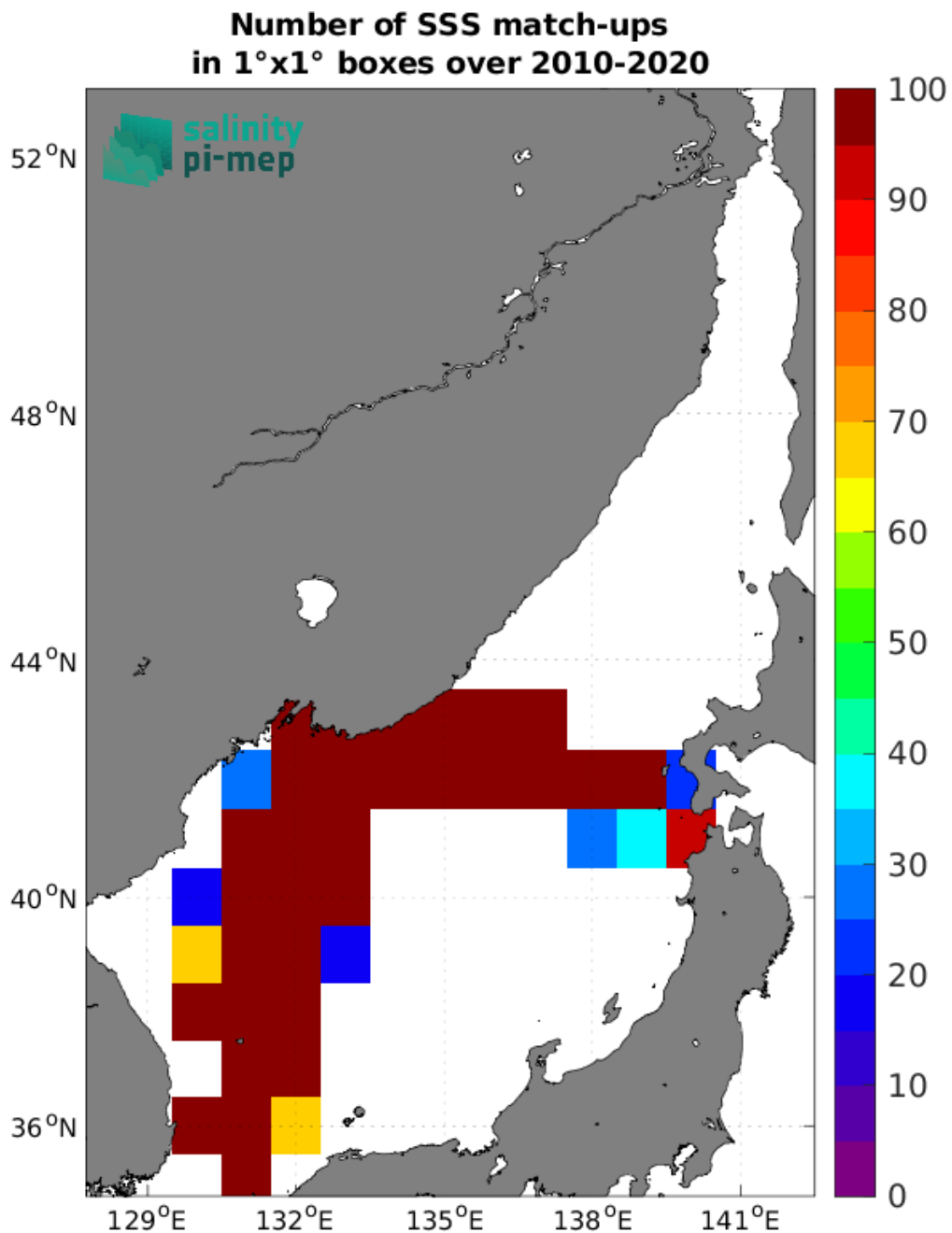
Figure 5: Number of SSS match-ups between TSG (LEGOS-DM) SSS and the CCI SSS L4 Merged-OI v4.41 - 30-day running (ESA) SSS product for the Sea of Japan Pi-MEP region over 1°x1° boxes and for the full satellite product period.
