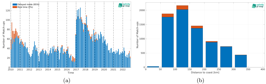
Figure 2: Number of match-ups between Argo and CCI SSS L4 Merged-OI v4.41 - 30-day running (ESA) SSS as a function of time (a) and as function of the distance to coast (b) over the Sea of Japan Pi-MEP region and for the full satellite product period.
