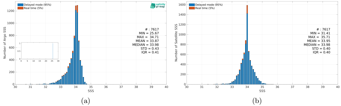
Figure 3: Histograms of SSS from Argo (a) and CCI SSS L4 Merged-OI v4.41 - 30-day running (ESA) (b) considering all match-up pairs per bins of 0.1 over the Sea of Japan Pi-MEP region and for the full satellite product period.
